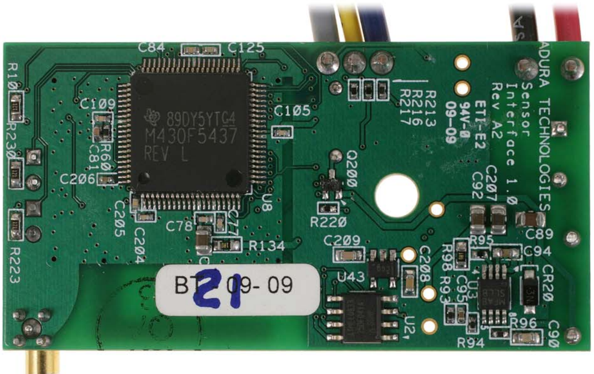
Sensor Interface board - back
