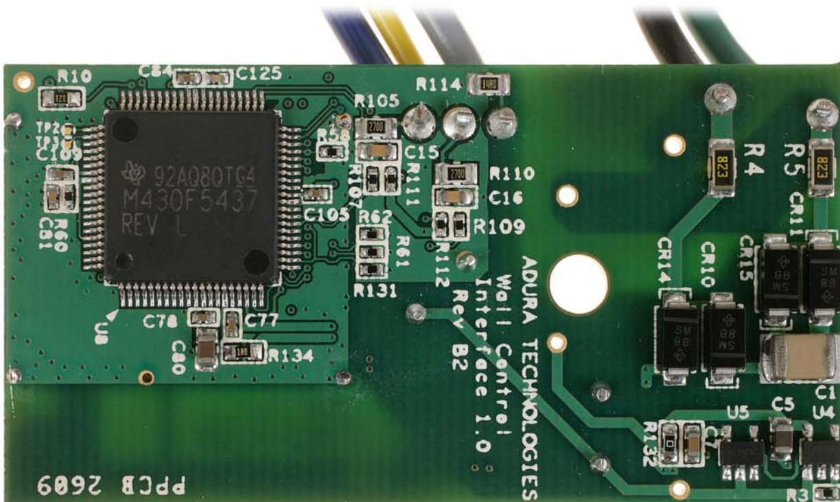
Wall Control Interface Board back
