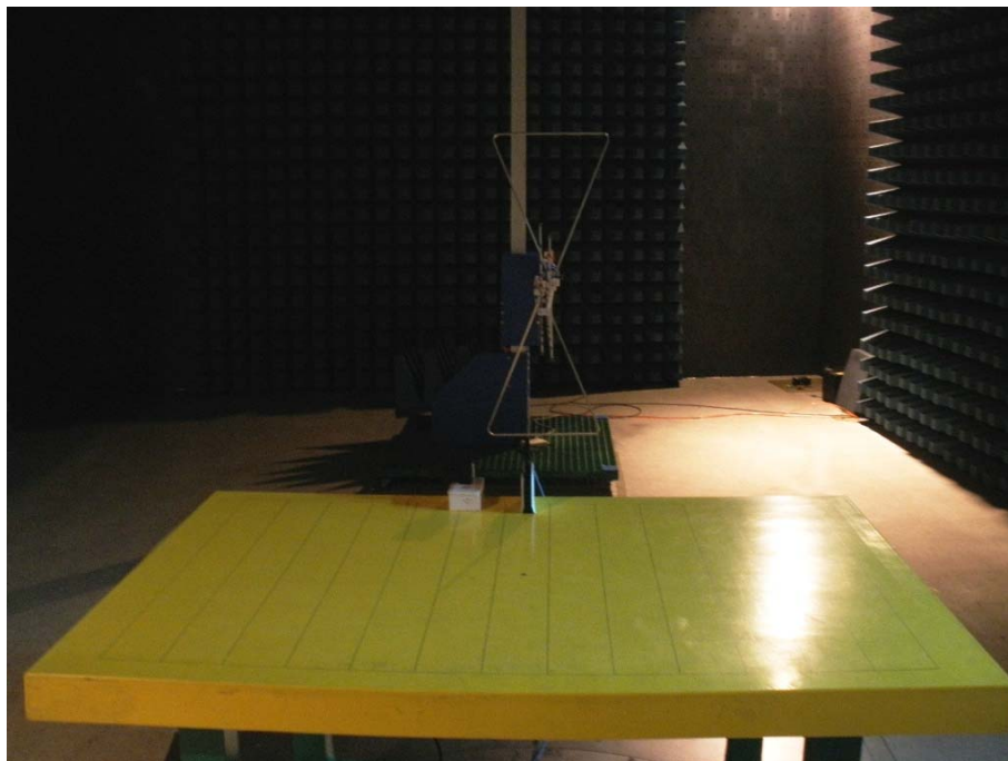
Radiated Emission Test set-up photo
