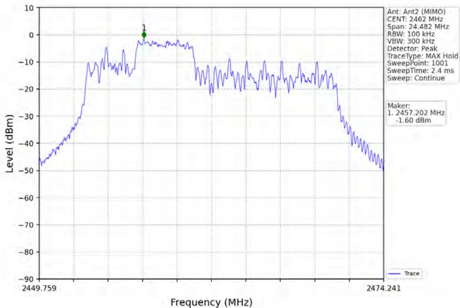
802.11ax(HEW20)_HCH_2462MHz_RU52_Mid_Ant2 (MIMO)_NTNV
