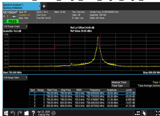
N14(5M)_DFT-s- OFDM_BPSK_Edge_1RB_Right_High_CH
