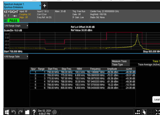
N14(10M)_DFT-s- OFDM_QPSK_Edge_1RB_Right_Mid_CH
