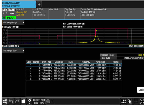
N14(10M)_DFT-s- OFDM_BPSK_Edge_1RB_Left_Mid_CH
