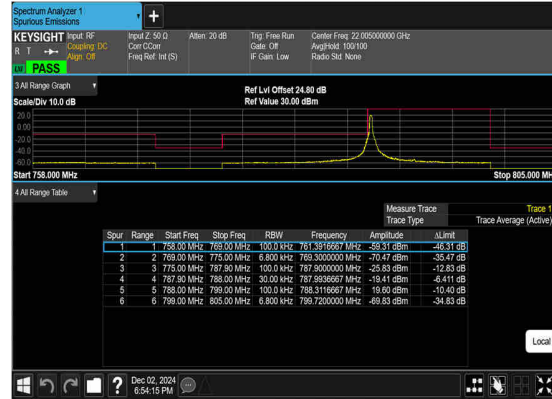
N14(5M)_DFT-s- OFDM_QPSK_Edge_1RB_Left_Low_CH
