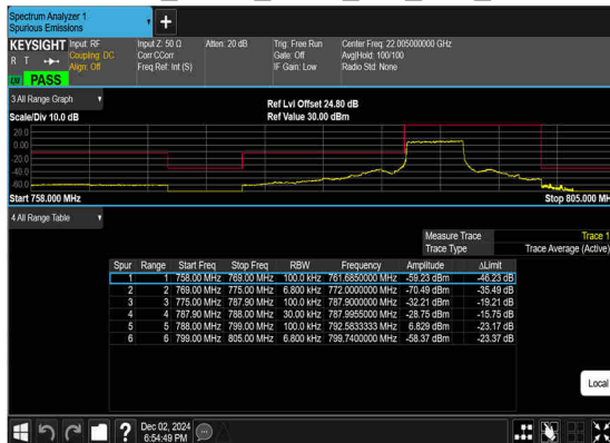
N14(5M)_DFT-s- OFDM_BPSK_Outer_Full_Low_CH
