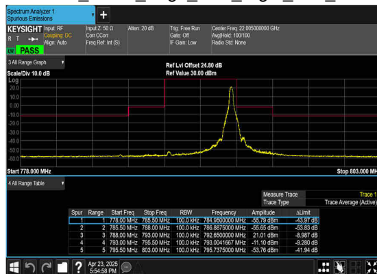
N14(5M)_DFT-s- OFDM_BPSK_Edge_1RB_Right_Low_CH
