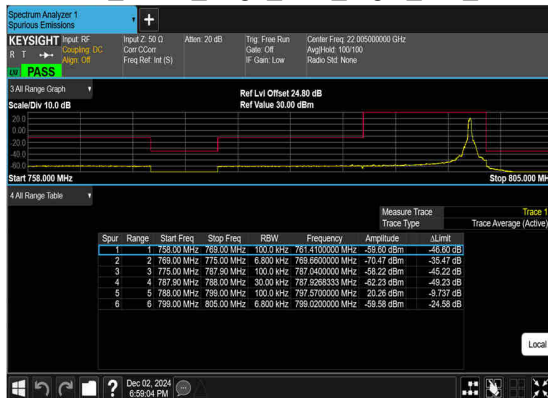
N14(10M)_DFT-s- OFDM_BPSK_Edge_1RB_Right_Mid_CH
