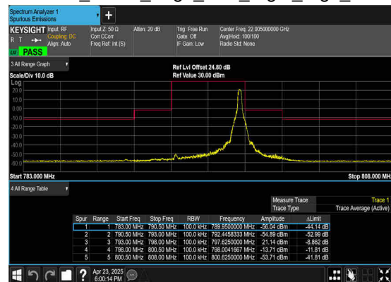
N14(5M)_DFT-s- OFDM_QPSK_Edge_1RB_Right_High_CH
