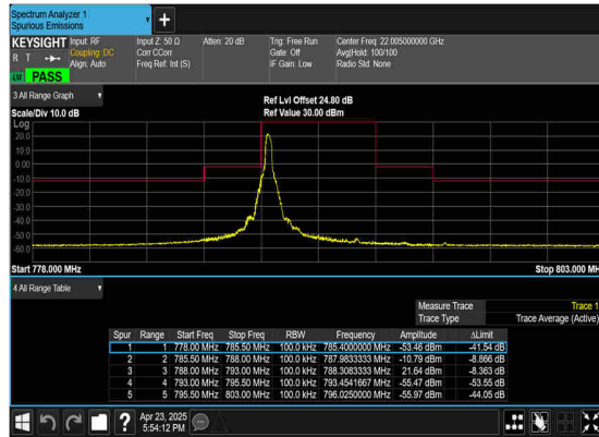
N14(5M)_DFT-s- OFDM_BPSK_Edge_1RB_Left_Low_CH
