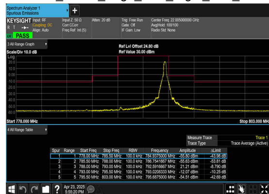
N14(5M)_DFT-s- OFDM_QPSK_Edge_1RB_Right_Low_CH
