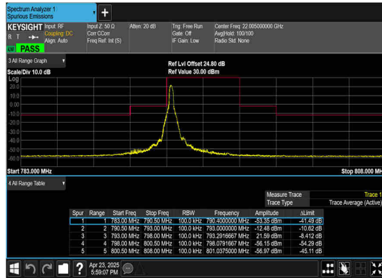
N14(5M)_DFT-s- OFDM_BPSK_Edge_1RB_Left_High_CH
