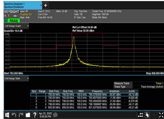
N14(5M)_DFT-s- OFDM_QPSK_Edge_1RB_Left_High_CH
