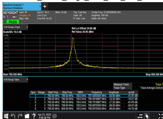
N14(5M)_DFT-s- OFDM_BPSK_Edge_1RB_Left_Mid_CH
