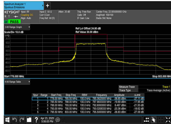
N14(5M)_DFT-s- OFDM_QPSK_Outer_Full_Low_CH
