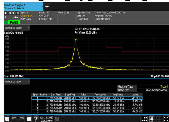
N14(5M)_DFT-s- OFDM_QPSK_Edge_1RB_Left_Mid_CH
