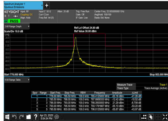
N14(5M)_DFT-s- OFDM_QPSK_Edge_1RB_Left_Low_CH
