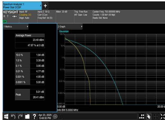
N14(5M)_DFT-s-OFDM_PI_2- BPSK_Outer_Full_Mid_CH
