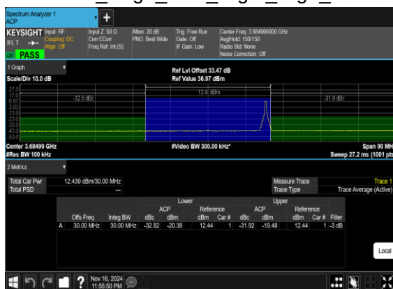
N48(30M)_DFT-s-OFDM_PI_2-BPSK_Edge_1RB_Right_High_CH
