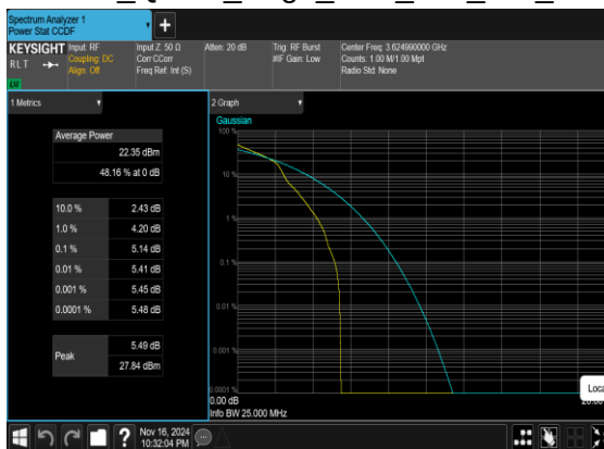
N48(20M)_DFT-s-OFDM_QPSK_Edge_1RB_Left_Mid_CH
