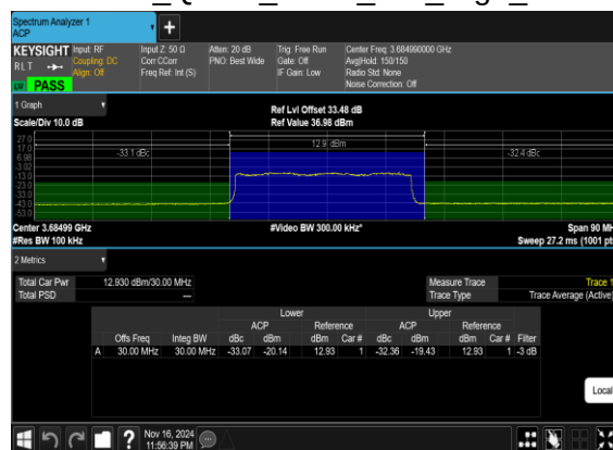
N48(30M)_DFT-s-OFDM_QPSK_Outer_Full_High_CH
