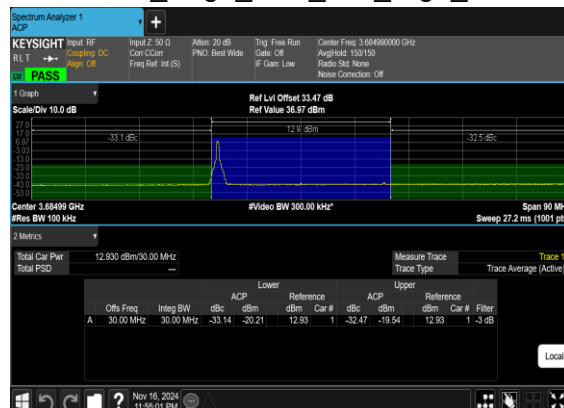
N48(30M)_DFT-s-OFDM_PI_2-BPSK_Edge_1RB_Left_High_CH
