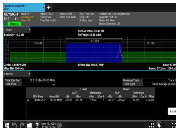
N48(30M)_DFT-s-OFDM_QPSK_Edge_1RB_Right_High_CH
