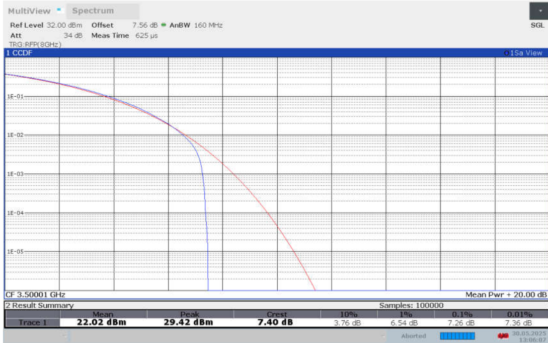
Band n78L , 20MHz Bandwidth,CP-256QAM
