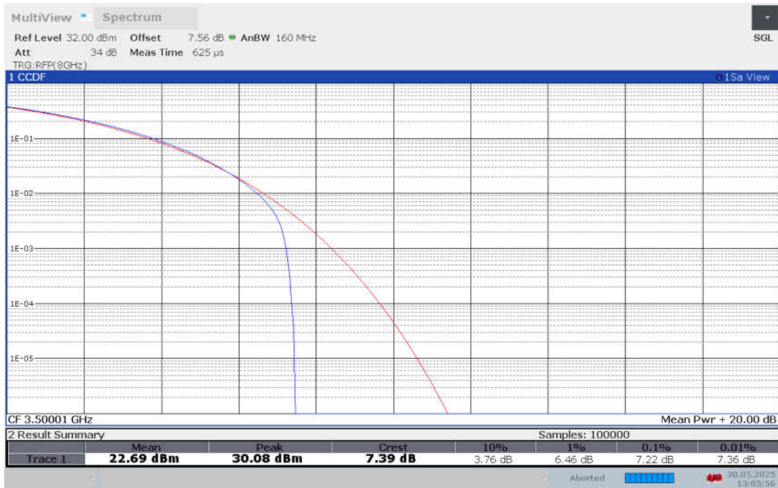
Band n78L , 20MHz Bandwidth,CP-64QAM
