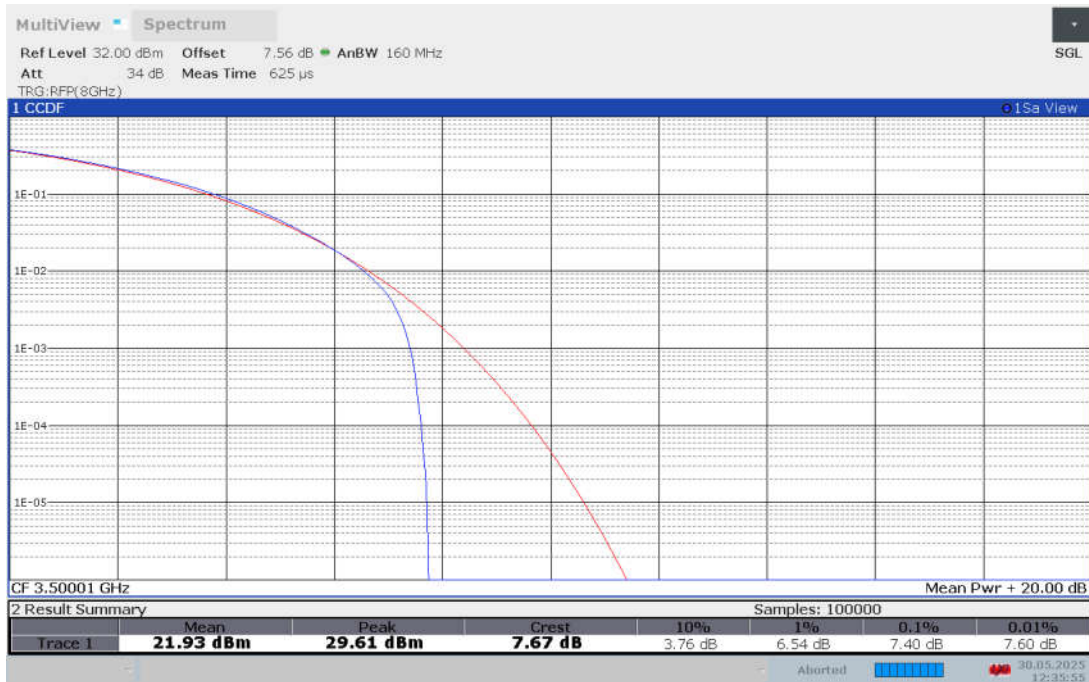
Band n77L , 90MHz Bandwidth,CP-256QAM
