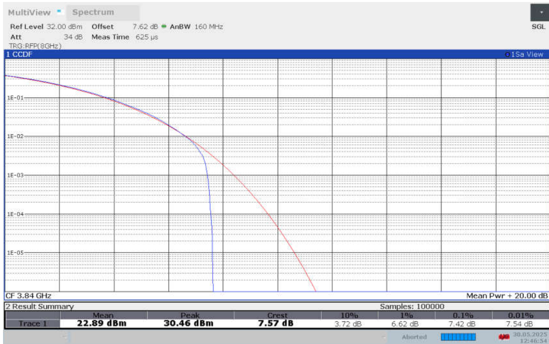
Band n77H , 40MHz Bandwidth,CP-256QAM
