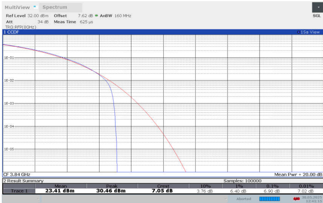
Band n77H , 20MHz Bandwidth,CP-64QAM
