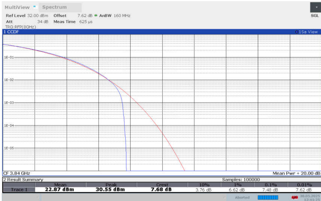
Band n77H , 20MHz Bandwidth,CP-256QAM
