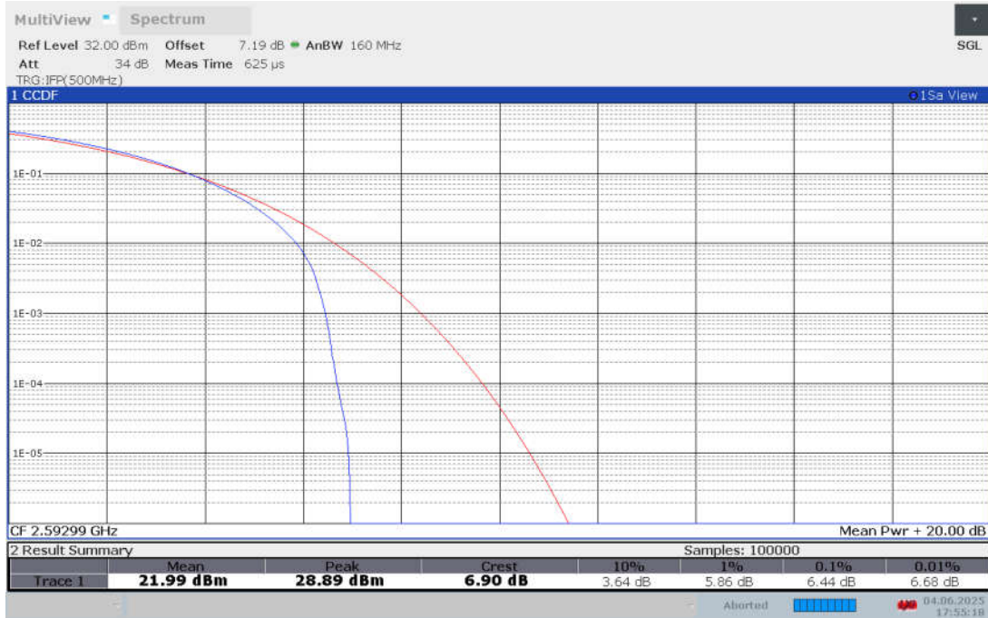
Band n41 , 90MHz Bandwidth,CP-16QAM
