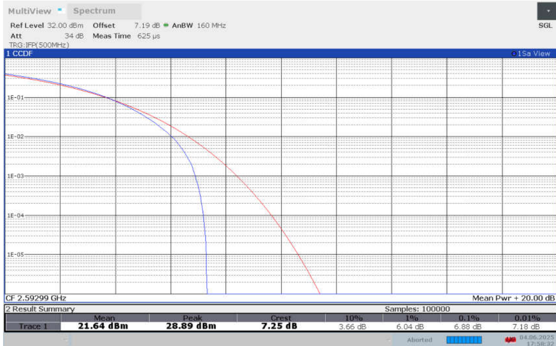
Band n41 , 100MHz Bandwidth,CP-256QAM
