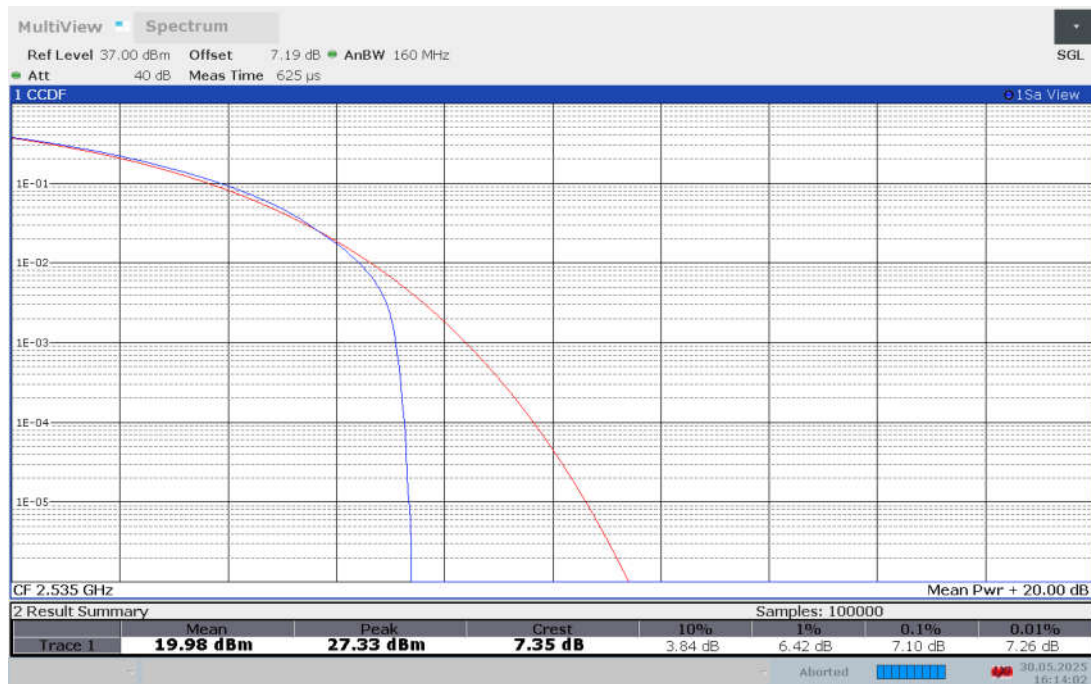
Band n7 , 10MHz Bandwidth,CP-64QAM
