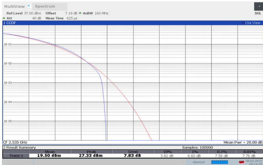
Band n7 , 10MHz Bandwidth,CP-256QAM
