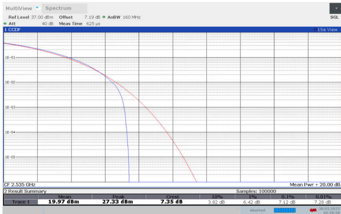
Band n7 , 20MHz Bandwidth,CP-64QAM
