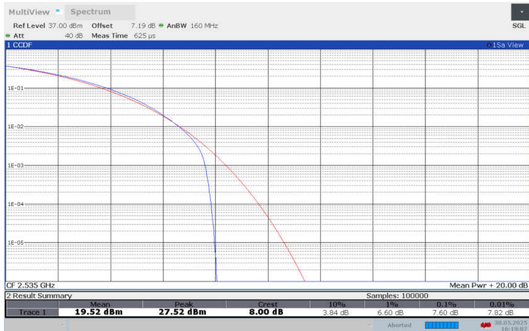
Band n7 , 20MHz Bandwidth,CP-256QAM
