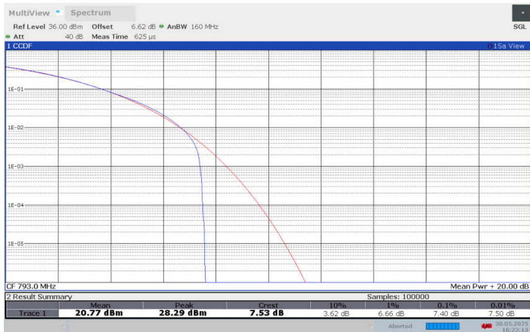
Band n14 , 5MHz Bandwidth,CP-16QAM
