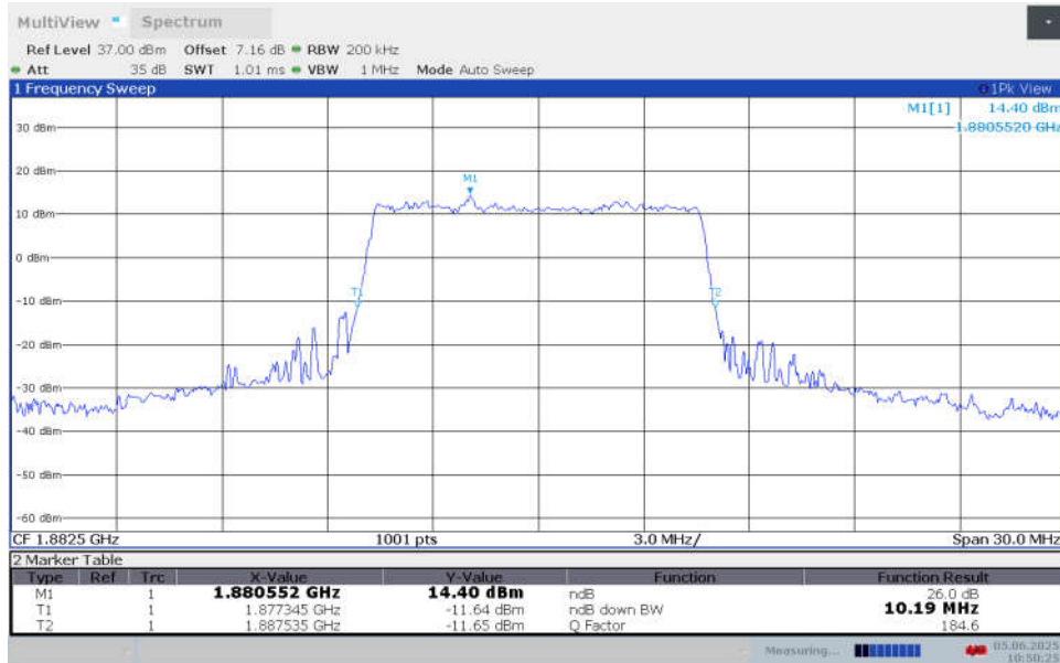
n25,10MHz Bandwidth,CP-16QAM (-26dBc BW)
