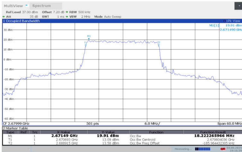
n41,20MHz Bandwidth,DFT-s-16QAM (99% BW)
