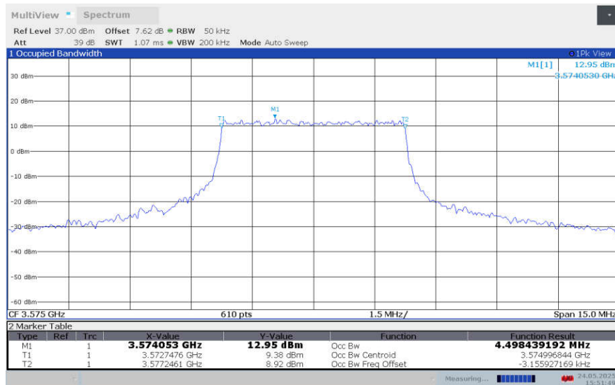
LTE band 42 , 5MHz Bandwidth,MID,16QAM (99% BW)
