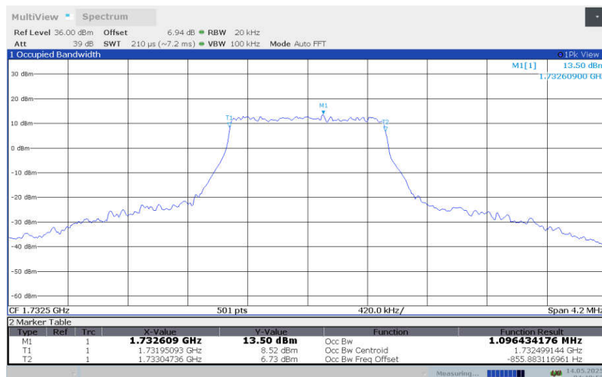
LTE band 4 , 1.4MHz Bandwidth,MID,64QAM (99% BW)
