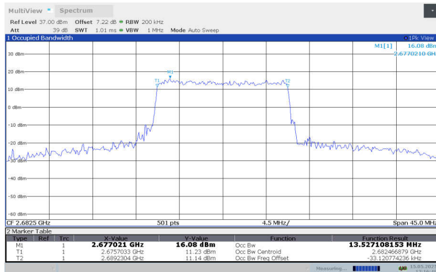
LTE band 41 , 15MHz Bandwidth,HIGH,16QAM (99% BW)
