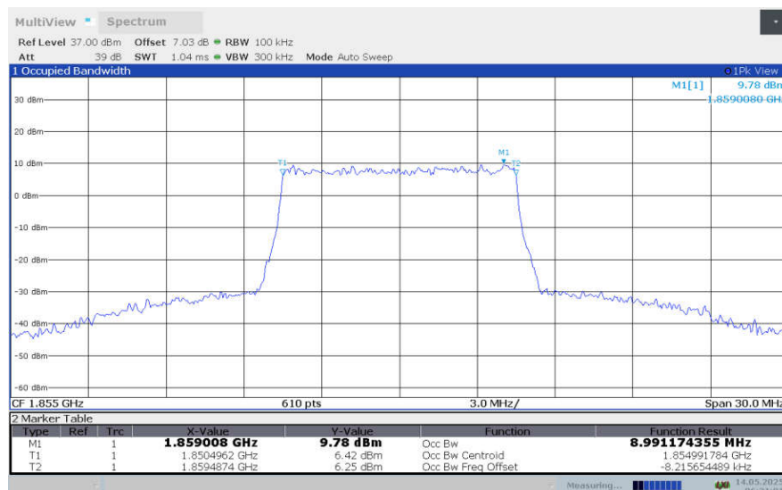
LTE band 25 , 10MHz Bandwidth,LOW,256QAM (99% BW)
