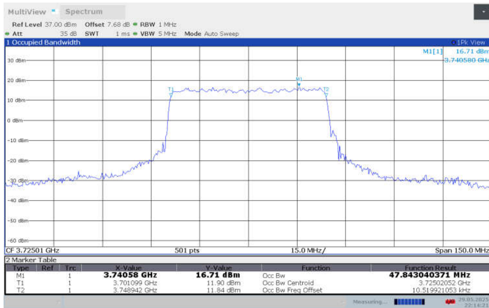
n77H,50MHz Bandwidth,CP-256QAM (99% BW)
