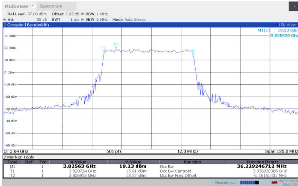
n77H,40MHz Bandwidth,DFT-s-16QAM (99% BW)
