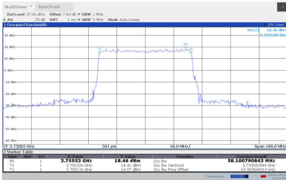
n77H,60MHz Bandwidth,DFT-s-16QAM (99% BW)
