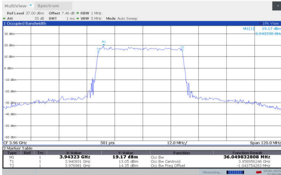
n77H,40MHz Bandwidth,DFT-s-64QAM (99% BW)
