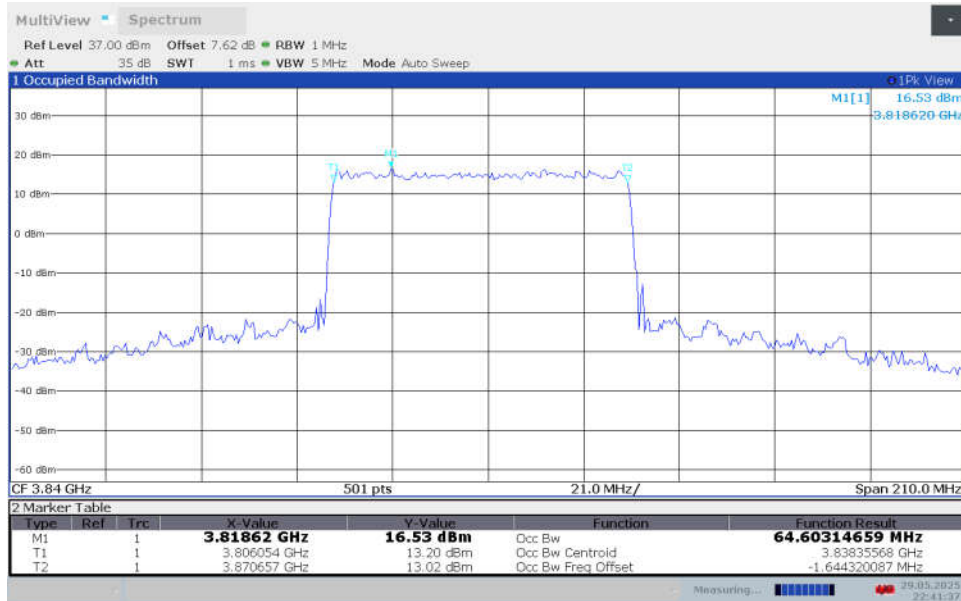
n77H,70MHz Bandwidth,DFT-s-16QAM (99% BW)
