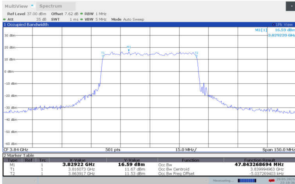
n77H,50MHz Bandwidth,CP-64QAM (99% BW)
