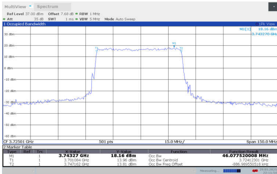
n77H,50MHz Bandwidth,DFT-s-16QAM (99% BW)
