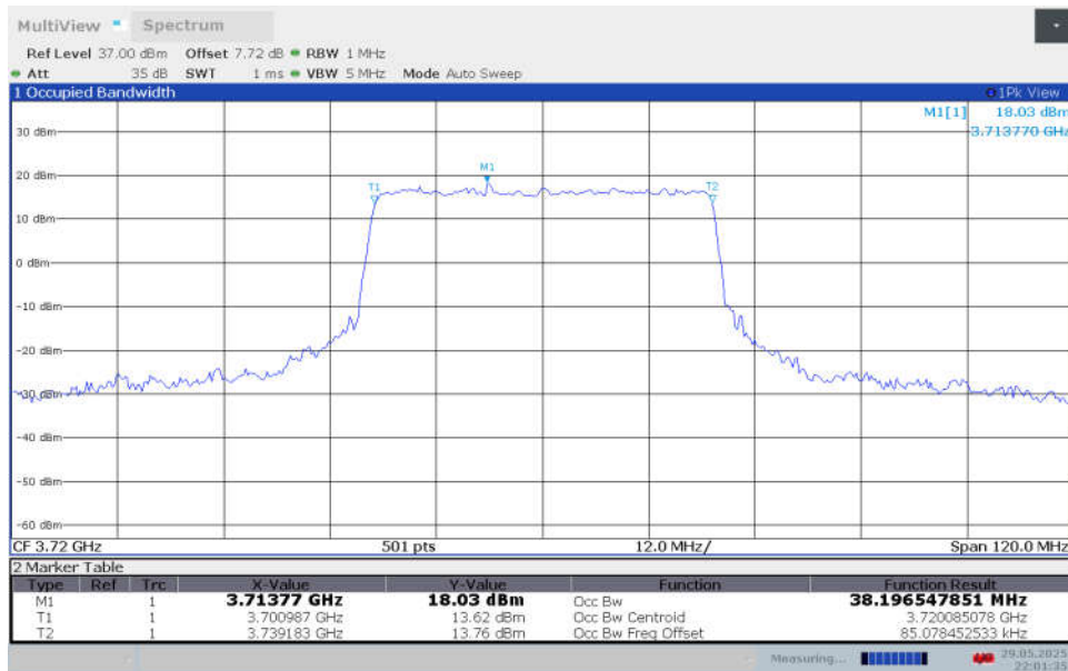
n77H,40MHz Bandwidth,CP-64QAM (99% BW)
