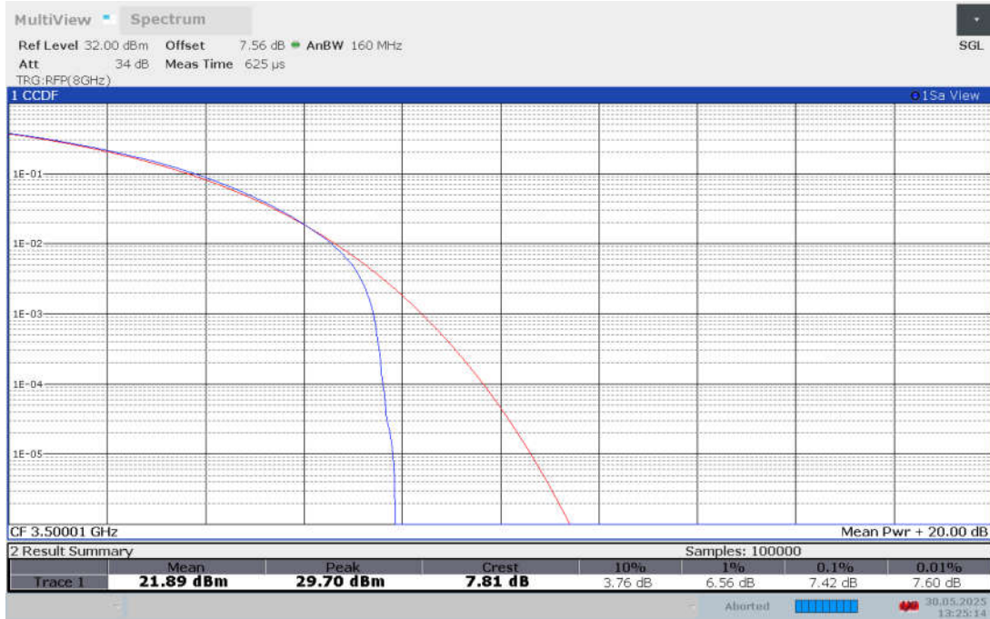
Band n78L , 90MHz Bandwidth,CP-256QAM
