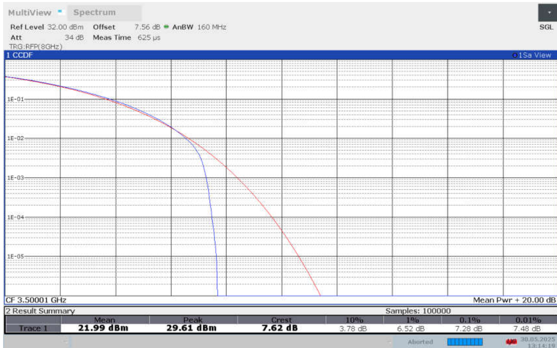
Band n78L , 50MHz Bandwidth,CP-256QAM
