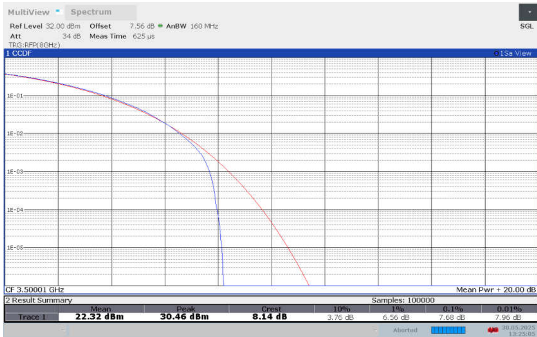
Band n78L , 90MHz Bandwidth,CP-64QAM
