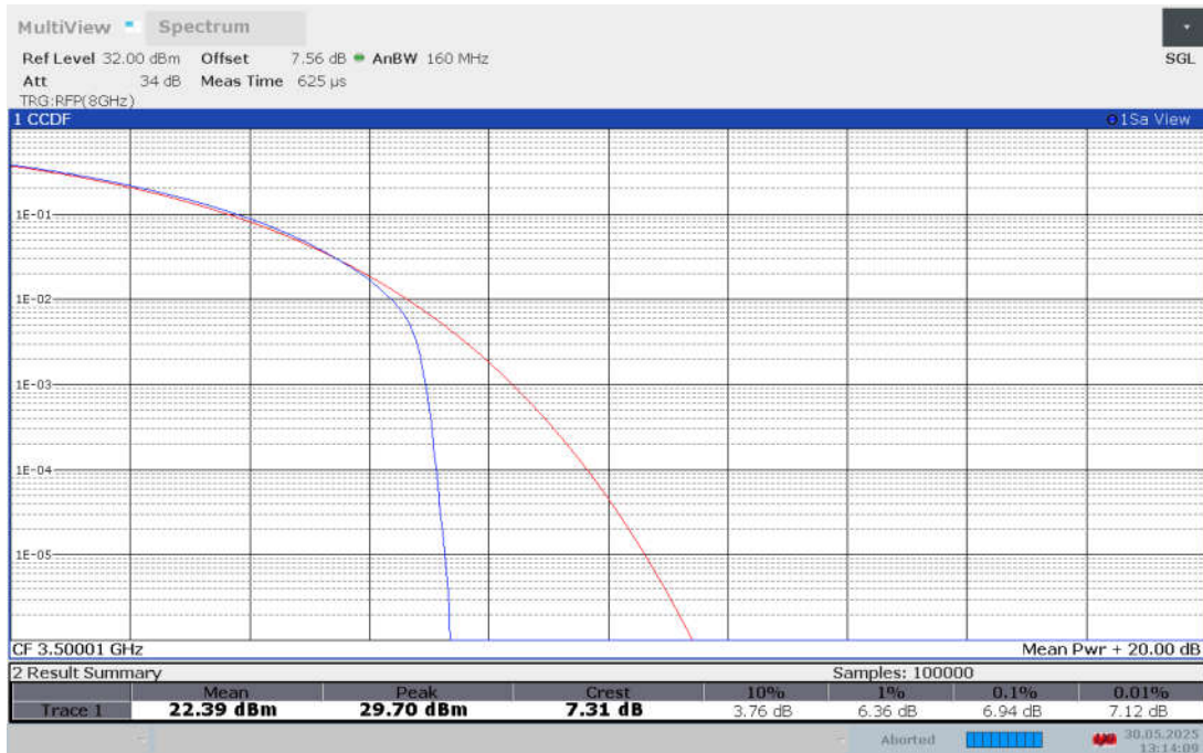
Band n78L , 50MHz Bandwidth,CP-64QAM
