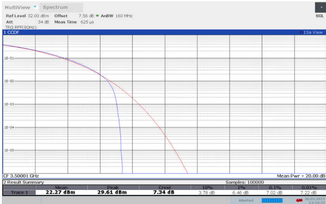
Band n78L , 70MHz Bandwidth,CP-16QAM
