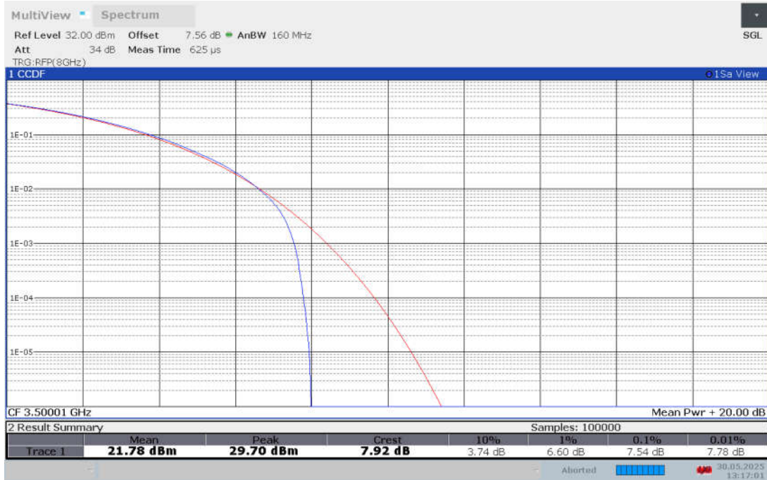
Band n78L , 60MHz Bandwidth,CP-256QAM
