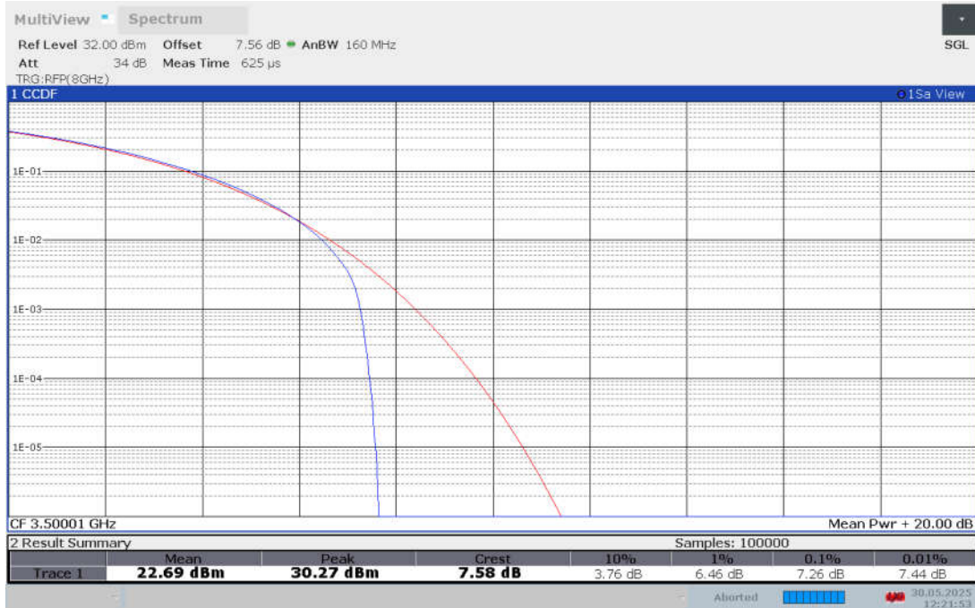
Band n77L , 40MHz Bandwidth,CP-16QAM
