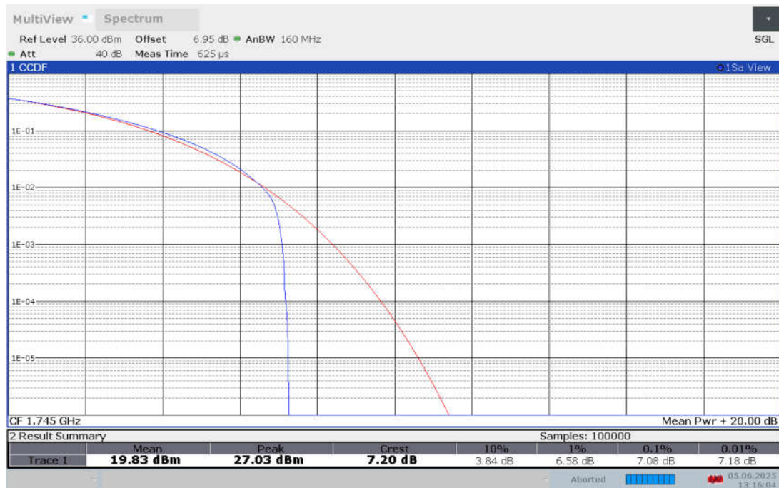
Band n66 , 10MHz Bandwidth,CP-64QAM
