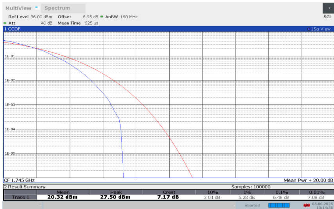
Band n66 , 10MHz Bandwidth,DFT-s-256QAM
