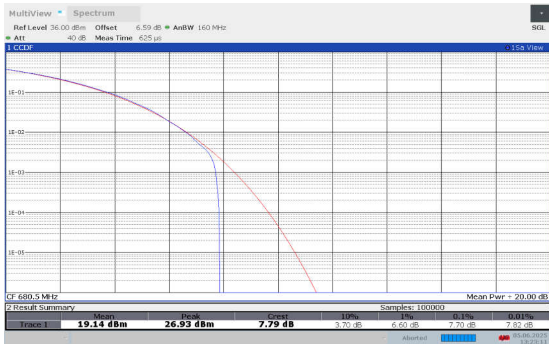
Band n71 , 5MHz Bandwidth,CP-256QAM
