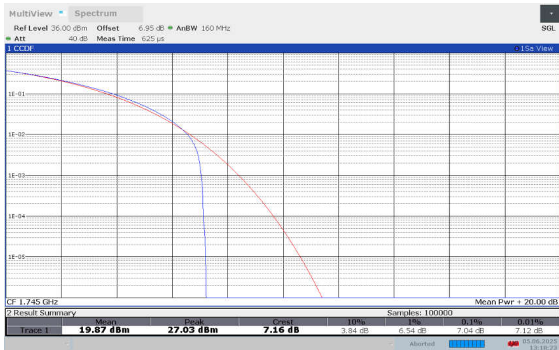
Band n66 , 15MHz Bandwidth,CP-64QAM
