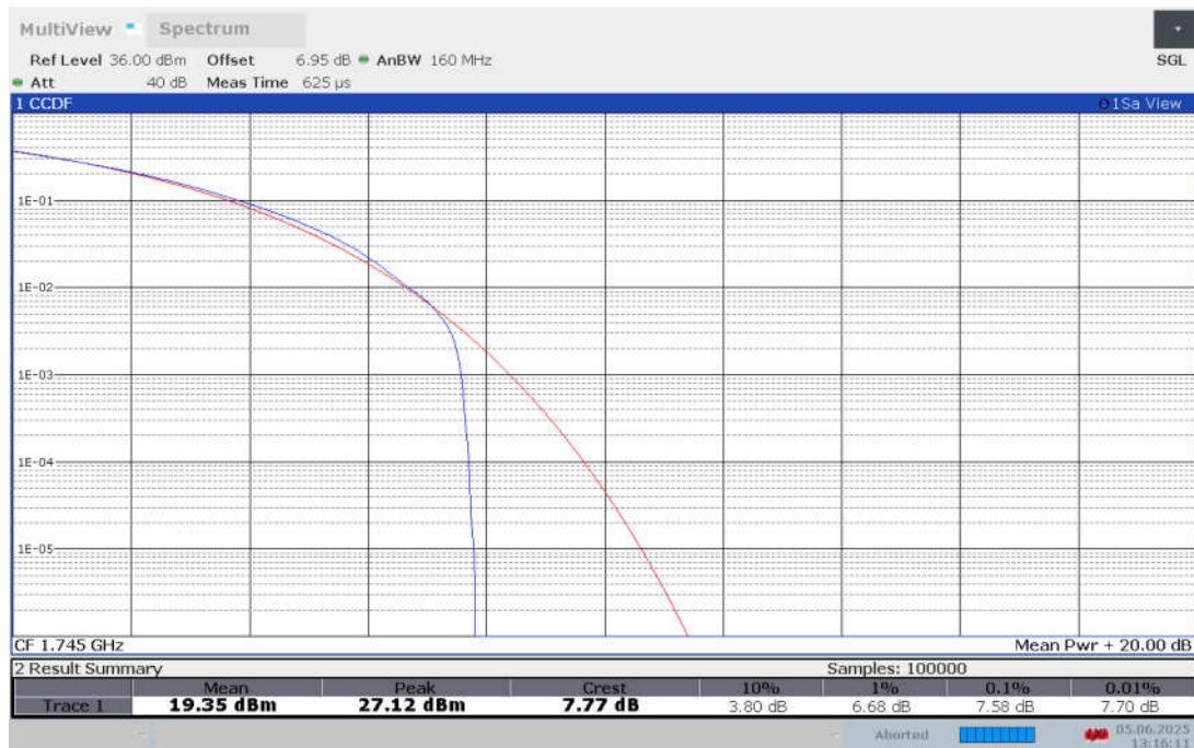
Band n66 , 10MHz Bandwidth,CP-256QAM
