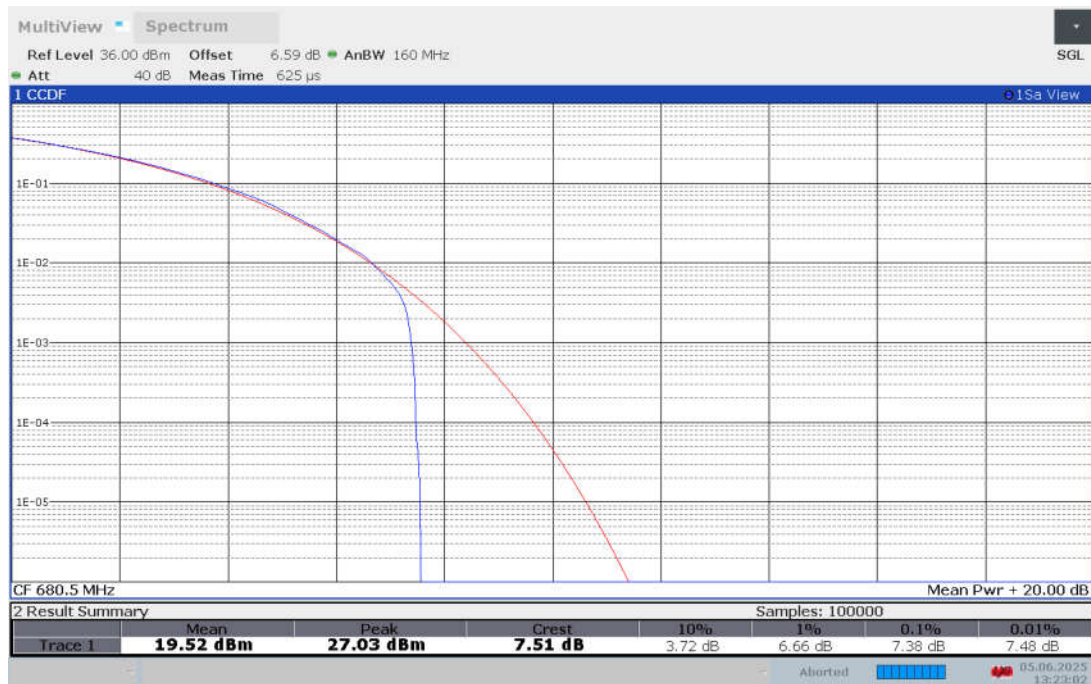
Band n71 , 5MHz Bandwidth,CP-64QAM
