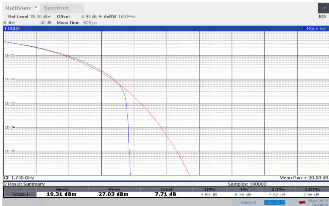
Band n66 , 15MHz Bandwidth,CP-256QAM
