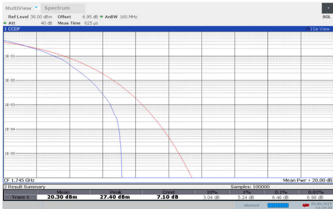
Band n66 , 20MHz Bandwidth,DFT-s-256QAM
