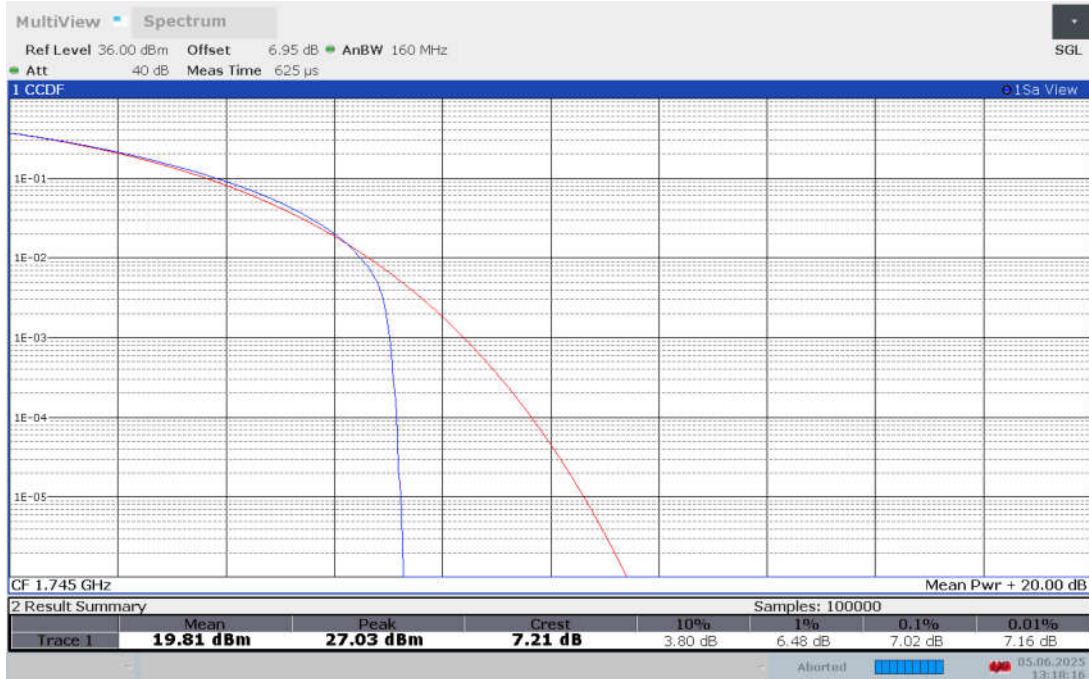
Band n66 , 15MHz Bandwidth,CP-16QAM
