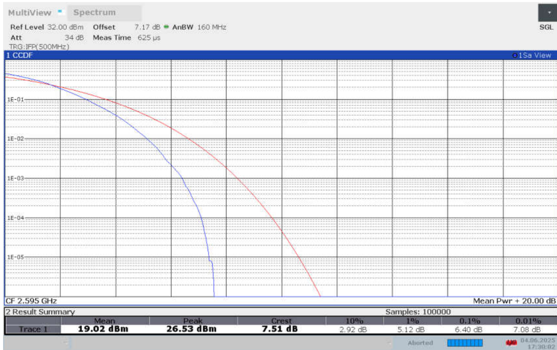
Band n38 , 30MHz Bandwidth,CP-QPSK
