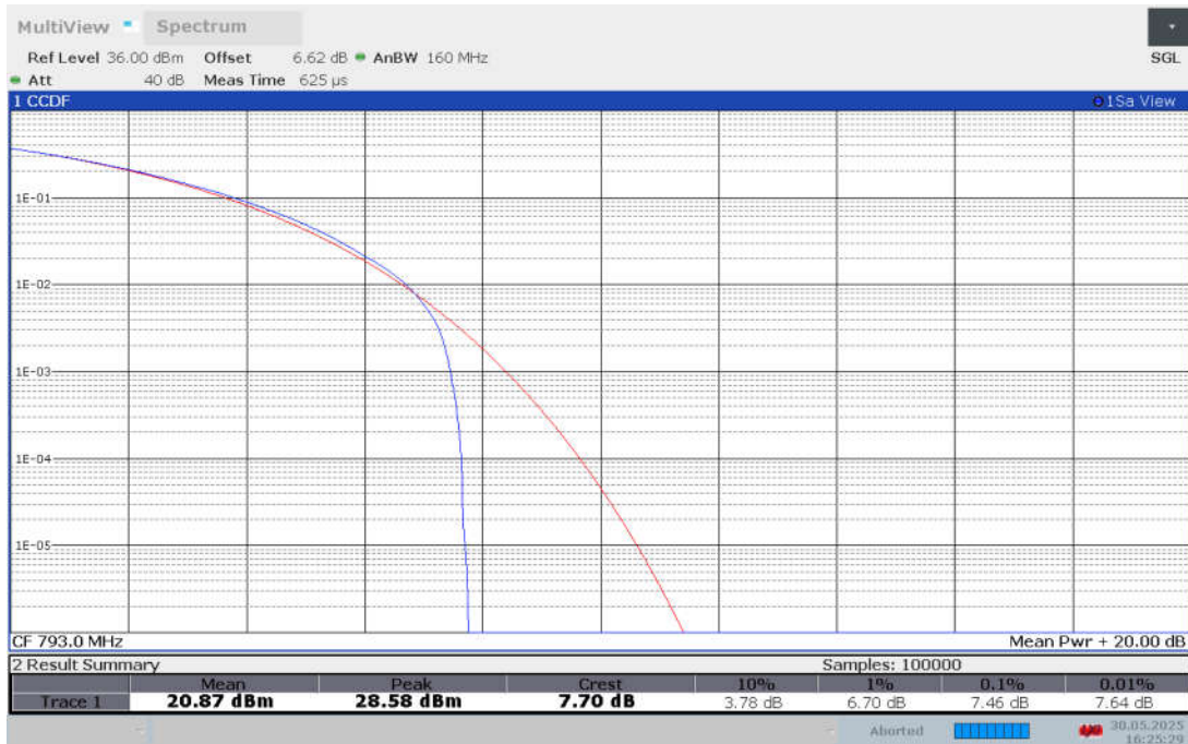
Band n14 , 10MHz Bandwidth,CP-64QAM
