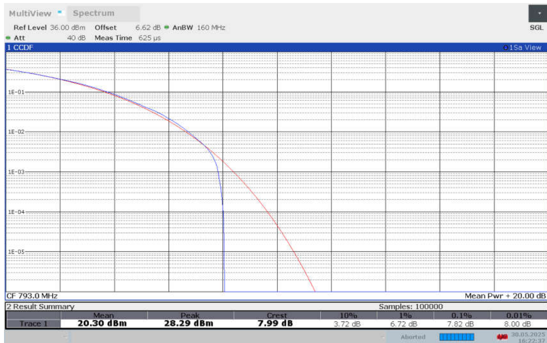
Band n14 , 5MHz Bandwidth,CP-256QAM
