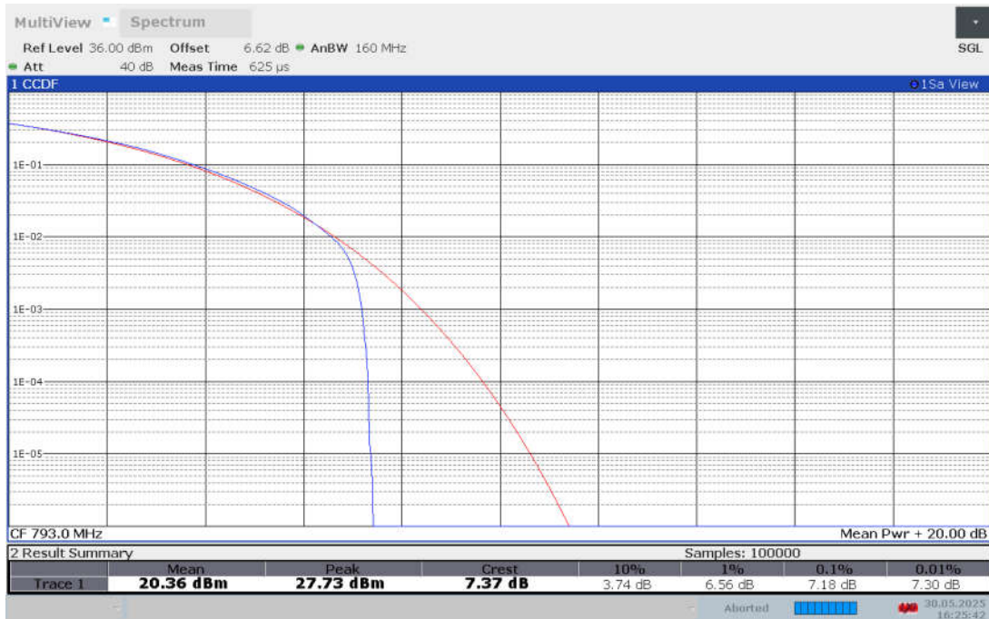
Band n14 , 10MHz Bandwidth,CP-256QAM
