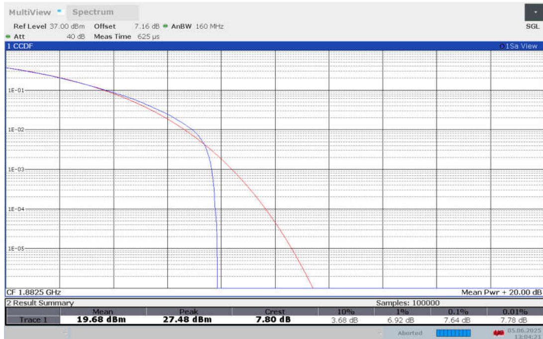
Band n25 , 5MHz Bandwidth,CP-16QAM
