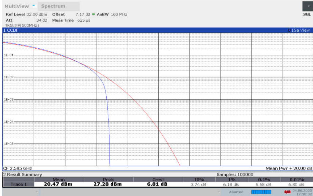
Band n38 , 30MHz Bandwidth,CP-16QAM
