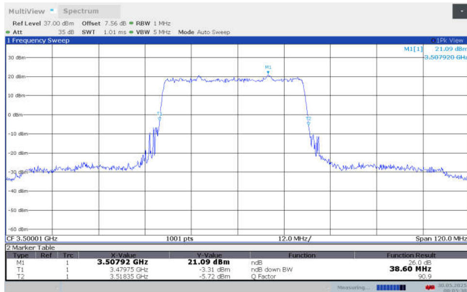
n78L,40MHz Bandwidth,DFT-s-pi/2 BPSK (-26dBc BW)
