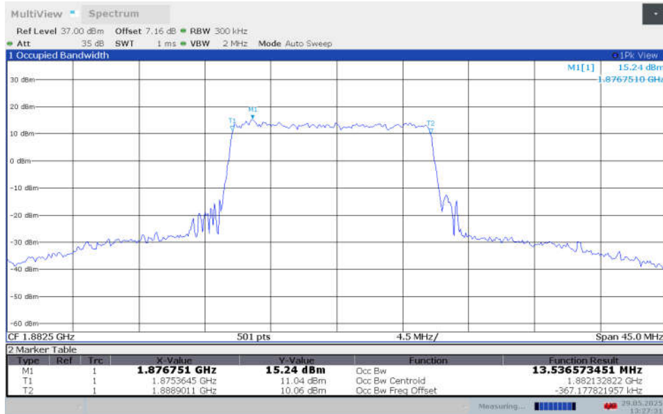
n25,15MHz Bandwidth,DFT-s-16QAM (99% BW)
