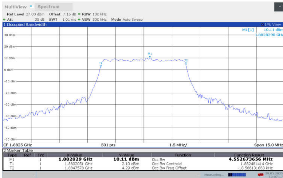
n25,5MHz Bandwidth,CP-256QAM (99% BW)
