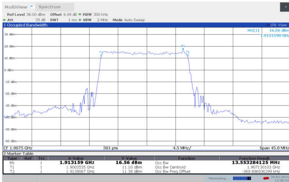
n25,15MHz Bandwidth,DFT-s-QPSK (99% BW)
