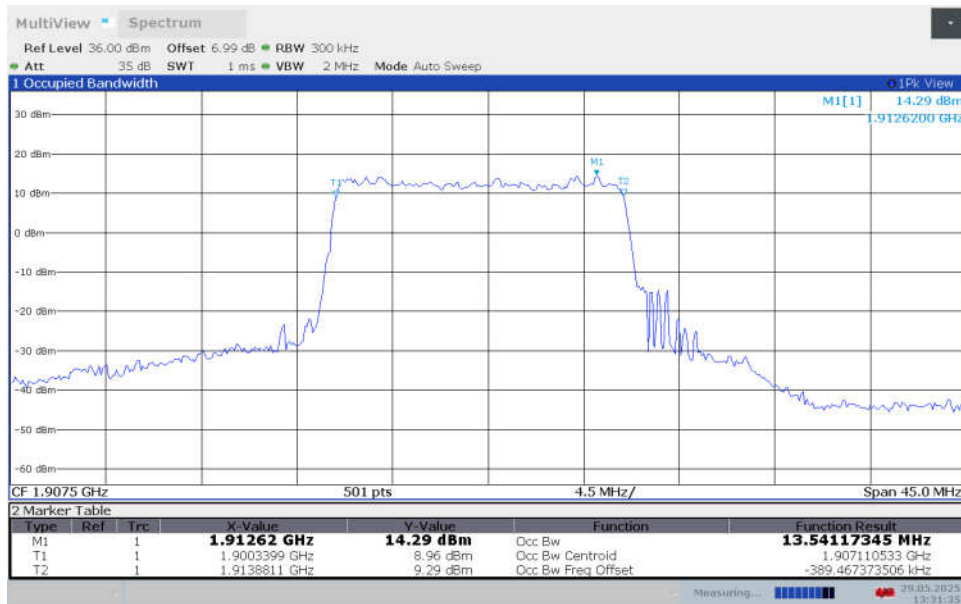
n25,15MHz Bandwidth,DFT-s-64QAM (99% BW)
