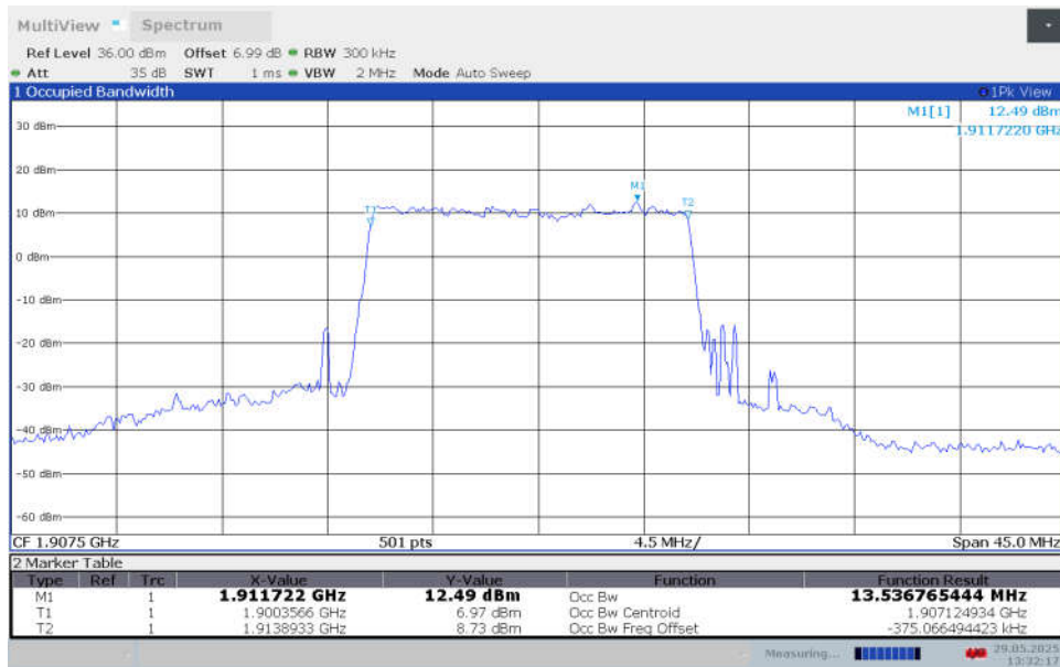
n25,15MHz Bandwidth,CP-QPSK (99% BW)
