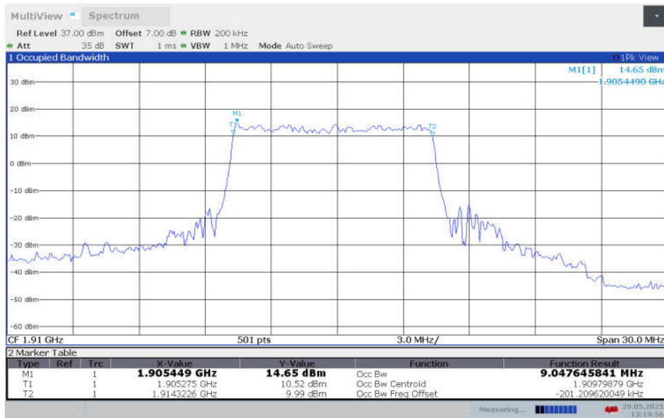
n25,10MHz Bandwidth,DFT-s-64QAM (99% BW)
