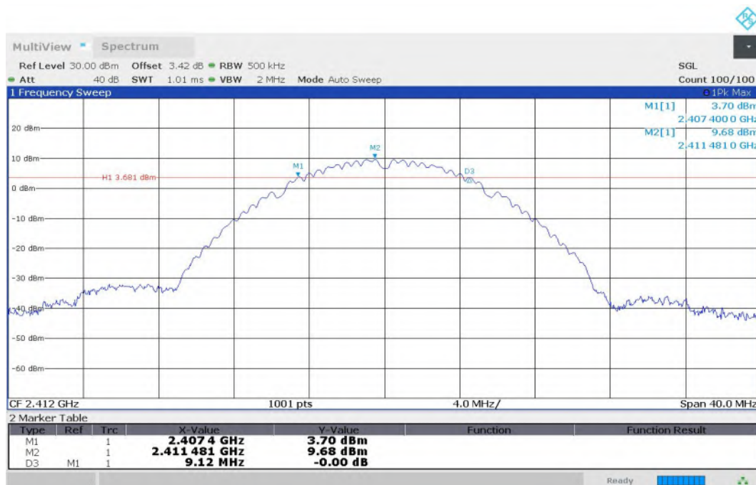
Fig.4 6dB Bandwidth (802.11b, CH1)
