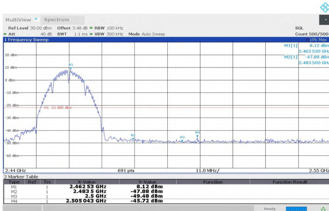
Fig.11 Band Edges (802.11b, CH11)
