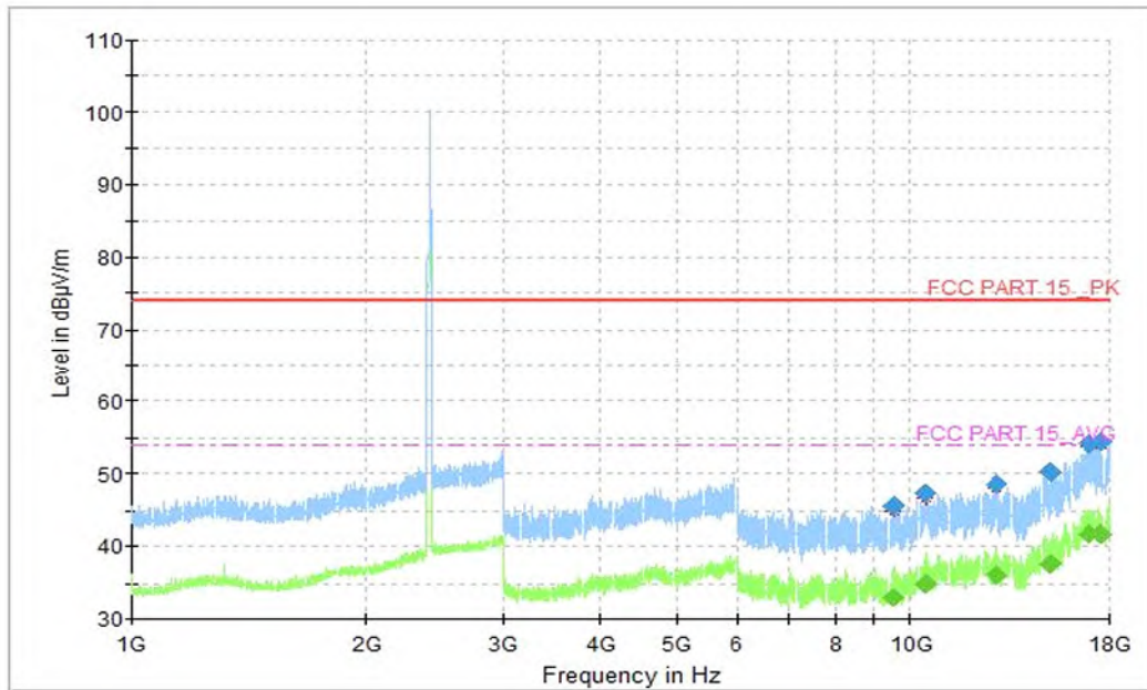
Fig.27 Radiated Spurious Emission (802.11b, CH1, 1GHz-18GHz)
