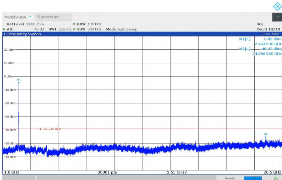
Fig.19 Conducted Spurious Emission (1GHz-26.5GHz, 802.11g, CH11)
