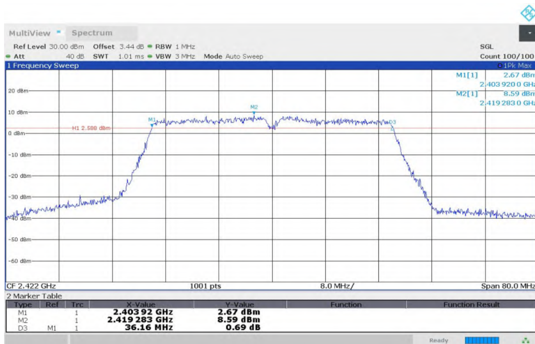
Fig.7 6dB Bandwidth (802.11n-HT40, CH3)
