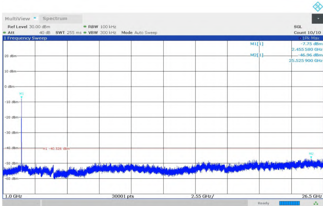
Fig.22 Conducted Spurious Emission (1GHz-26.5GHz, 802.11n-HT20, CH11)
