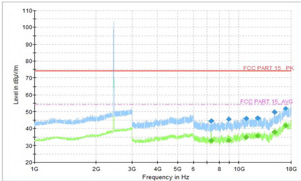
Fig.37 Radiated Spurious Emission (802.11n-HT20, CH1, 1GHz-18GHz)
