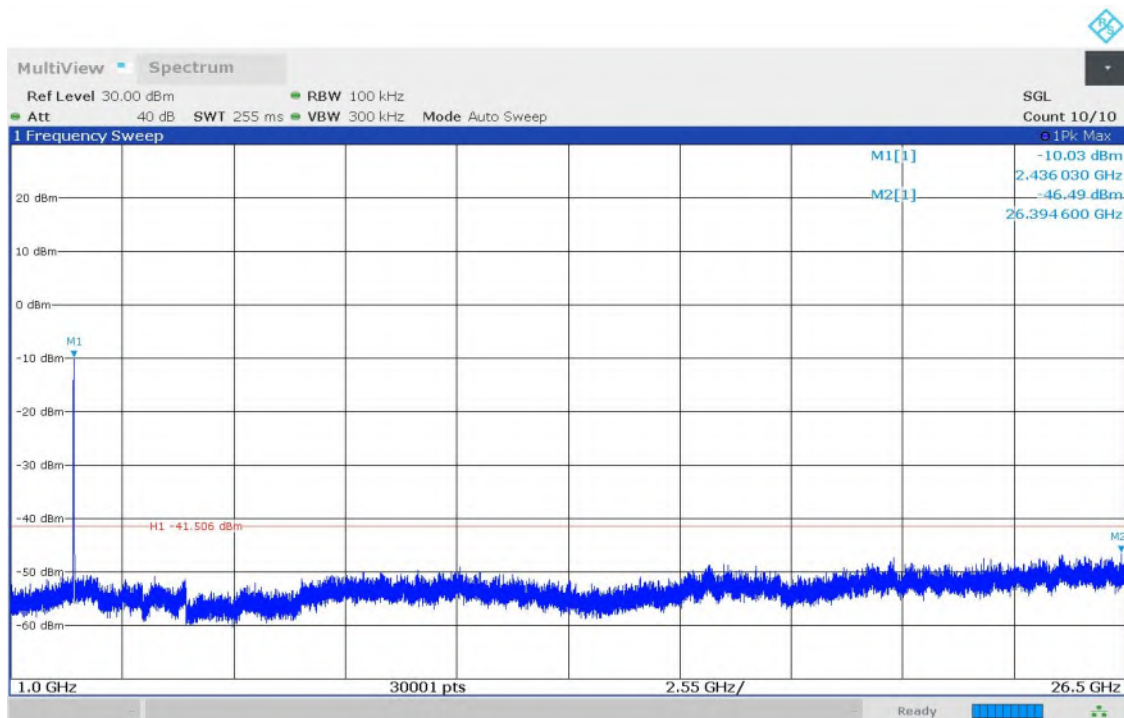
Fig.21 Conducted Spurious Emission (1GHz-26.5GHz, 802.11n-HT20, CH6)
