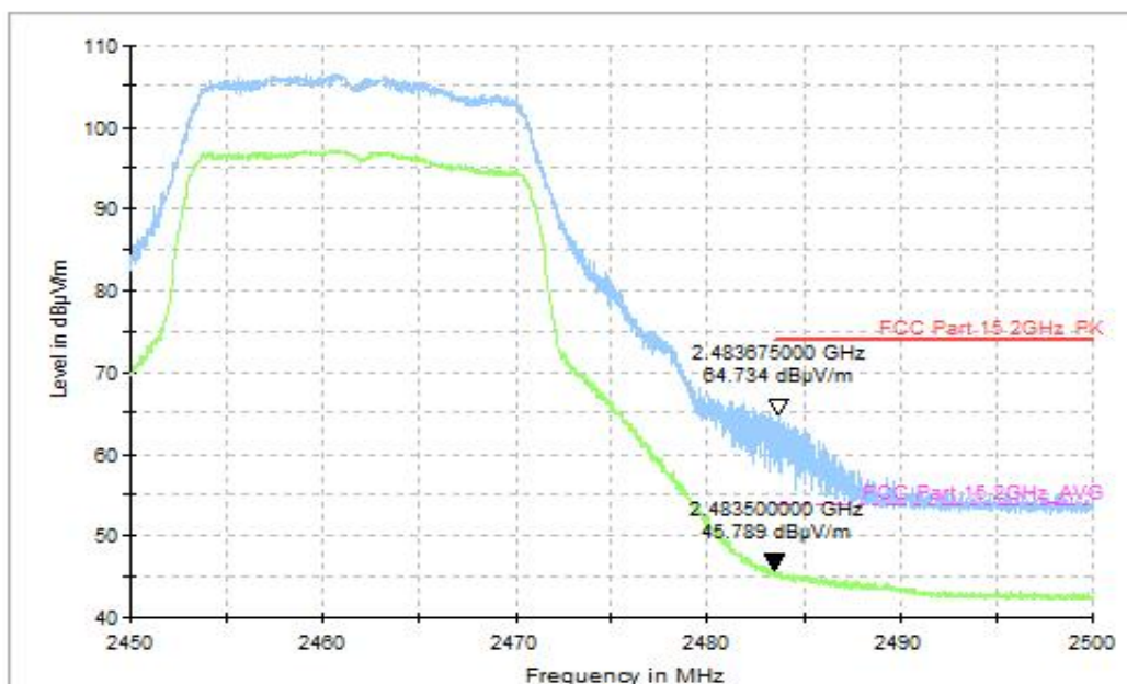
Fig.41 Radiated Restricted Band (802.11n-HT20, CH11, 2.45GHz~2.50GHz)
