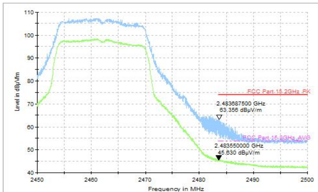
Fig.36 Radiated Restricted Band (802.11g, CH11, 2.45GHz~2.50GHz)
