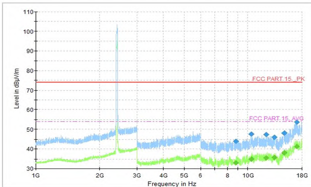
Fig.32 Radiated Spurious Emission (802.11g, CH1, 1GHz-18GHz)
