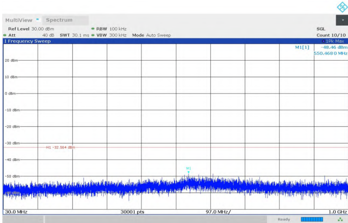
Fig.26 Conducted Spurious Emission (All Channels, 30MHz -1GHz)
