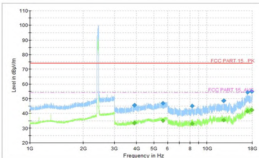
Fig.42 Radiated Spurious Emission (802.11n-HT40, CH3, 1GHz-18GHz)
