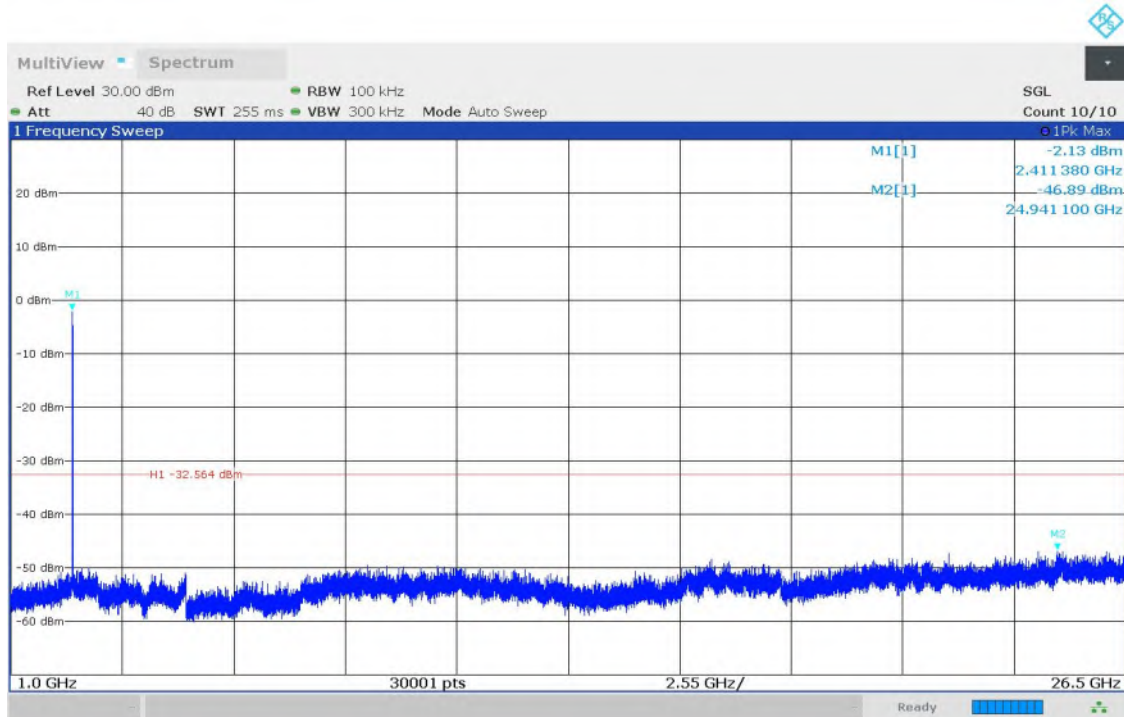
Fig.14 Conducted Spurious Emission (1GHz-26.5GHz, 802.11b, CH1)
