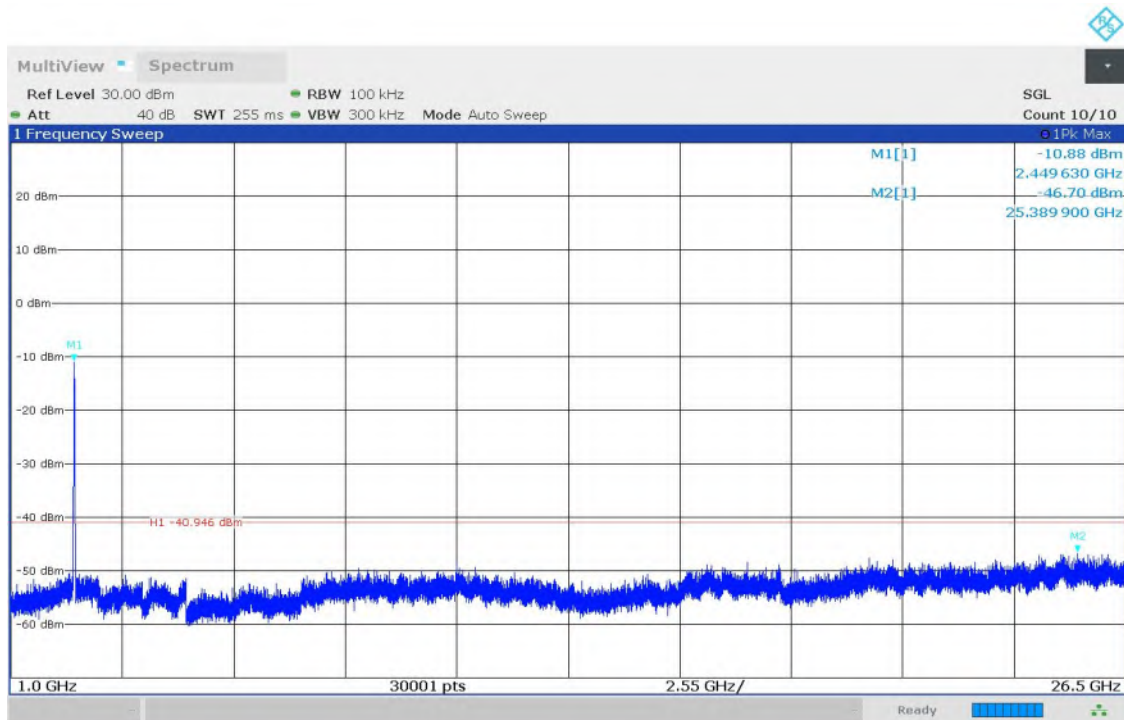
Fig.25 Conducted Spurious Emission (1GHz-26.5GHz, 802.11n-HT40, CH9)
