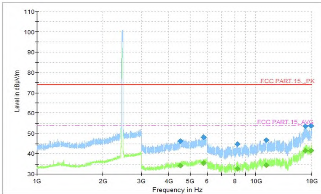
Fig.44 Radiated Spurious Emission (802.11n-HT40, CH9, 1GHz-18GHz)
