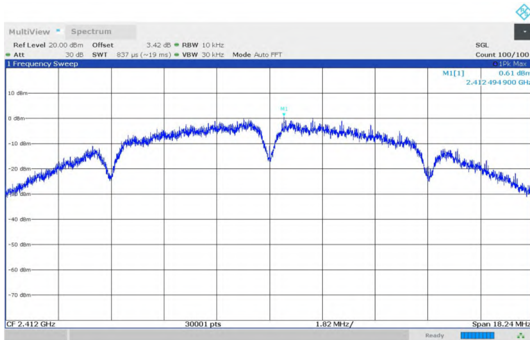
Fig.1 Power Spectral Density (802.11b, CH1)
