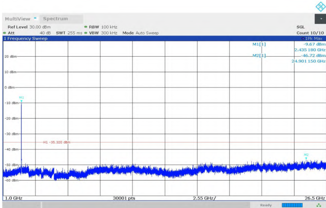
Fig.18 Conducted Spurious Emission (1GHz-26.5GHz, 802.11g, CH6)
