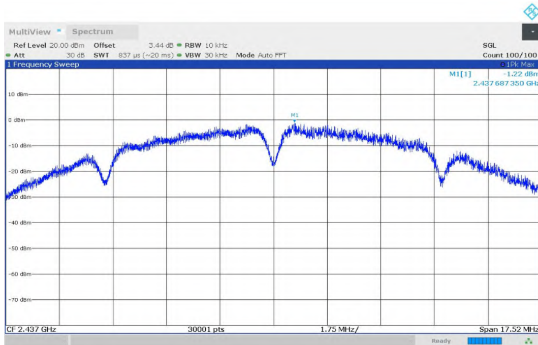
Fig.2 Power Spectral Density (802.11b, CH6)
