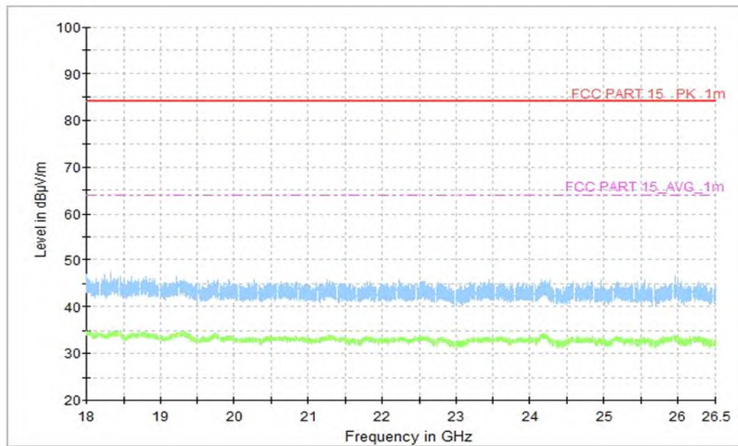
Fig.49 Radiated Spurious Emission (All Channels, 18GHz-26.5GHz)
