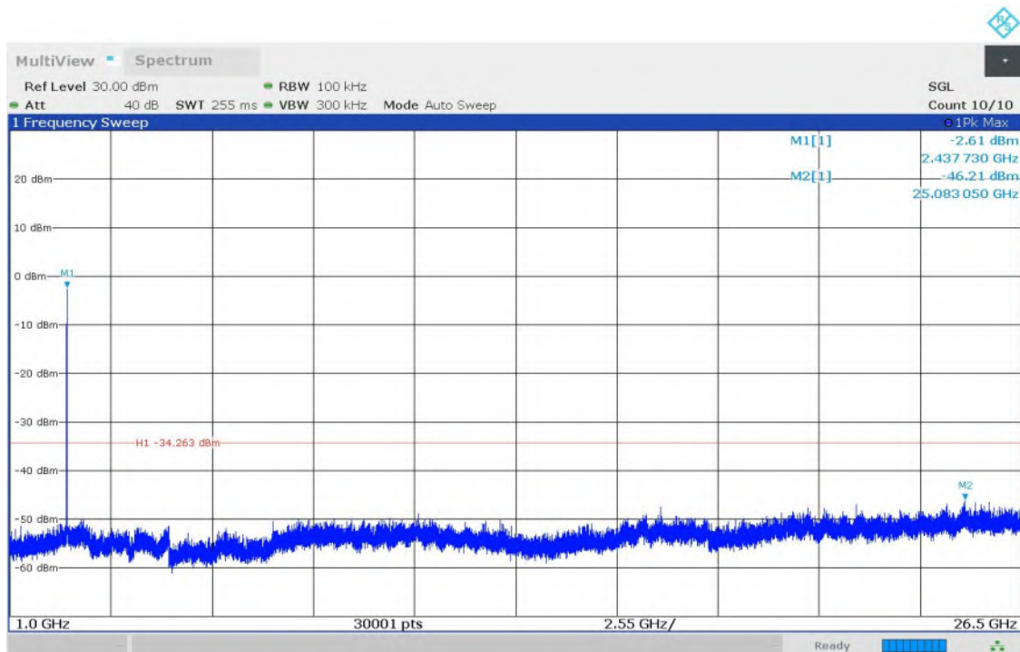
Fig.15 Conducted Spurious Emission (1GHz-26.5GHz, 802.11b, CH6)
