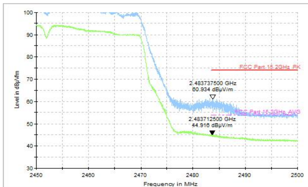
Fig.46 Radiated Restricted Band (802.11n-HT40, CH9, 2.45GHz~2.50GHz)
