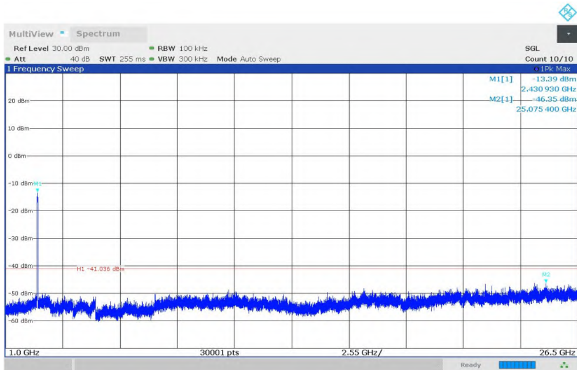
Fig.23 Conducted Spurious Emission (1GHz-26.5GHz, 802.11n-HT40, CH3)
