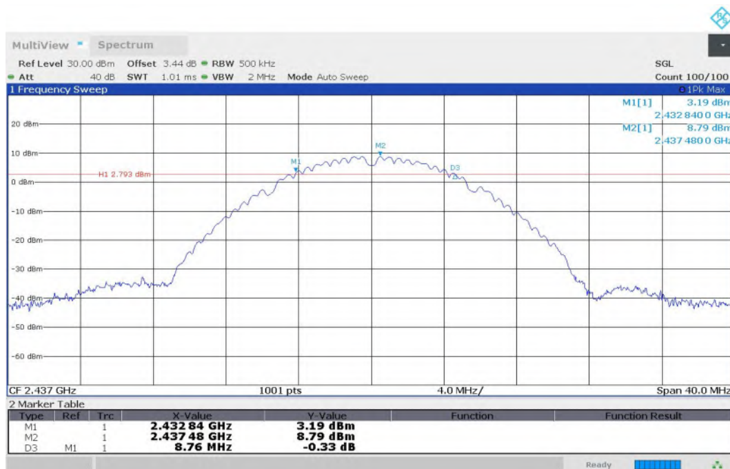
Fig.5 6dB Bandwidth (802.11b, CH6)
