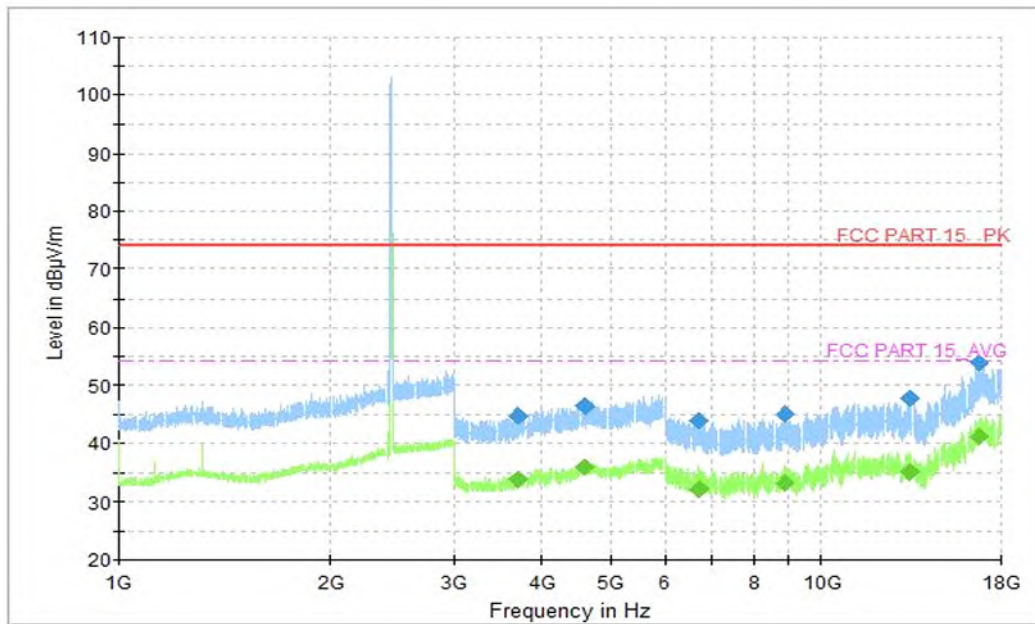
Fig.38 Radiated Spurious Emission (802.11n-HT20, CH6, 1GHz-18GHz)
