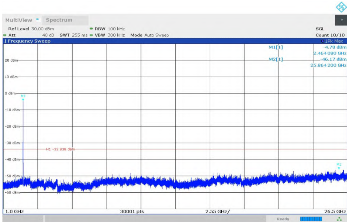
Fig.16 Conducted Spurious Emission (1GHz-26.5GHz, 802.11b, CH11)
