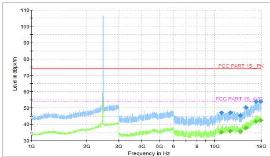
Fig.29 Radiated Spurious Emission (802.11b, CH11, 1GHz-18GHz)
