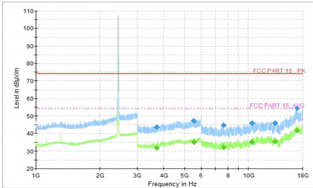
Fig.33 Radiated Spurious Emission (802.11g, CH6, 1GHz-18GHz)
