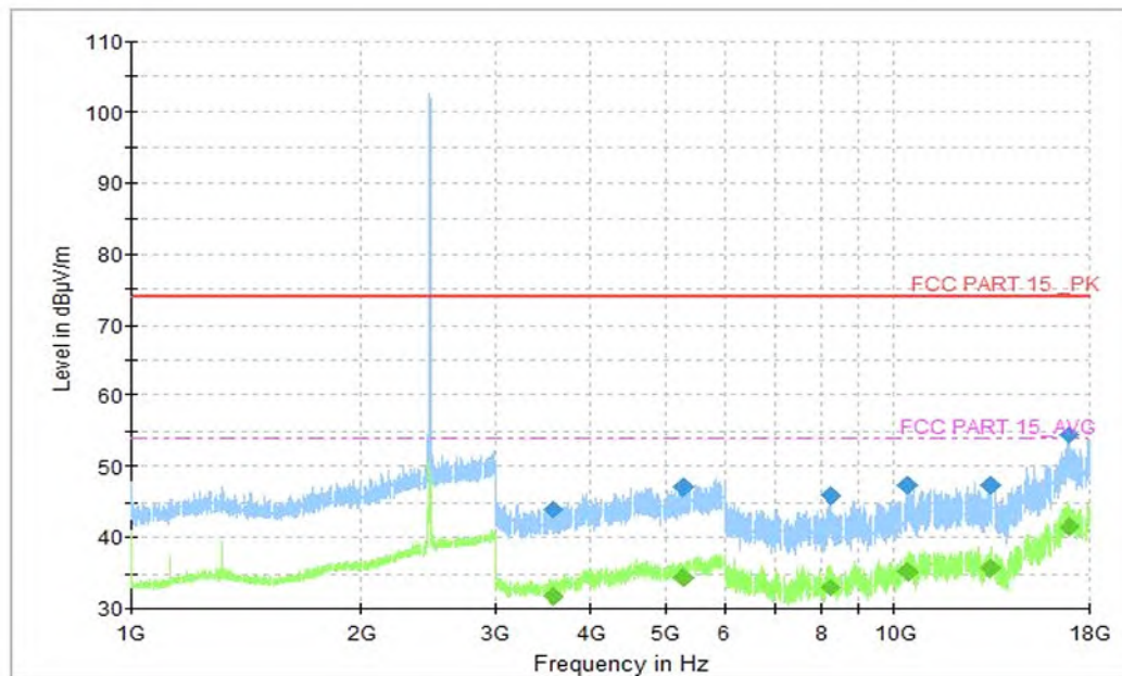
Fig.39 Radiated Spurious Emission (802.11n-HT20, CH11, 1GHz-18GHz)
