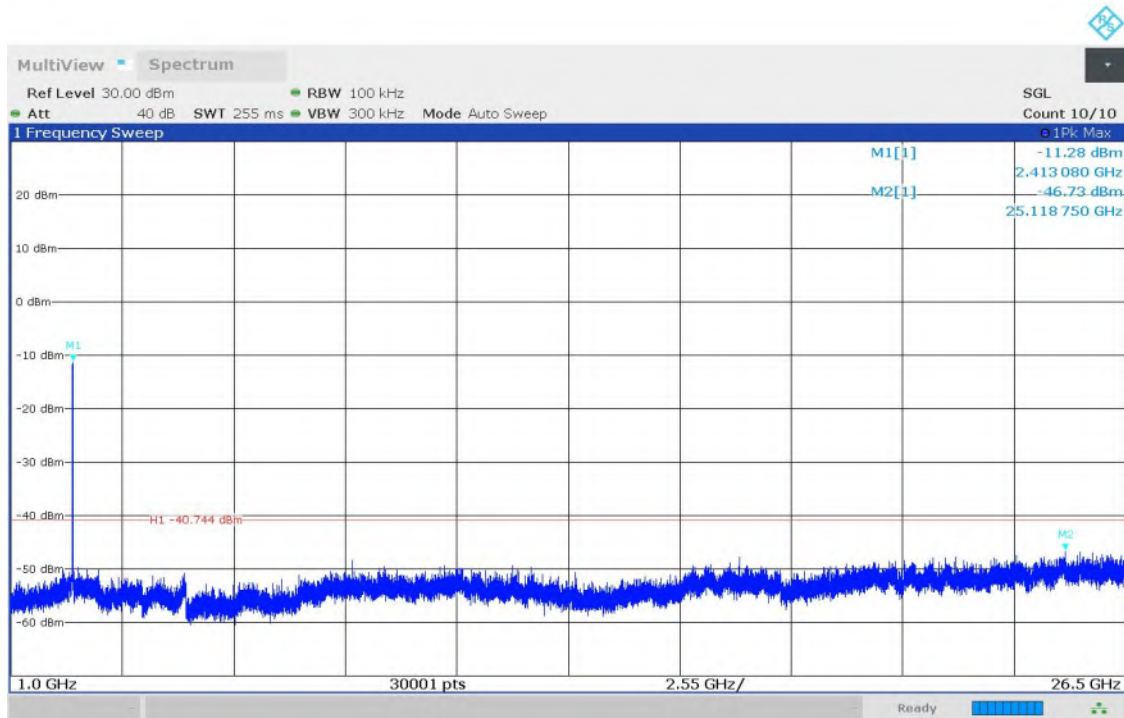
Fig.20 Conducted Spurious Emission (1GHz-26.5GHz, 802.11n-HT20, CH1)
