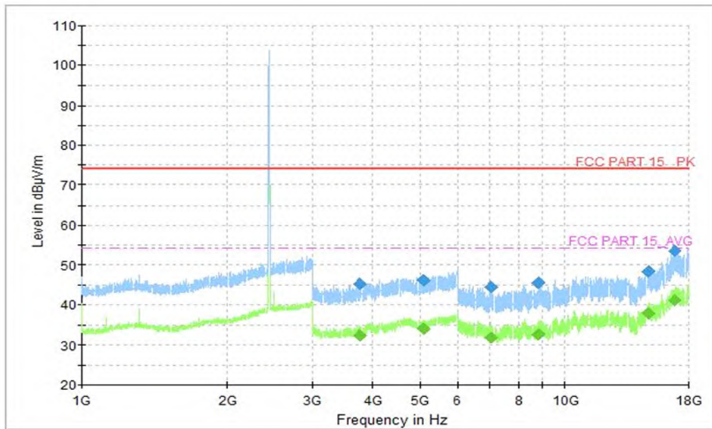
Fig.28 Radiated Spurious Emission (802.11b, CH6, 1GHz-18GHz)
