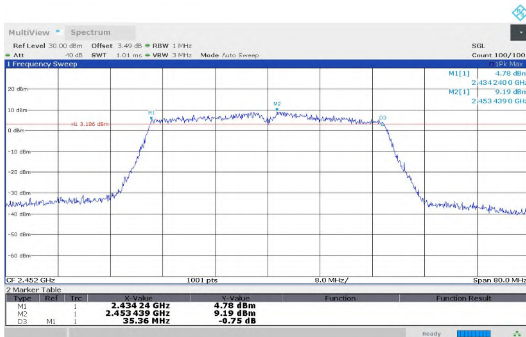
Fig.9 6dB Bandwidth (802.11n-HT40, CH9)
