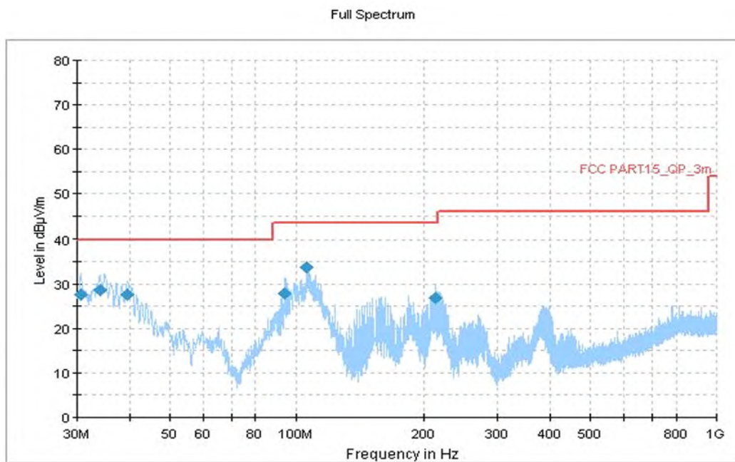
Fig.48 Radiated Spurious Emission (All Channels, 30MHz-1GHz)
