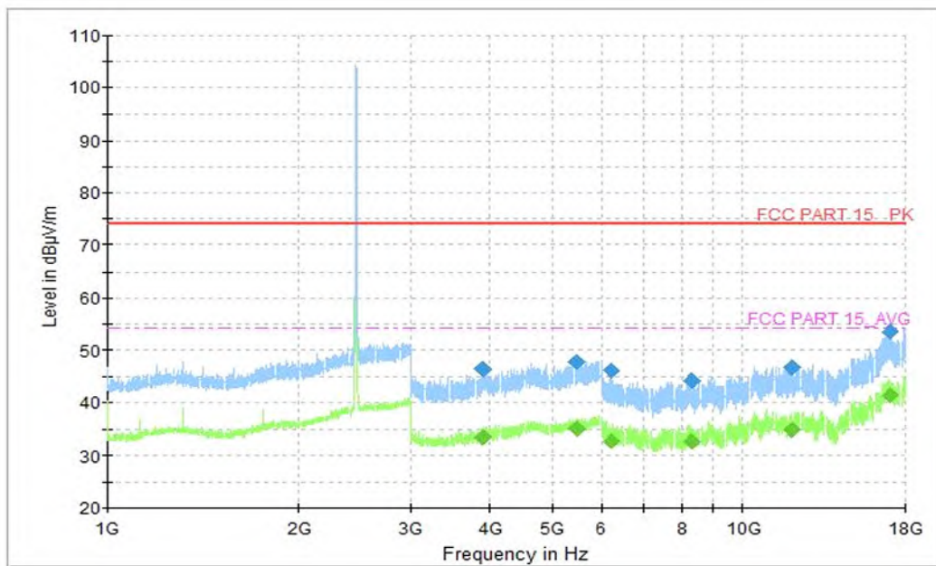
Fig.34 Radiated Spurious Emission (802.11g, CH11, 1GHz-18GHz)
