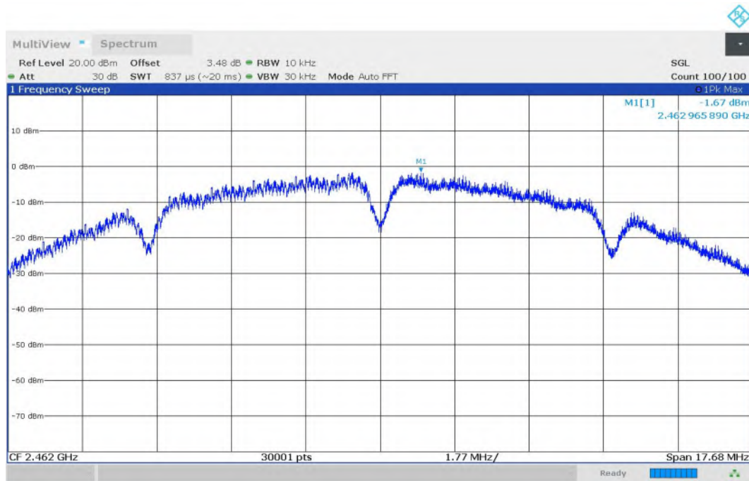
Fig.3 Power Spectral Density (802.11b, CH11)
