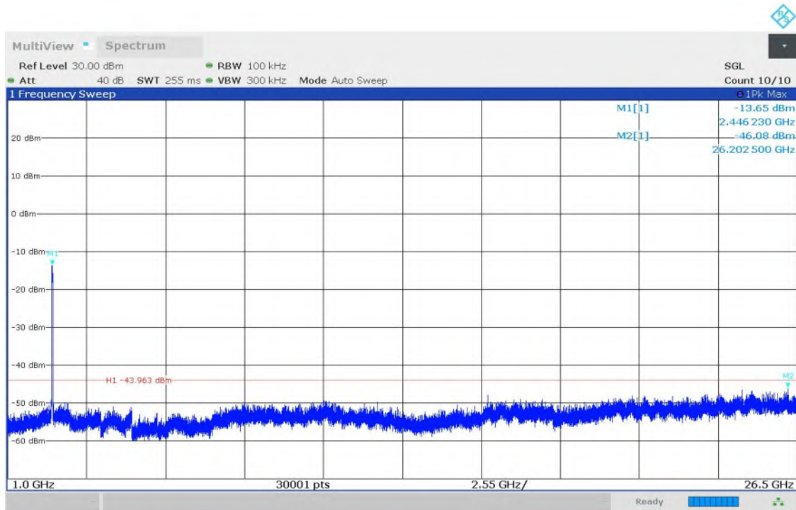
Fig.24 Conducted Spurious Emission (1GHz-26.5GHz, 802.11n-HT40, CH6)
