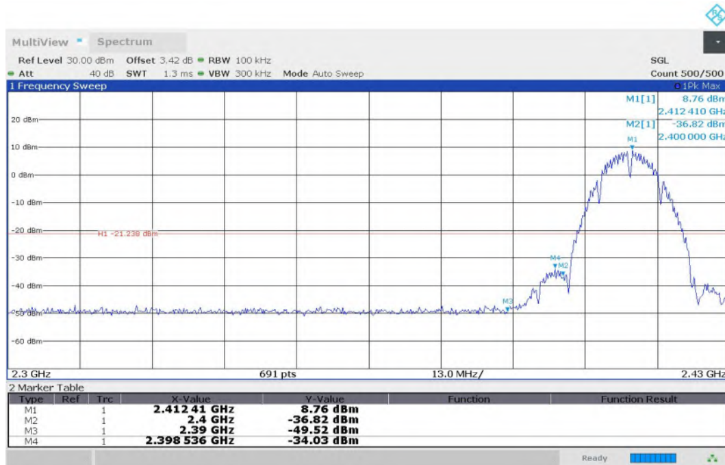
Fig.10 Band Edges (802.11b, CH1)
