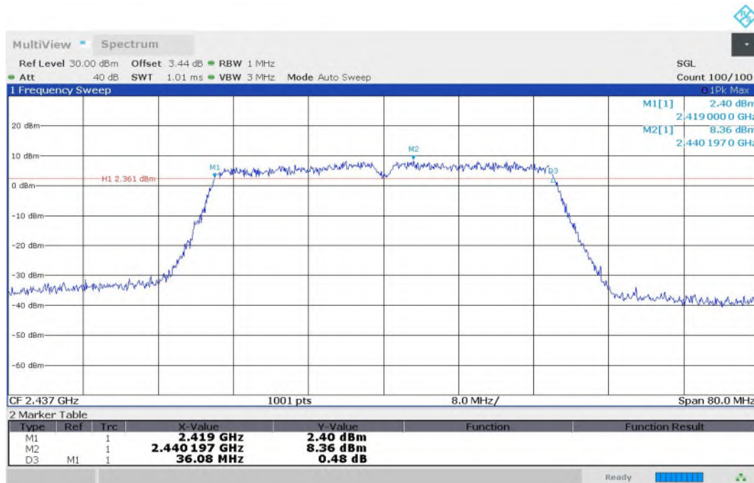
Fig.8 6dB Bandwidth (802.11n-HT40, CH6)
