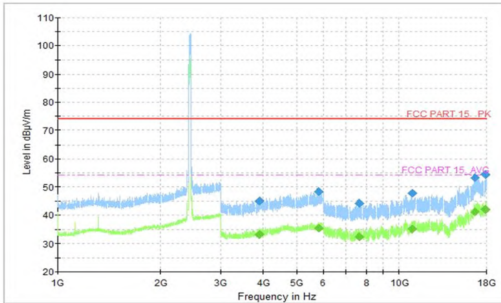
Fig.43 Radiated Spurious Emission (802.11n-HT40, CH6, 1GHz-18GHz)
