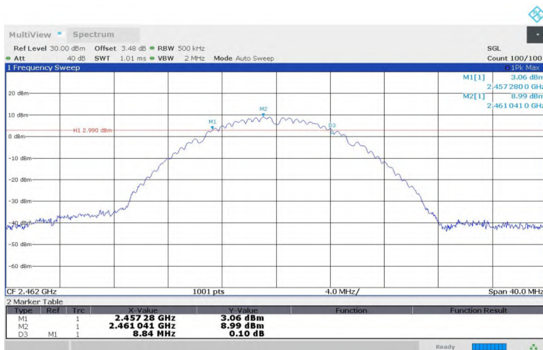
Fig.6 6dB Bandwidth (802.11b, CH11)
