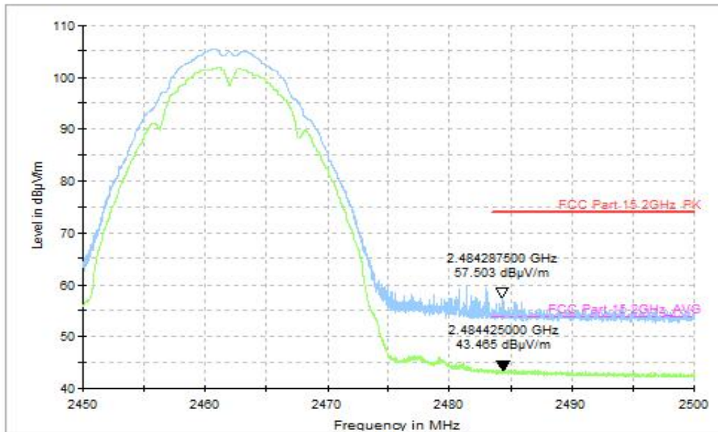
Fig.31 Radiated Restricted Band (802.11b, CH11, 2.45GHz~2.50GHz)
