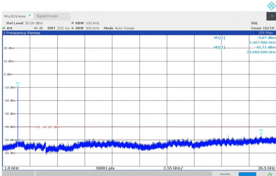
Fig.17 Conducted Spurious Emission (1GHz-26.5GHz, 802.11g, CH1)
