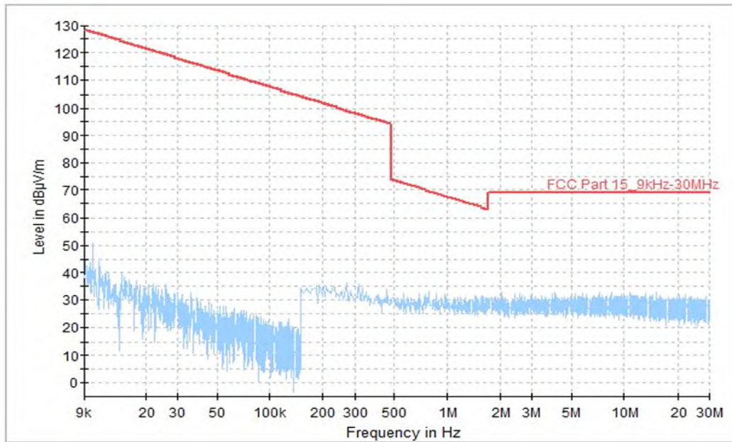
Fig.47 Radiated Spurious Emission (All Channels, 9kHz-30MHz)
