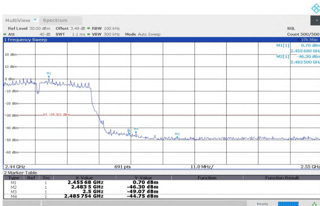
Fig.13 Band Edges (802.11n-HT40, CH9)
