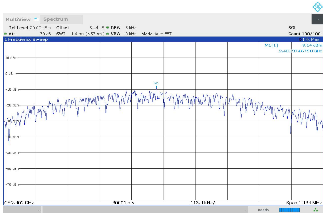
Fig.1 Power Spectral Density (CH0), LE 1M
