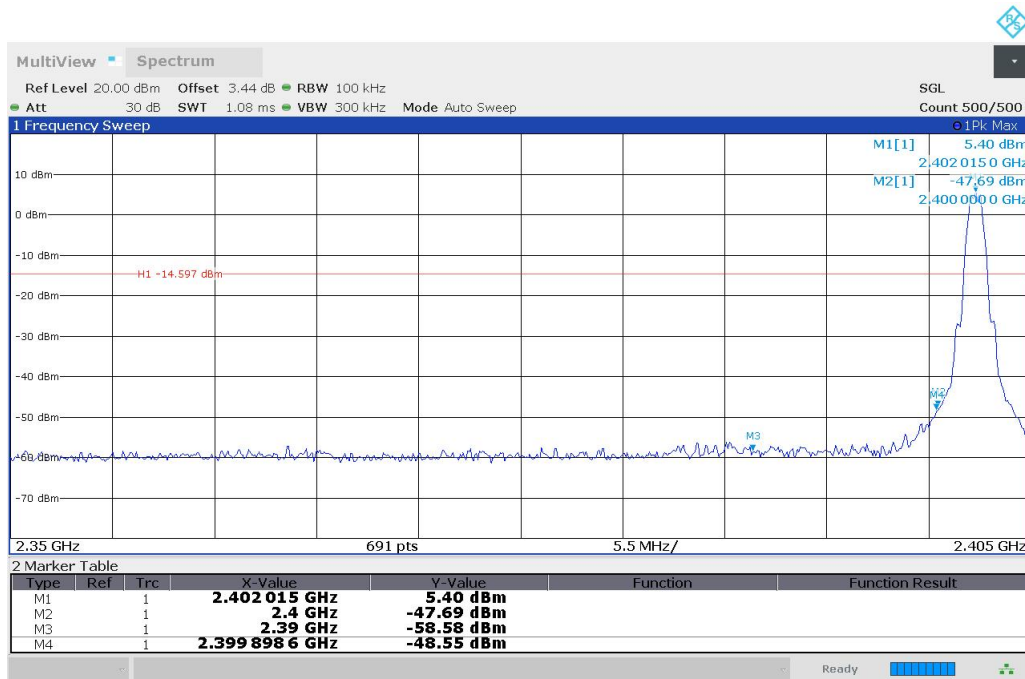
Fig.7 Band Edges (CH0), LE 1M
