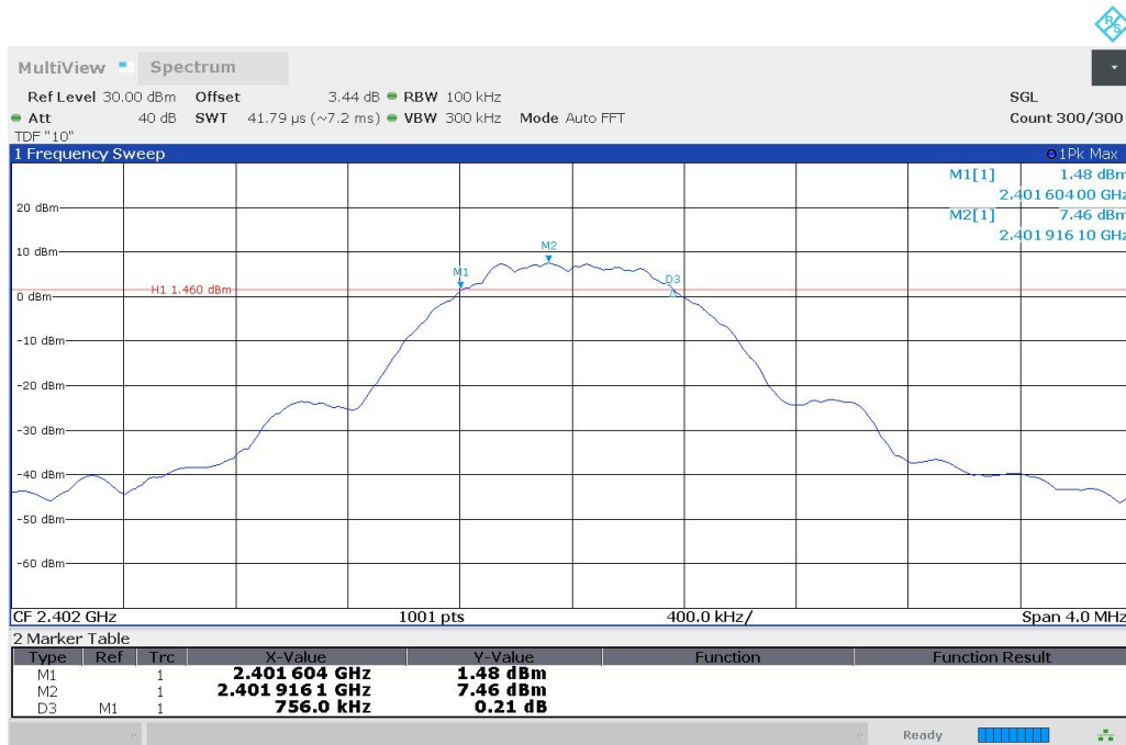
Fig.4 6dB Bandwidth (CH0), LE 1M
