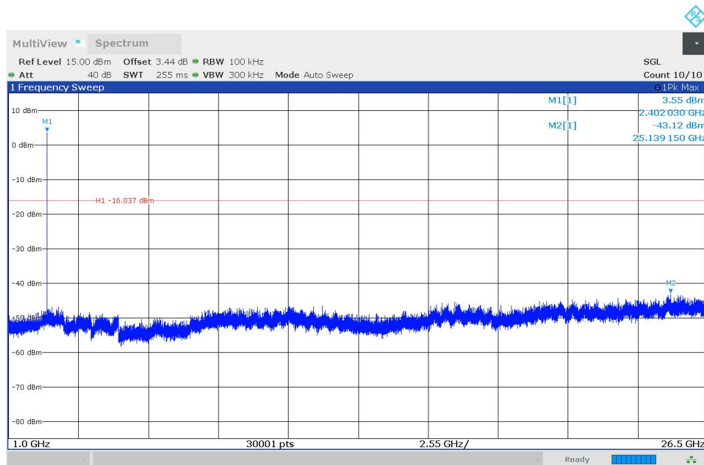
Fig.9 Conducted Spurious Emission (CH0, 1GHz-26.5GHz), LE 1M
