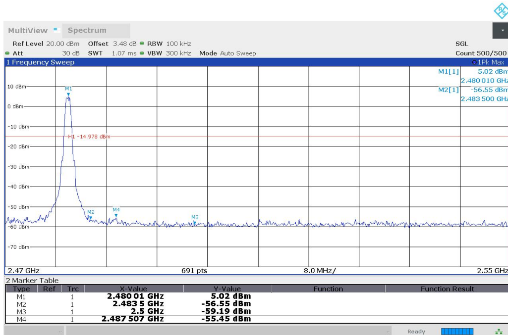
Fig.8 Band Edges (CH39), LE 1M
