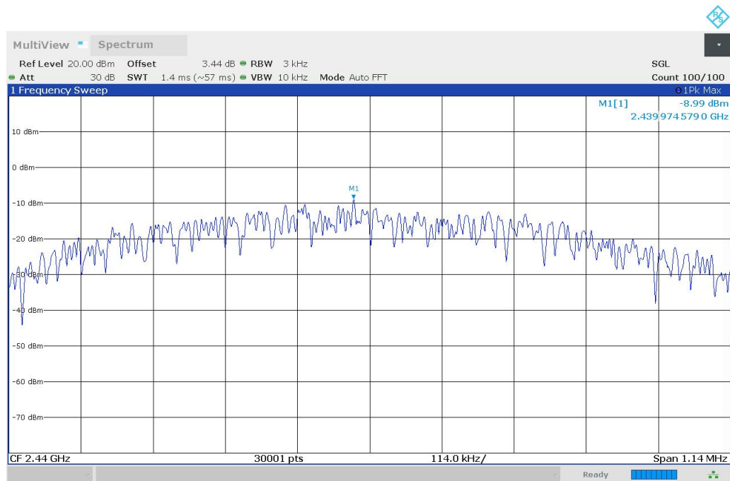
Fig.2 Power Spectral Density (CH19), LE 1M
