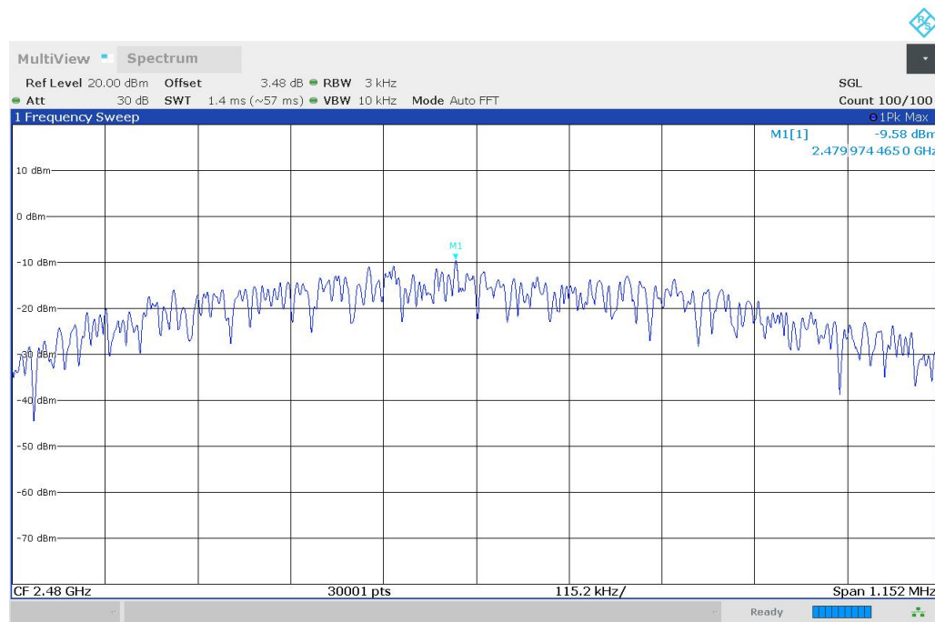
Fig.3 Power Spectral Density (CH39), LE 1M
