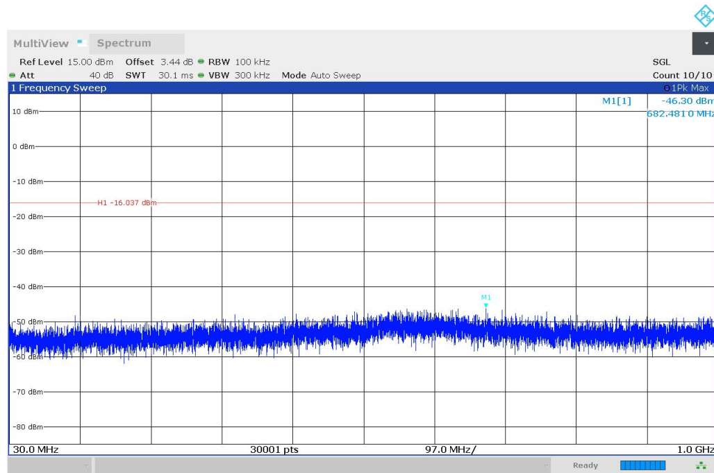
Fig.12 Conducted Spurious Emission (All Channels, 30MHz -1GHz)
