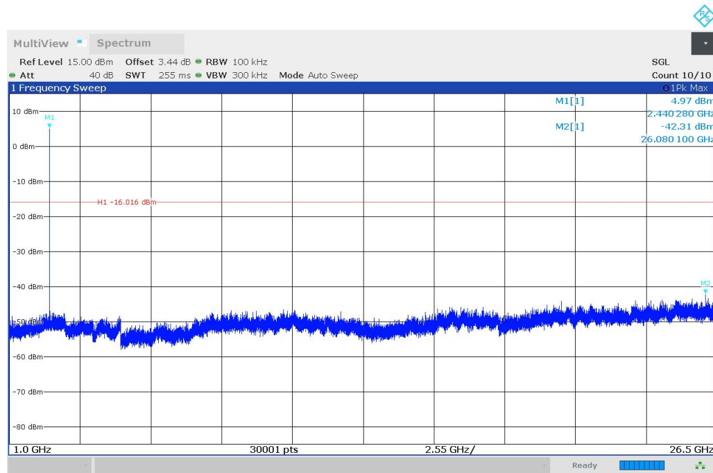
Fig.10 Conducted Spurious Emission (CH19, 1GHz-26.5GHz), LE 1M
