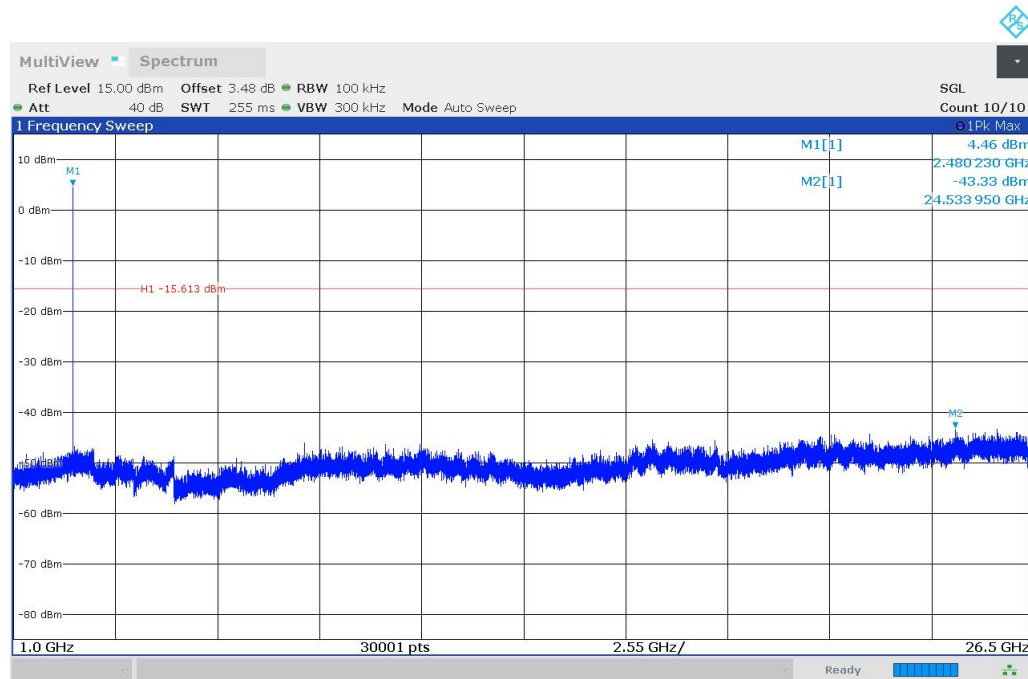
Fig.11 Conducted Spurious Emission (CH39, 1GHz-26.5GHz), LE 1M
