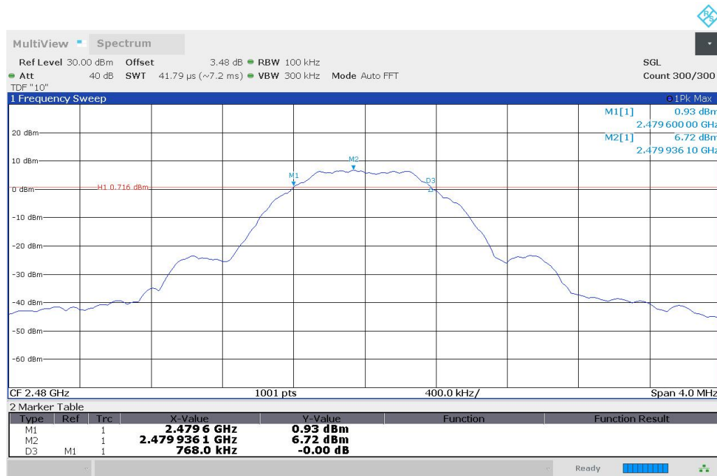
Fig.6 6dB Bandwidth (CH39), LE 1M
