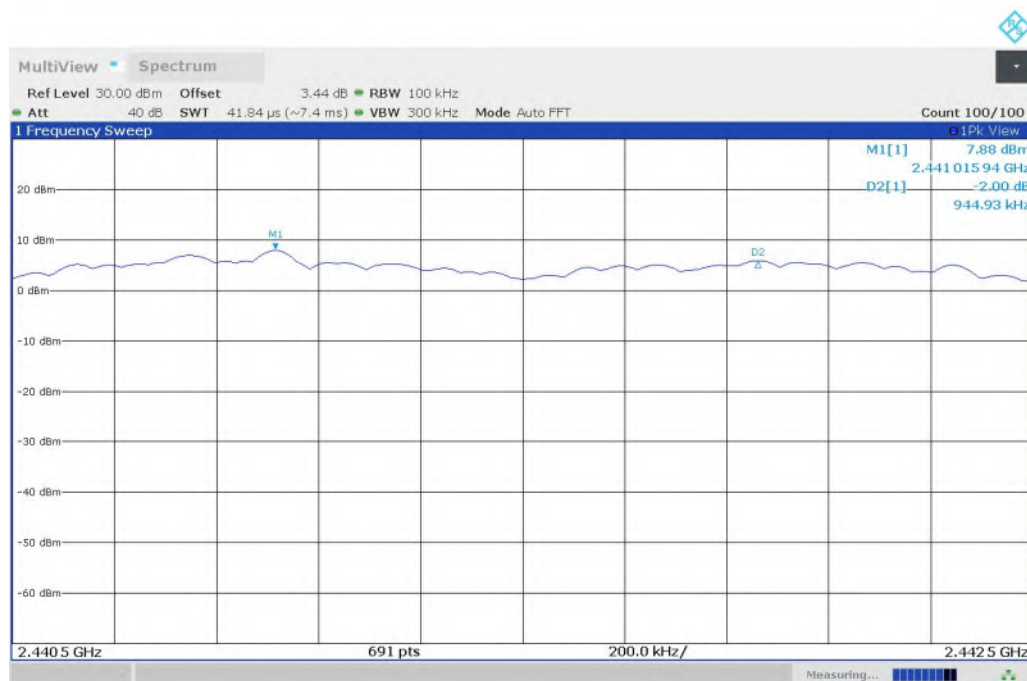
Fig. 57 Carrier Frequency Separation ( \pi/4 DQPSK, CH39)
