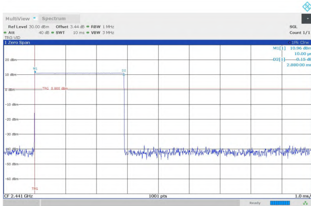
Fig. 50 BurstWidth (Dwell Time) (GFSK, CH39)
