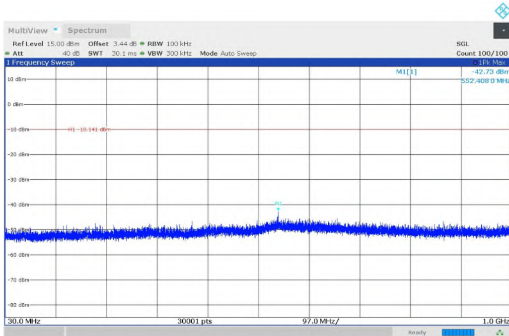
Fig. 22 Conducted Spurious Emission (All Channels, 30MHz -1GHz)
