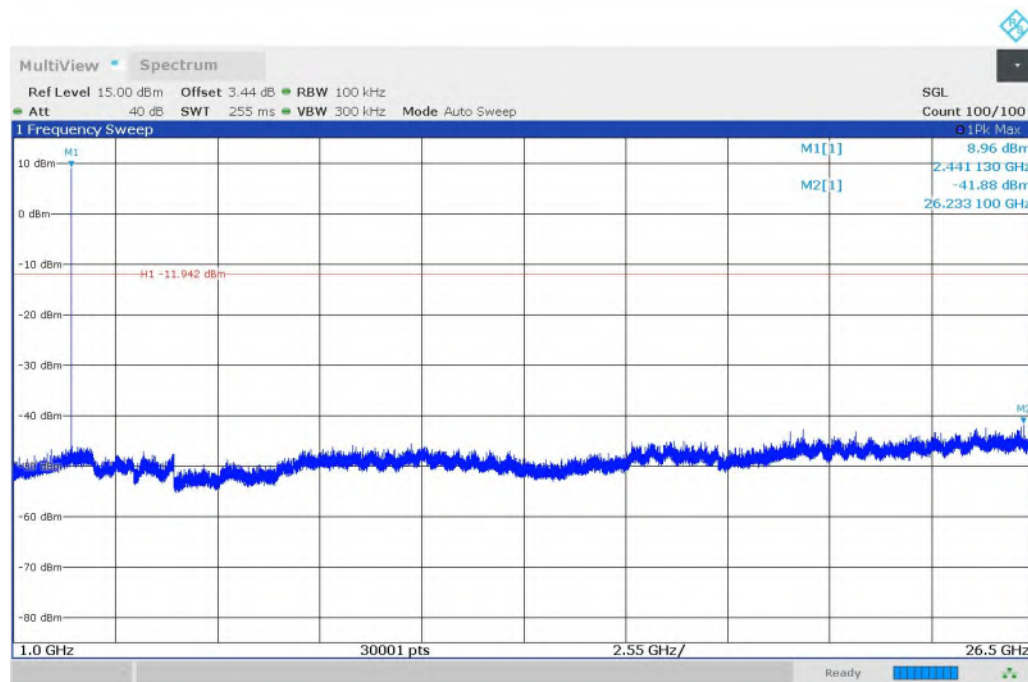
Fig. 20 Conducted Spurious Emission (8DPSK, CH39, 1GHz-26.5GHz)
