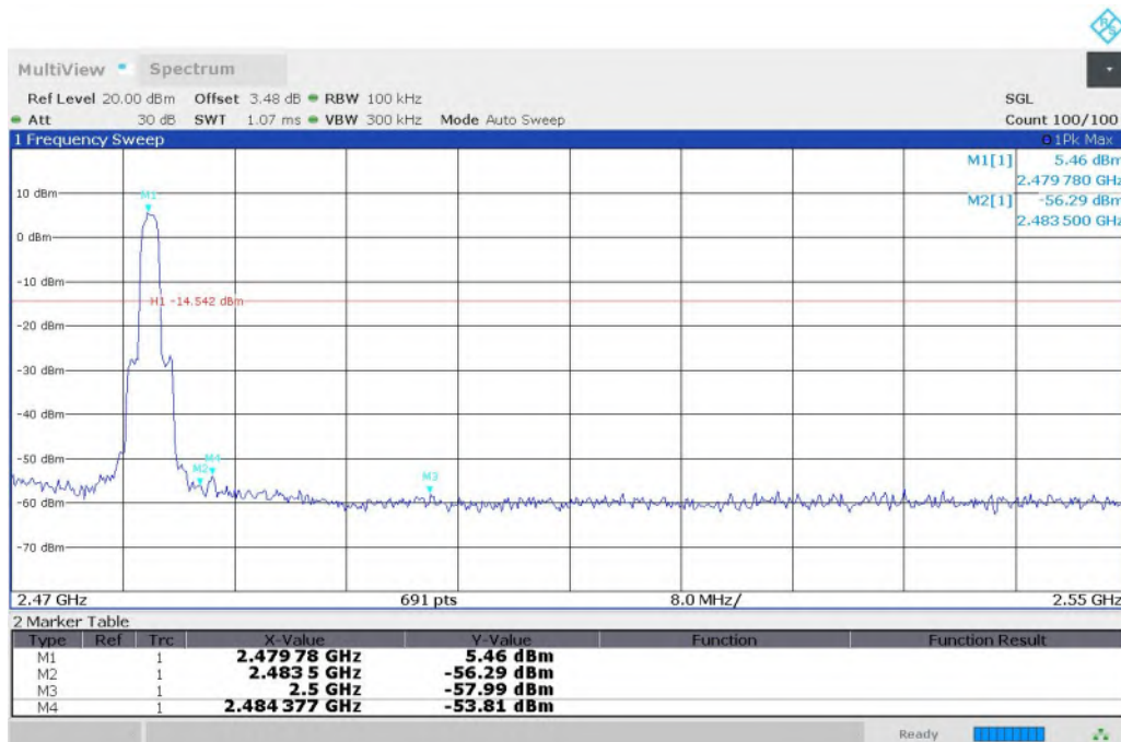
Fig. 6 Band Edges ( \pi/4 DQPSK, CH78, Hopping OFF)
