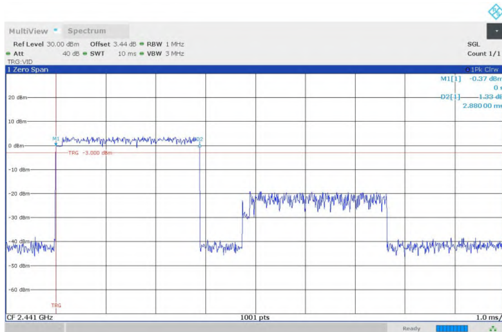
Fig. 51 BurstWidth (Dwell Time) ( \pi/4 DQPSK, CH39)
