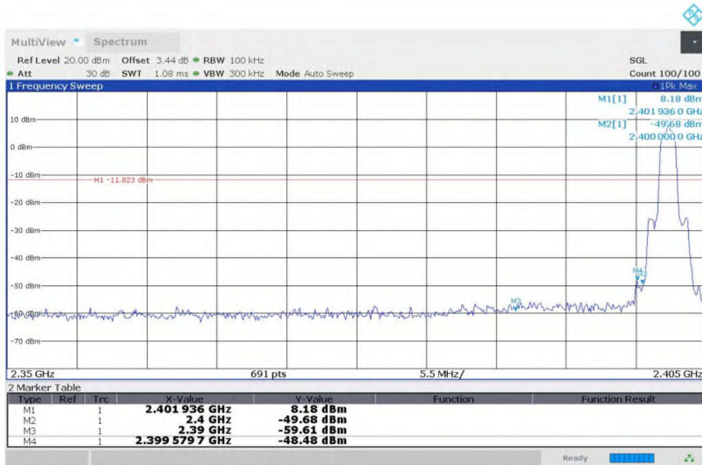
Fig. 5 Band Edges ( \pi/4 DQPSK, CH0, Hopping OFF)
