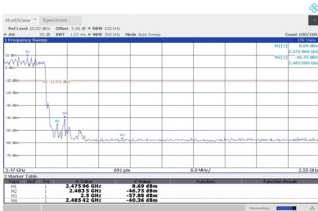
Fig. 8 Band Edges ( \pi/4 DQPSK, CH78, Hopping ON)
