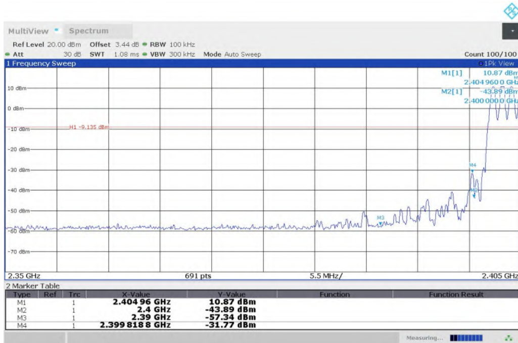
Fig. 3 Band Edges (GFSK, CH0, Hopping ON)
