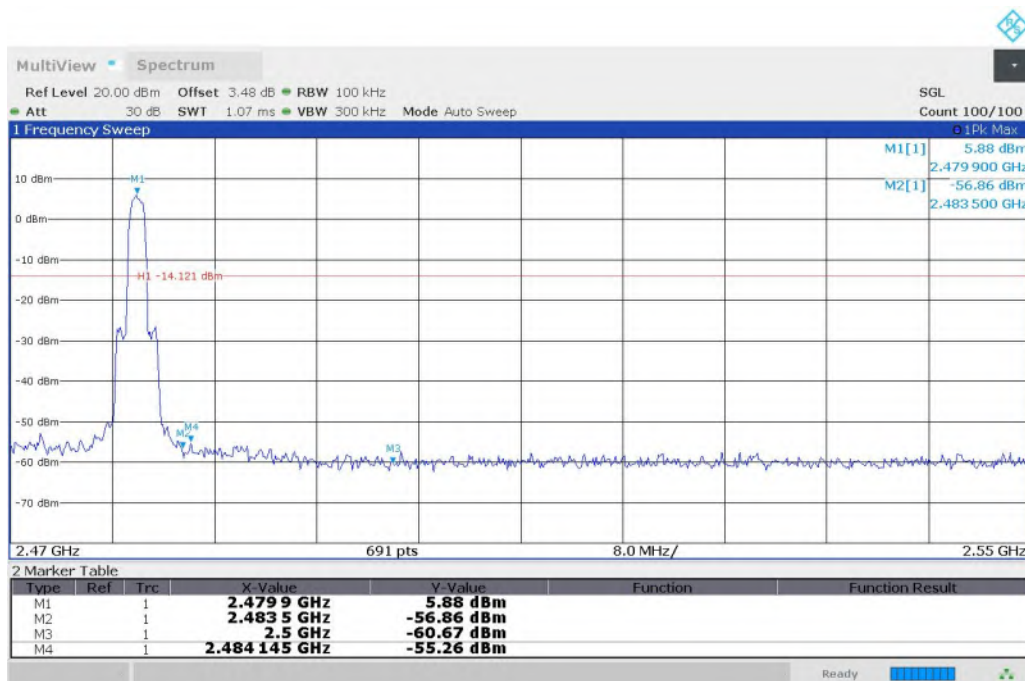
Fig. 10 Band Edges (8DPSK, CH78, Hopping OFF)
