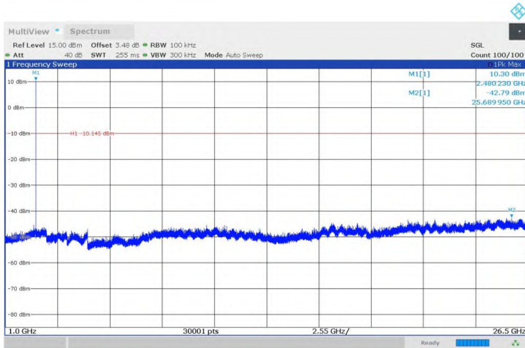
Fig. 15 Conducted Spurious Emission (GFSK, CH78, 1GHz-26.5GHz)
