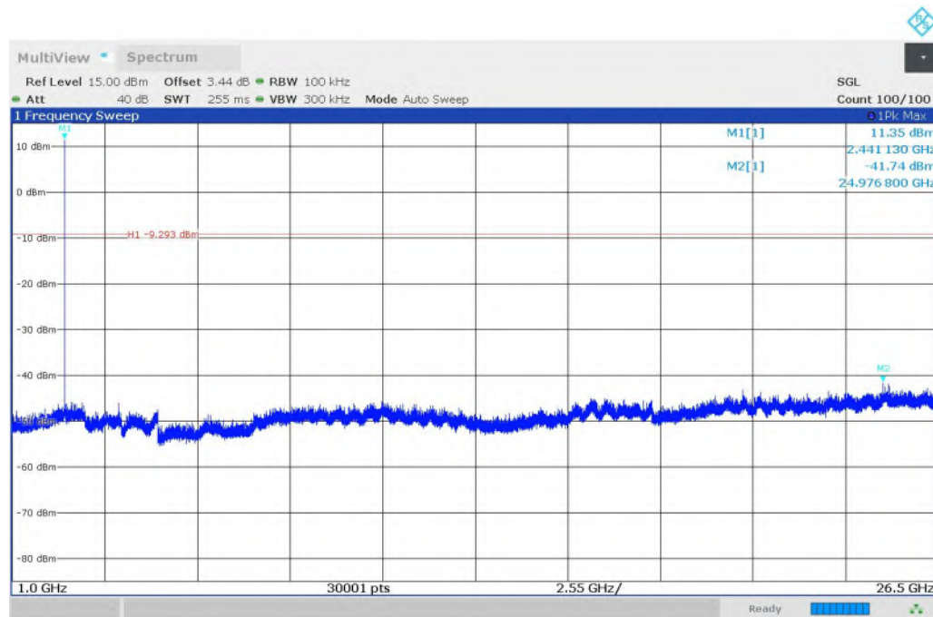
Fig. 14 Conducted Spurious Emission (GFSK, CH39, 1GHz-26.5GHz)
