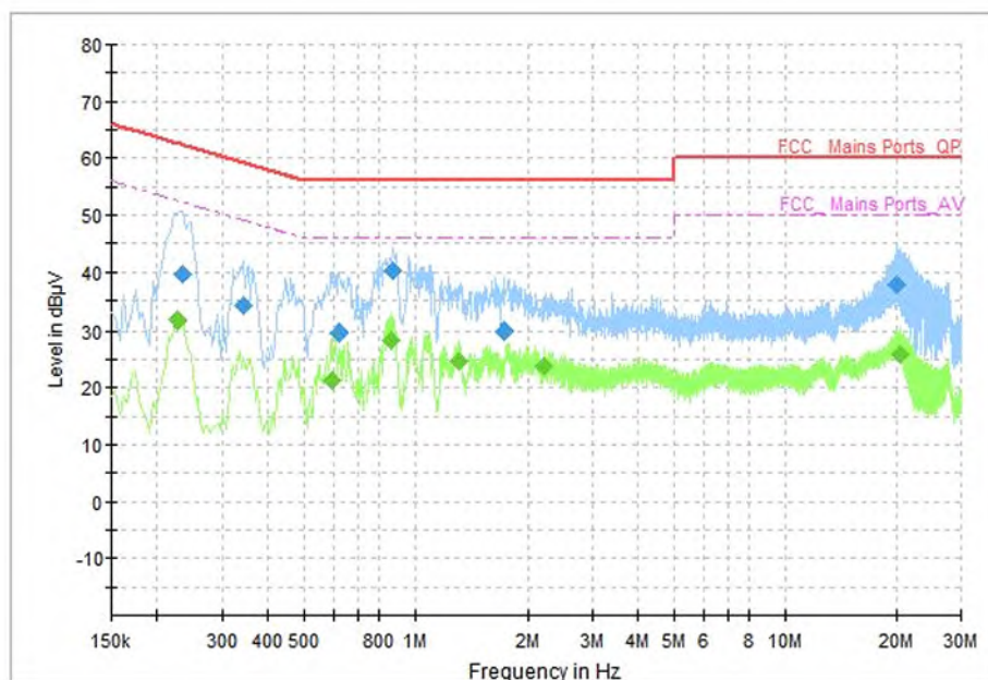
Fig. 60 AC Power line Conducted Emission (Idle)
