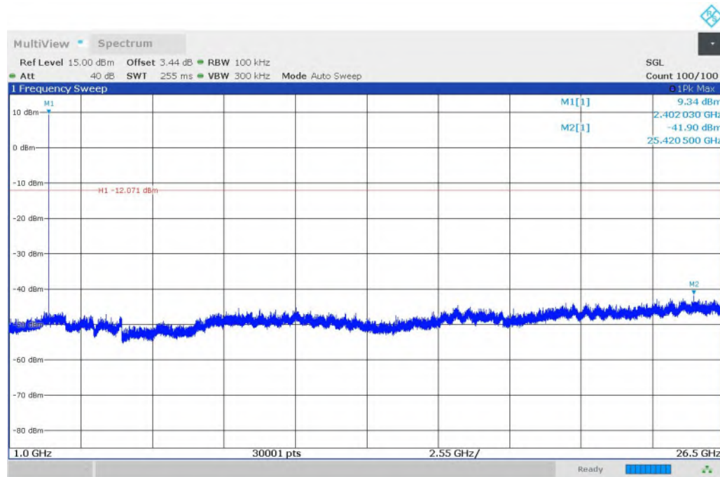
Fig. 19 Conducted Spurious Emission (8DPSK, CH0, 1GHz-26.5GHz)
