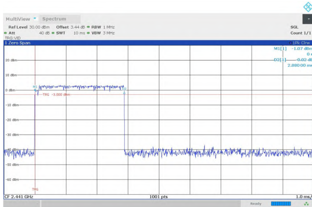
Fig. 52 BurstWidth (Dwell Time) (8DPSK, CH39)
