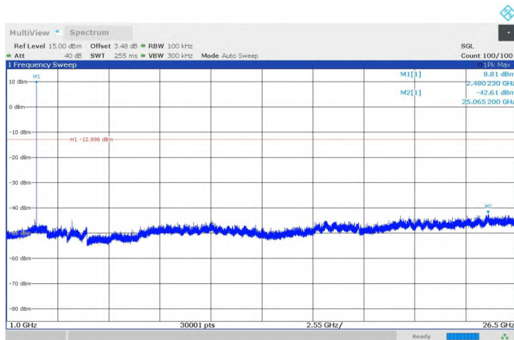
Fig. 18 Conducted Spurious Emission ( \pi/4 DQPSK, CH78, 1GHz-26.5GHz)
