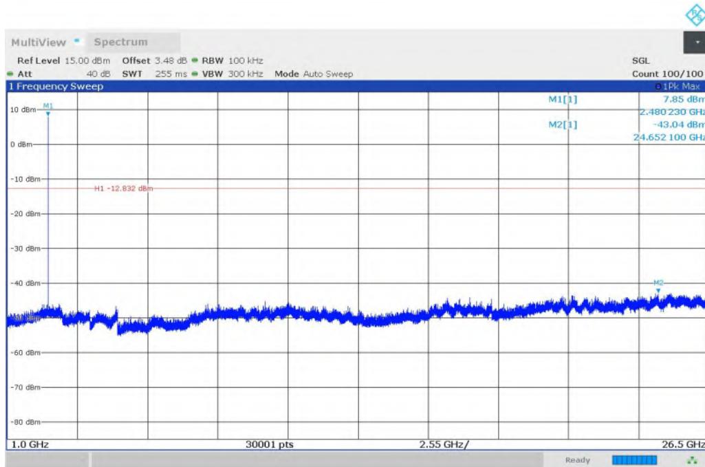
Fig. 21 Conducted Spurious Emission (8DPSK, CH78, 1GHz-26.5GHz)
