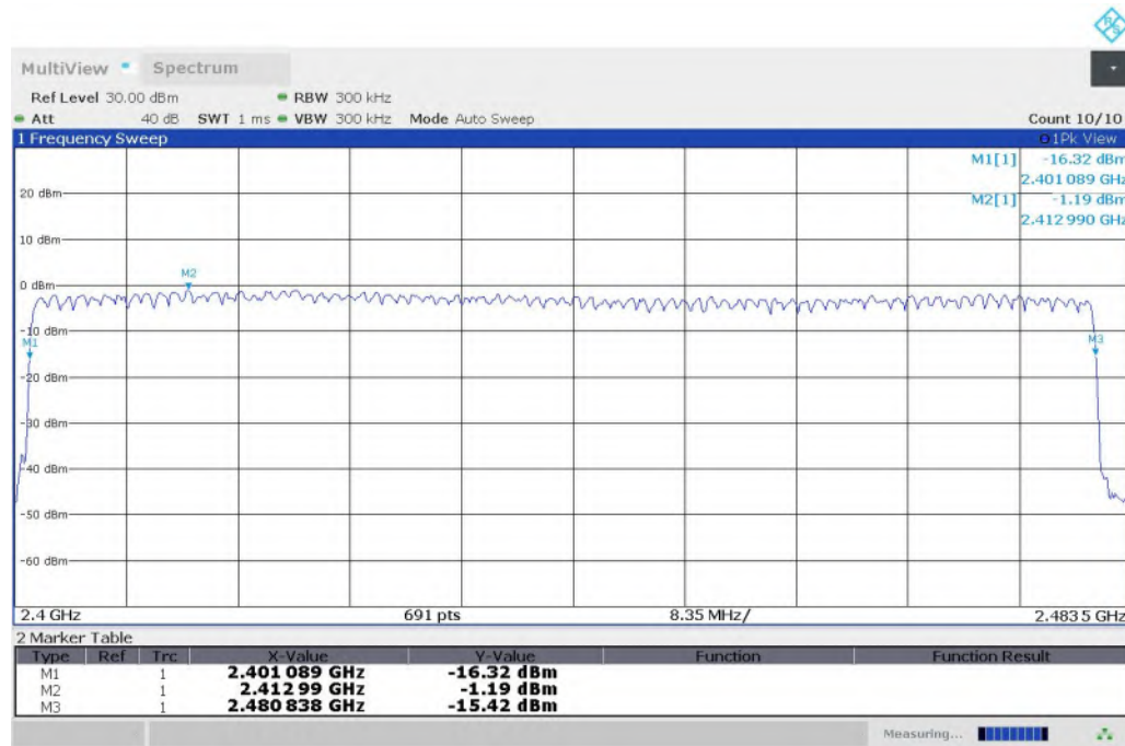
Fig. 55 Number of Hopping Channels (8DPSK, Hopping)
