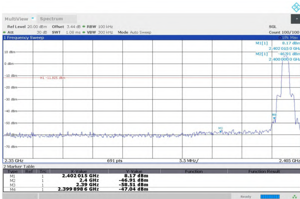
Fig. 9 Band Edges (8DPSK, CH0, Hopping OFF)
