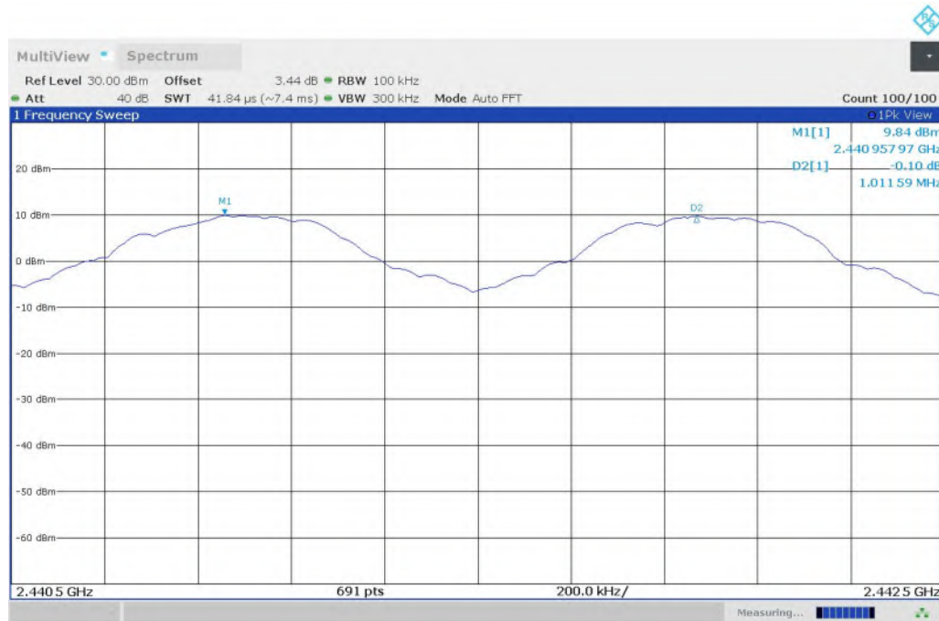
Fig. 56 Carrier Frequency Separation (GFSK, CH39)
