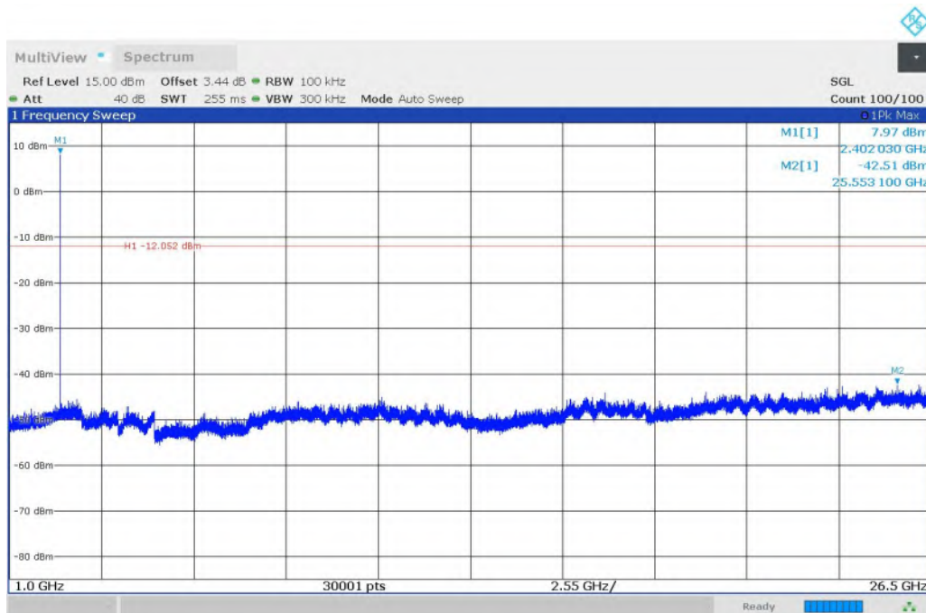
Fig. 16 Conducted Spurious Emission ( \pi/4 DQPSK, CH0, 1GHz-26.5GHz)
