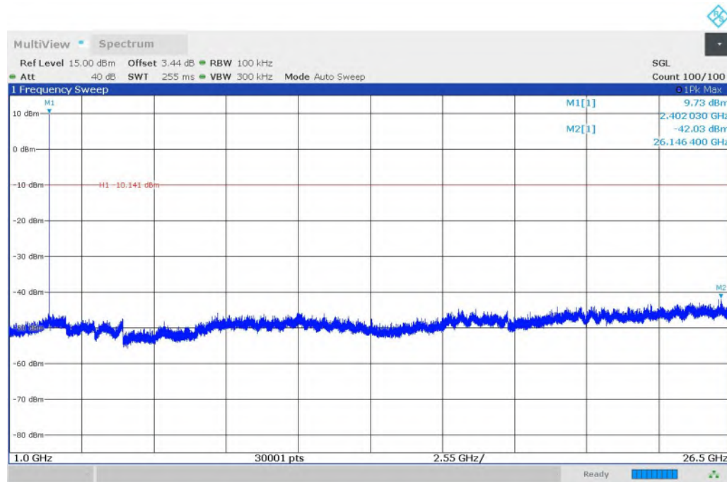
Fig. 13 Conducted Spurious Emission (GFSK, CH0, 1GHz-26.5GHz)
