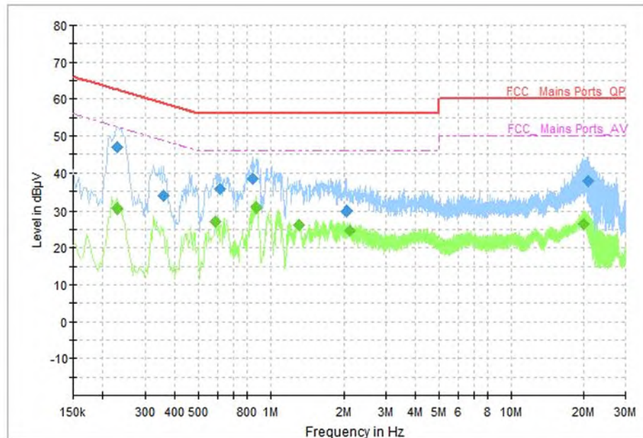
Fig. 59 AC Power line Conducted Emission (Traffic)
