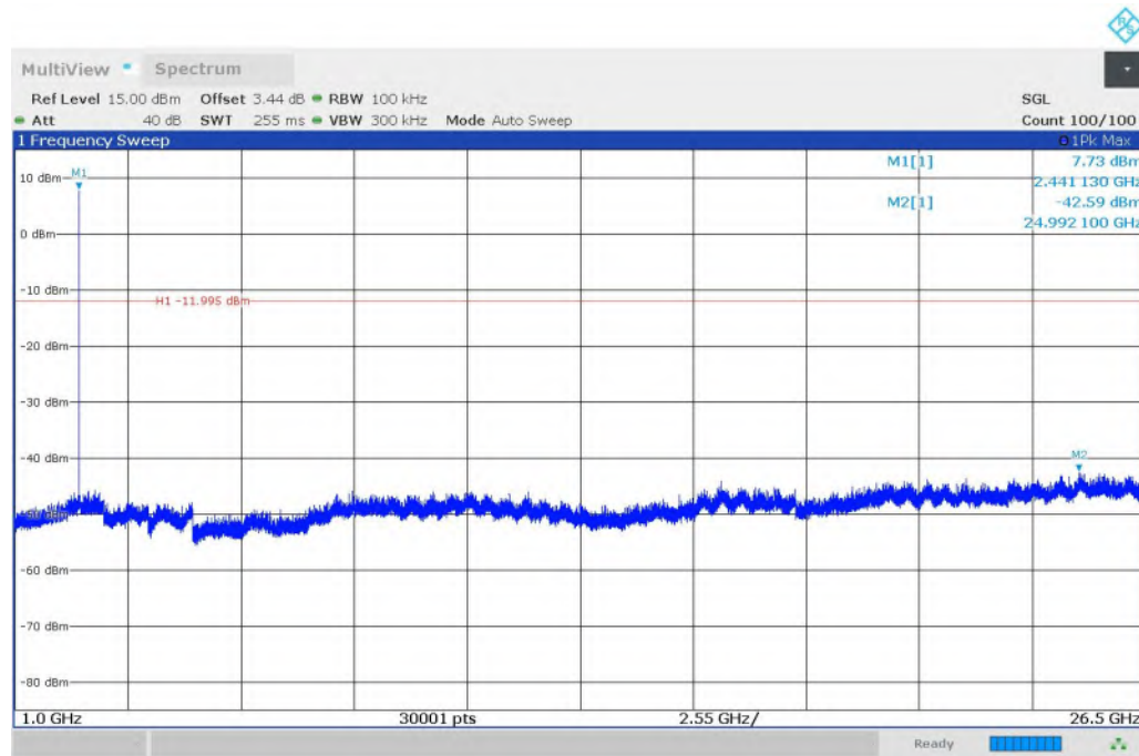
Fig. 17 Conducted Spurious Emission ( \pi/4 DQPSK, CH39, 1GHz-26.5GHz)
