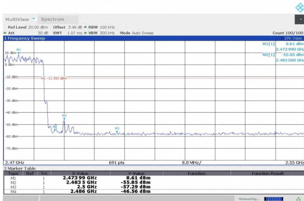
Fig. 12 Band Edges (8DPSK, CH78, Hopping ON)
