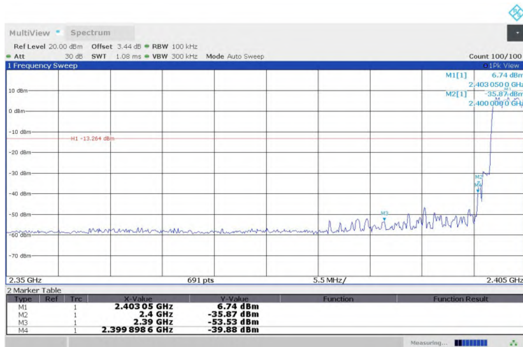
Fig. 11 Band Edges (8DPSK, CH0, Hopping ON)
