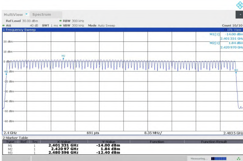
Fig. 53 Number of Hopping Channels (GFSK, Hopping)
