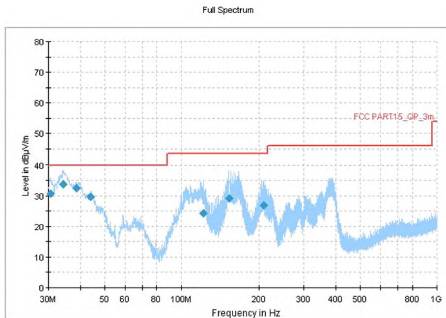
Fig. 39 Radiated Spurious Emission (All Channels, 30MHz ~1GHz)
