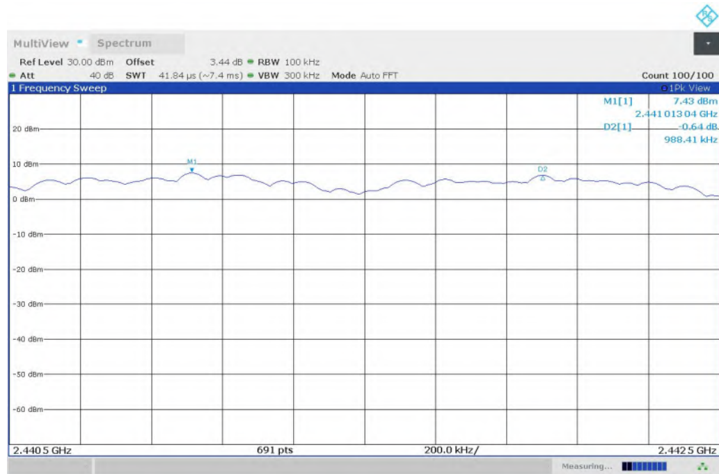
Fig. 58 Carrier Frequency Separation (8DPSK, CH39)
