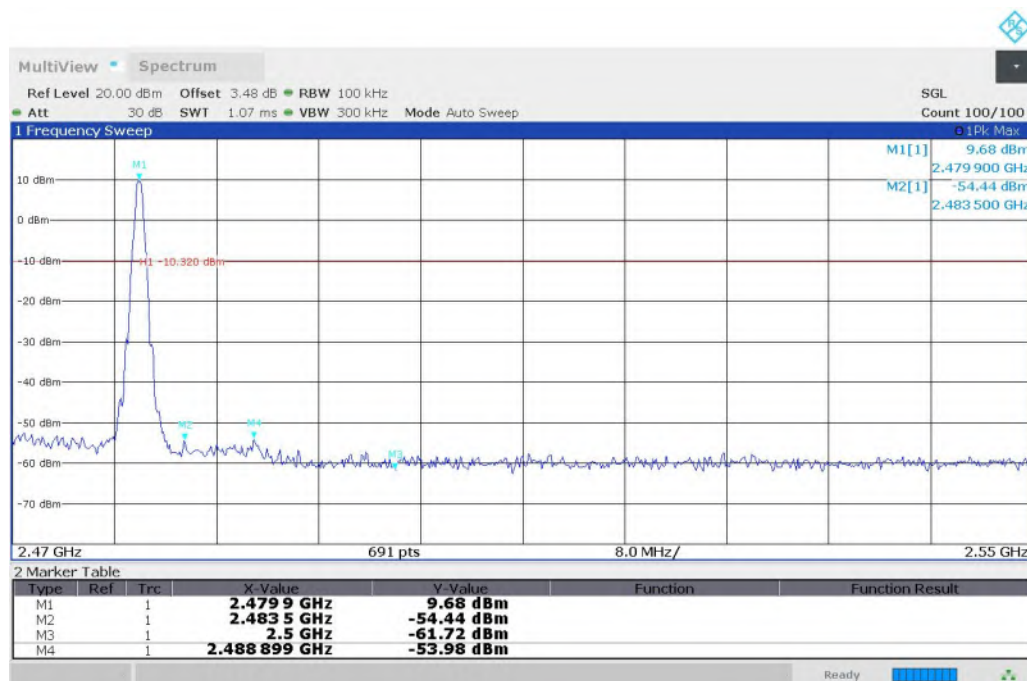
Fig. 2 Band Edges (GFSK, CH78, Hopping OFF)
