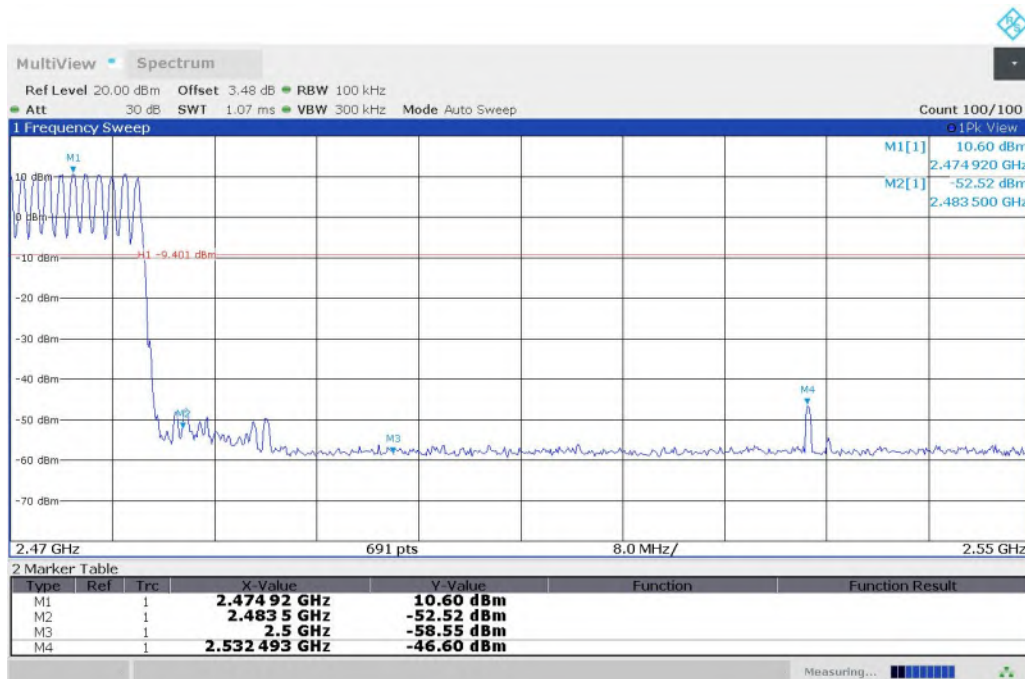
Fig. 4 Band Edges (GFSK, CH78, Hopping ON)
