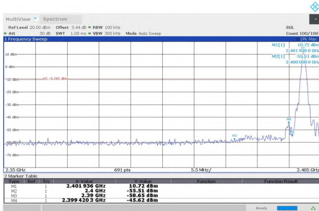
Fig. 1 Band Edges (GFSK, CH0, Hopping OFF)
