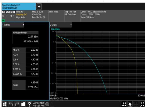
B2_N7(20M)_DFT-s-OFDM_PI_2- BPSK_Outer_Full_Mid_CH
