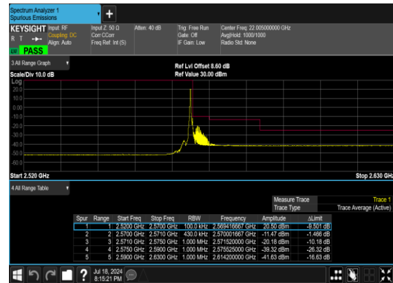
B2_N7(20M)_DFT-s- OFDM_BPSK_Edge_1RB_Right_High_CH
