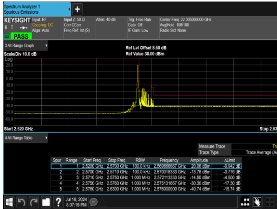
B2_N7(5M)_DFT-s- OFDM_BPSK_Edge_1RB_Right_High_CH
