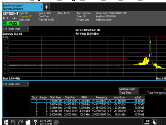
B2_N7(20M)_DFT-s- OFDM_QPSK_Edge_1RB_Left_Low_CH
