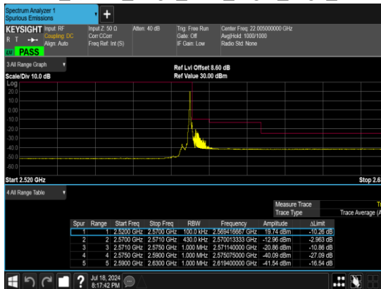
B2_N7(20M)_DFT-s- OFDM_QPSK_Edge_1RB_Right_High_CH
