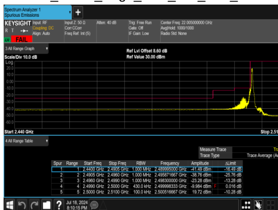
B2_N7(20M)_DFT-s- OFDM_BPSK_Edge_1RB_Left_Low_CH
