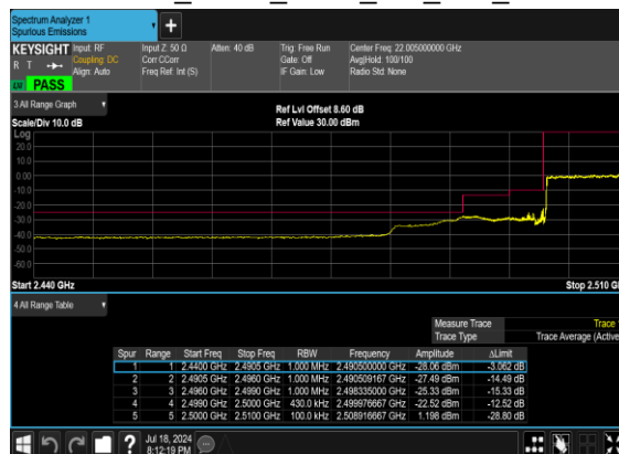
B2_N7(20M)_DFT-s- OFDM_BPSK_Outer_Full_Low_CH
