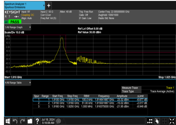
B12_N25(5M)_DFT-s- OFDM_QPSK_Edge_1RB_Right_High_CH
