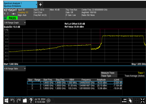
B12_N25(5M)_DFT-s- OFDM_QPSK_Outer_Full_Low_CH
