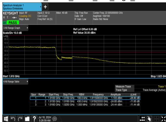
B12_N25(40M)_DFT-s- OFDM_BPSK_Outer_Full_High_CH
