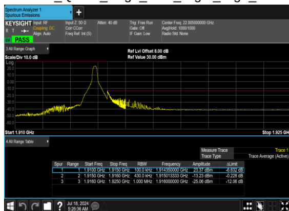
B12_N25(40M)_DFT-s- OFDM_QPSK_Edge_1RB_Right_High_CH
