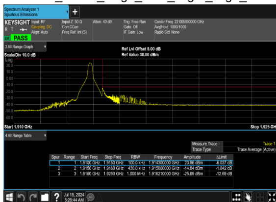
B12_N25(40M)_DFT-s- OFDM_BPSK_Edge_1RB_Right_High_CH
