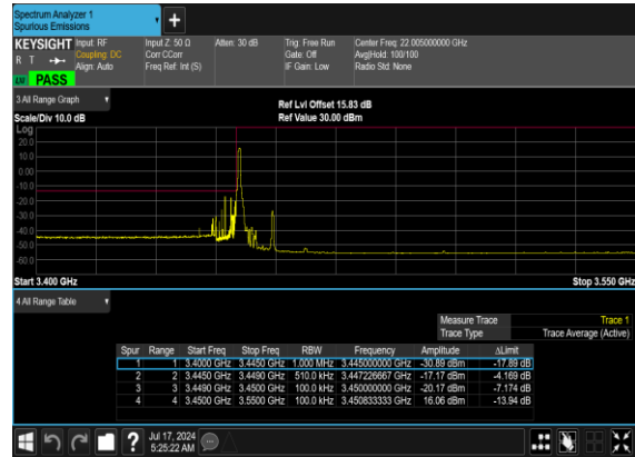
B2_N77(10M)_DFT-s- OFDM_QPSK_Edge_1RB_Left_Low_CH
