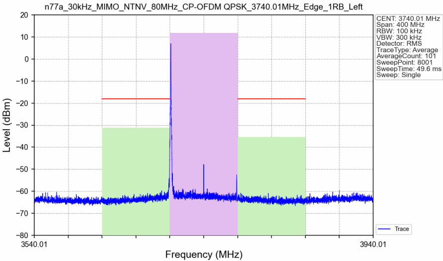
n77a_30kHz_MIMO_NTNV_80MHz_CP-OFDM QPSK_3740.01MHz_Edge_1RB_Left_Ant3
