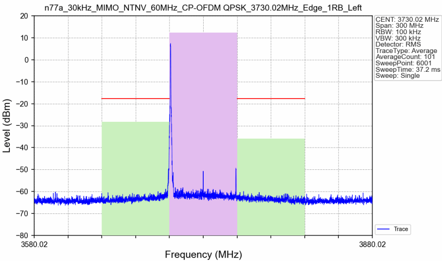
n77a_30kHz_MIMO_NTNV_60MHz_CP-OFDM QPSK_3730.02MHz_Edge_1RB_Left_Ant3
