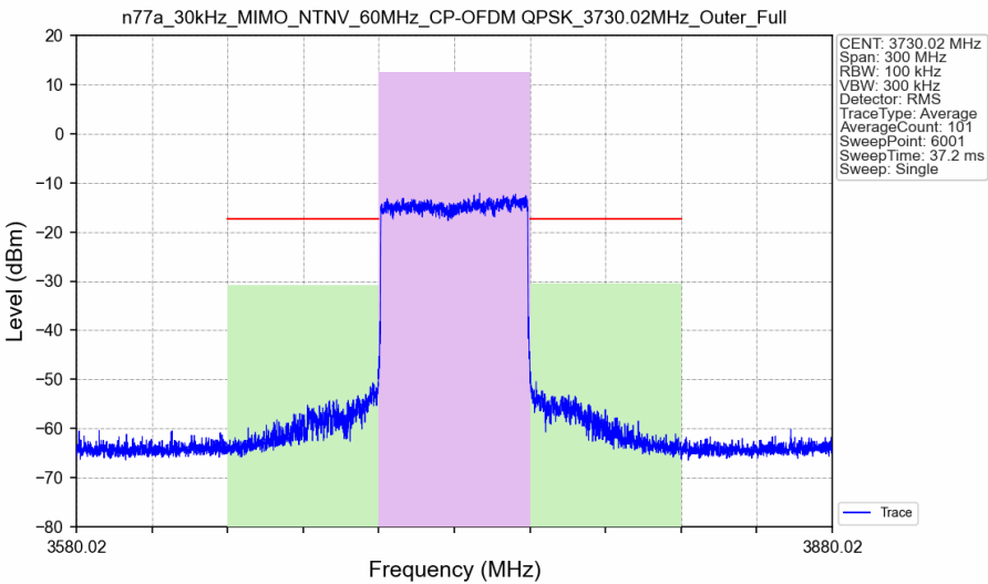
n77a_30kHz_MIMO_NTNV_60MHz_CP-OFDM QPSK_3730.02MHz_Outer_Full_Ant3
