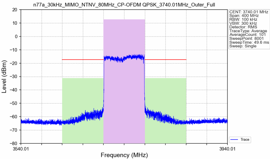
n77a_30kHz_MIMO_NTNV_80MHz_CP-OFDM QPSK_3740.01MHz_Outer_Full_Ant3
