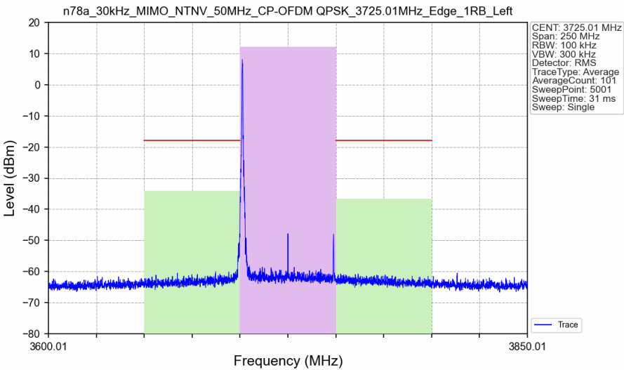
n78a_30kHz_MIMO_NTNV_50MHz_CP-OFDM QPSK_3725.01MHz_Edge_1RB_Left_Ant3
