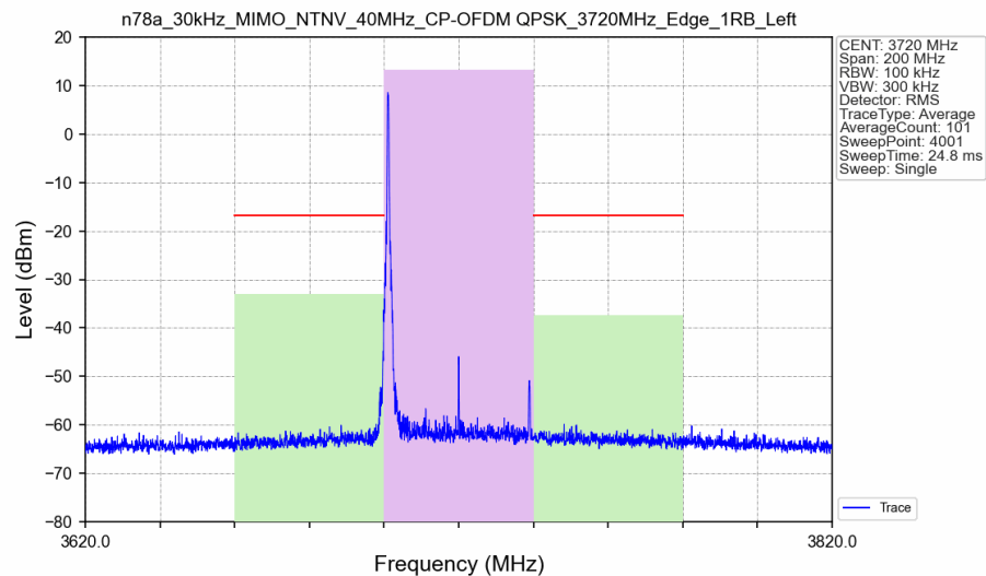
n78a_30kHz_MIMO_NTNV_40MHz_CP-OFDM QPSK_3720MHz_Edge_1RB_Left_Ant3
