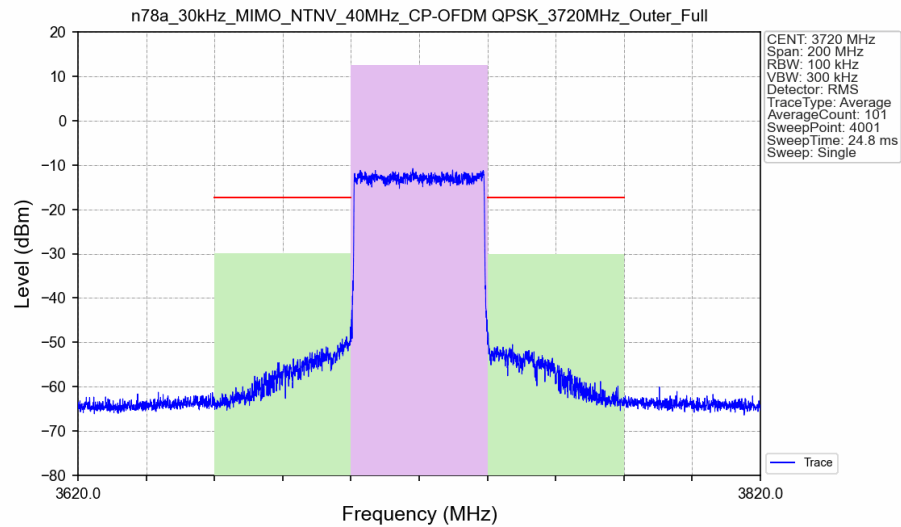
n78a_30kHz_MIMO_NTNV_40MHz_CP-OFDM QPSK_3720MHz_Outer_Full_Ant3
