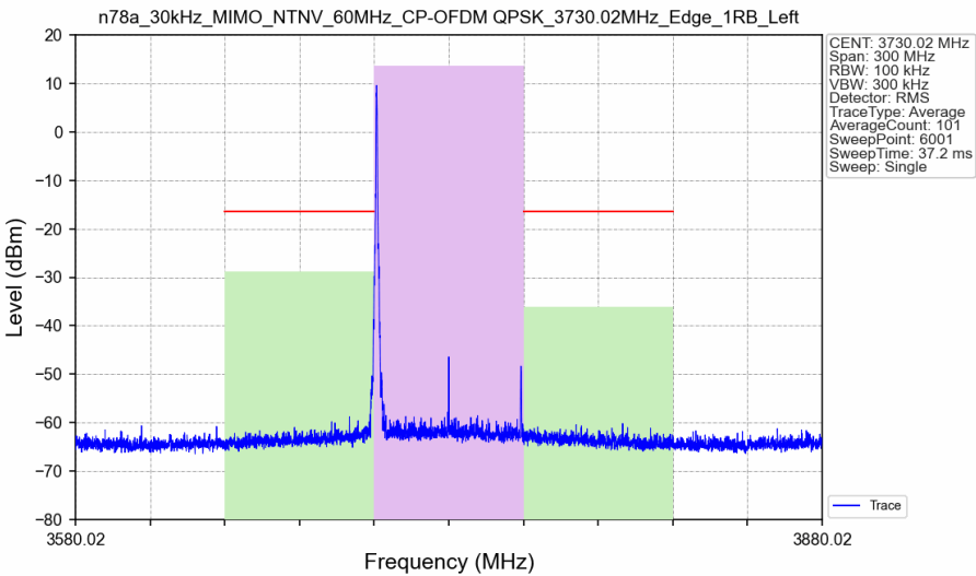
n78a_30kHz_MIMO_NTNV_60MHz_CP-OFDM QPSK_3730.02MHz_Edge_1RB_Left_Ant3
