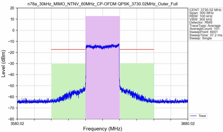
n78a_30kHz_MIMO_NTNV_60MHz_CP-OFDM QPSK_3730.02MHz_Outer_Full_Ant3
