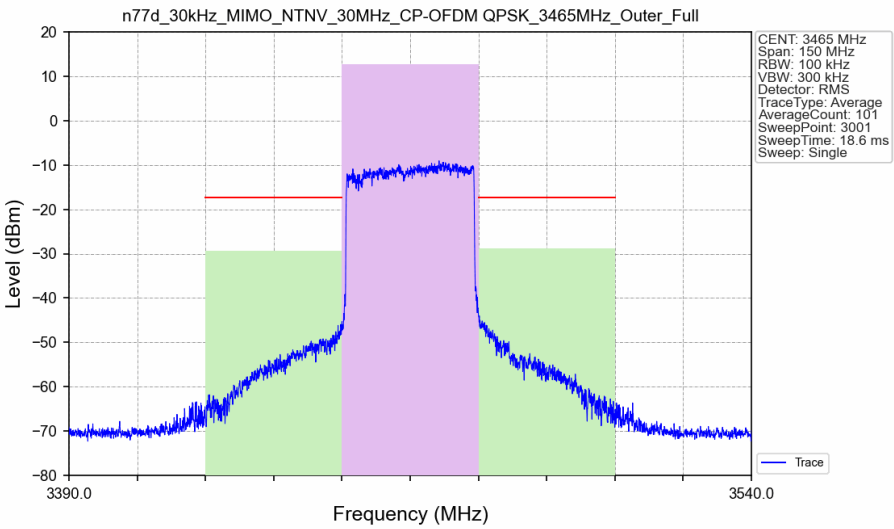
n77d_30kHz_MIMO_NTNV_30MHz_CP-OFDM QPSK_3465MHz_Outer_Full_Ant3
