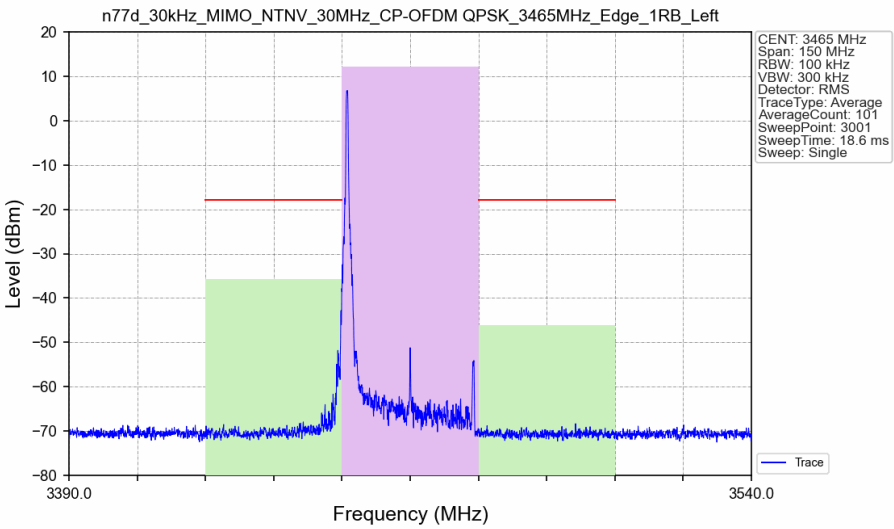
n77d_30kHz_MIMO_NTNV_30MHz_CP-OFDM QPSK_3465MHz_Edge_1RB_Left_Ant3
