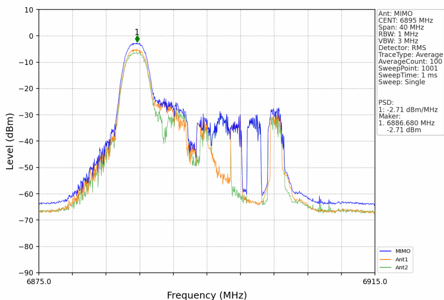
802.11ax(HEW20)_LCH_6895MHz_RU52_Left_MIMO_NTNV
