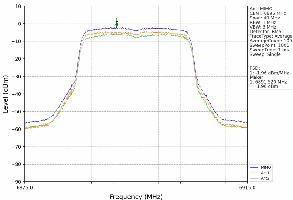
802.11ax(HEW20)_LCH_6895MHz_SU_MIMO_NTNV
