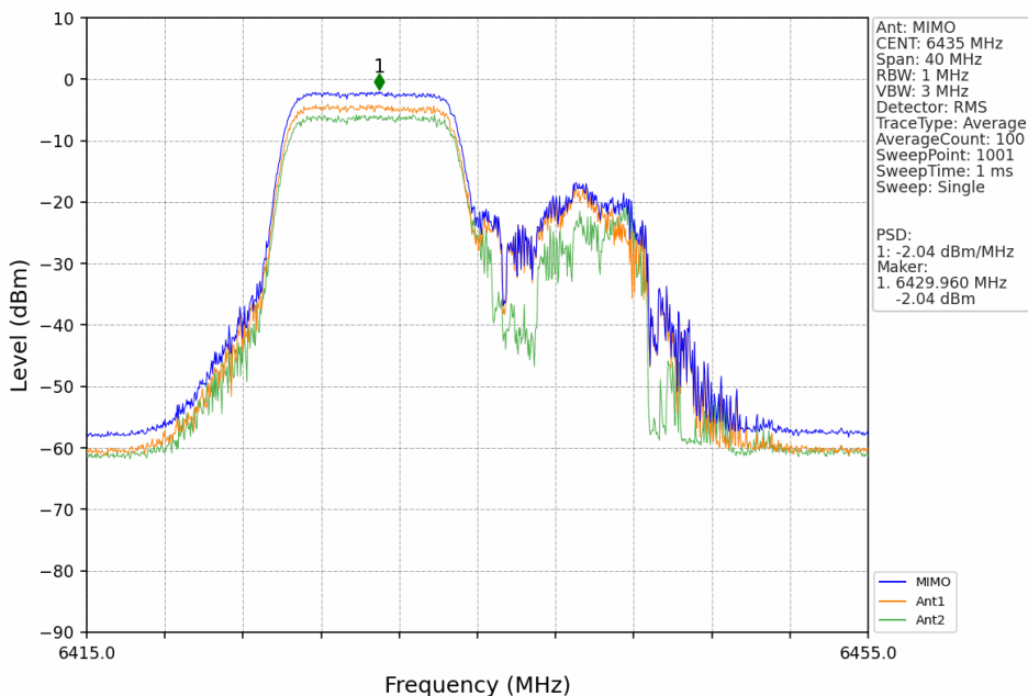
802.11ax(HEW20)_LCH_6435MHz_SU_MIMO_NTNV
