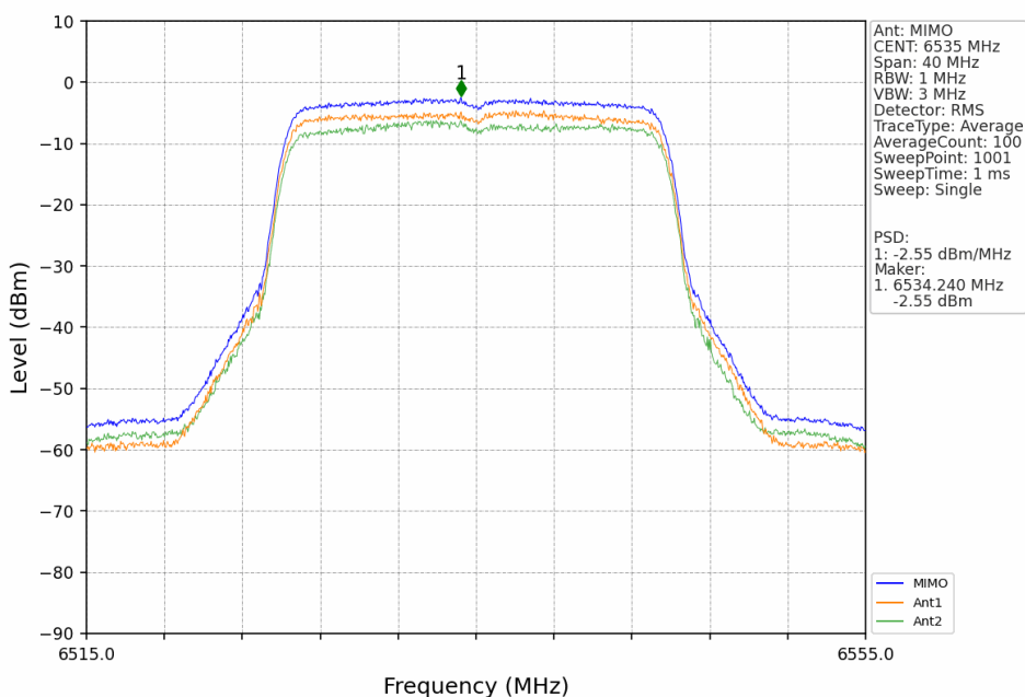
802.11ax(HEW20)_LCH_6535MHz_SU_MIMO_NTNV
