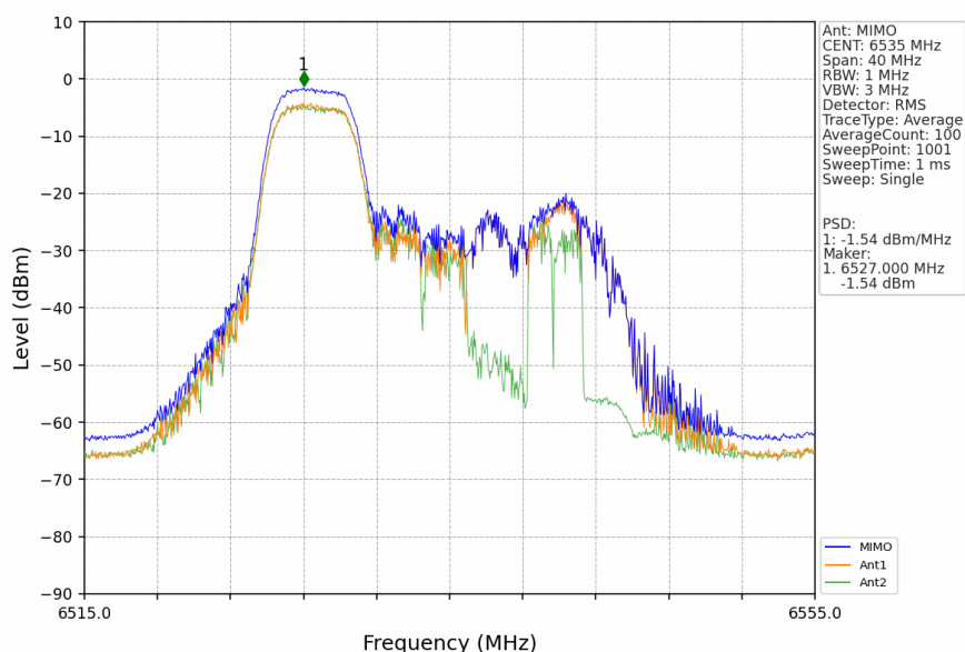
802.11ax(HEW20)_LCH_6535MHz_RU52_Left_MIMO_NTNV
