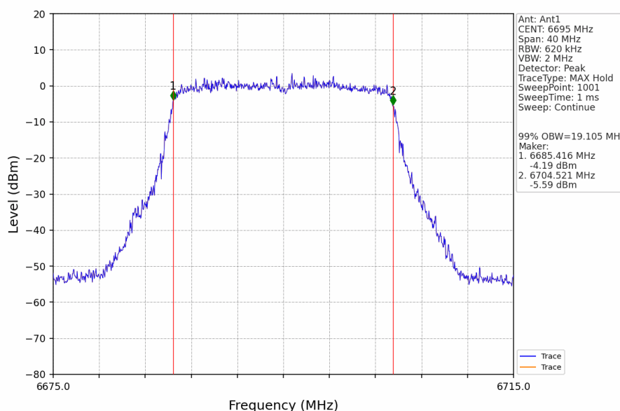
802.11ax(HEW20)_MCH_6695MHz_SU_Ant1_NTNV
