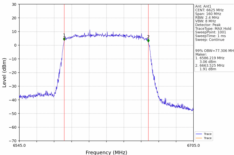
802.11ax(HEW80)_LCH_6625MHz_SU_Ant1_NTNV
