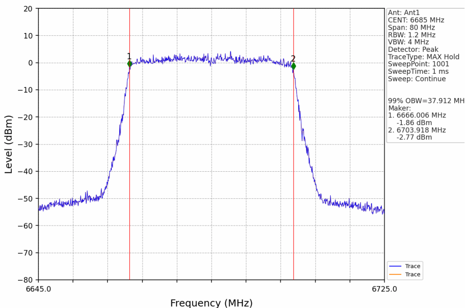
802.11ax(HEW40)_MCH_6685MHz_SU_Ant1_NTNV
