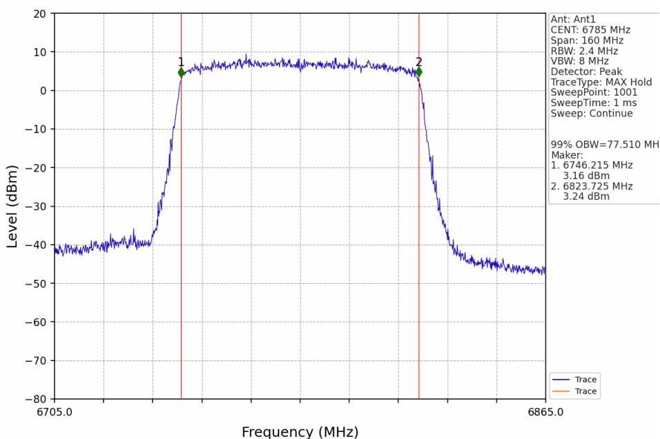
802.11ax(HEW80)_HCH_6785MHz_SU_Ant1_NTNV
