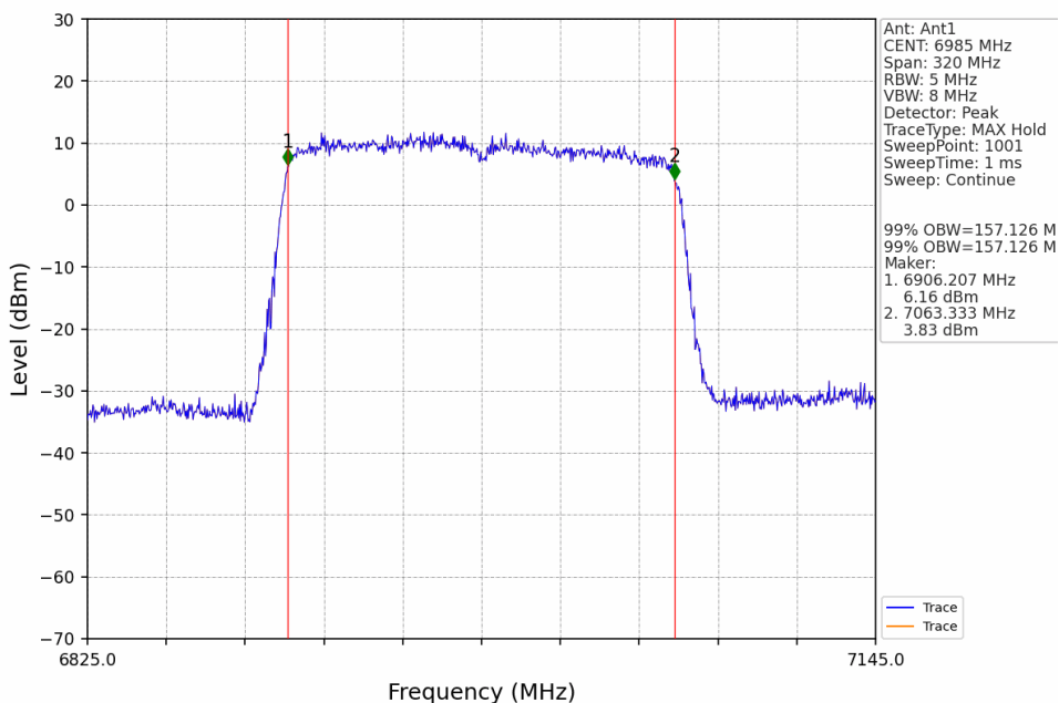
802.11ax(HEW160)_MCH_6985MHz_SU_Ant1_NTNV
