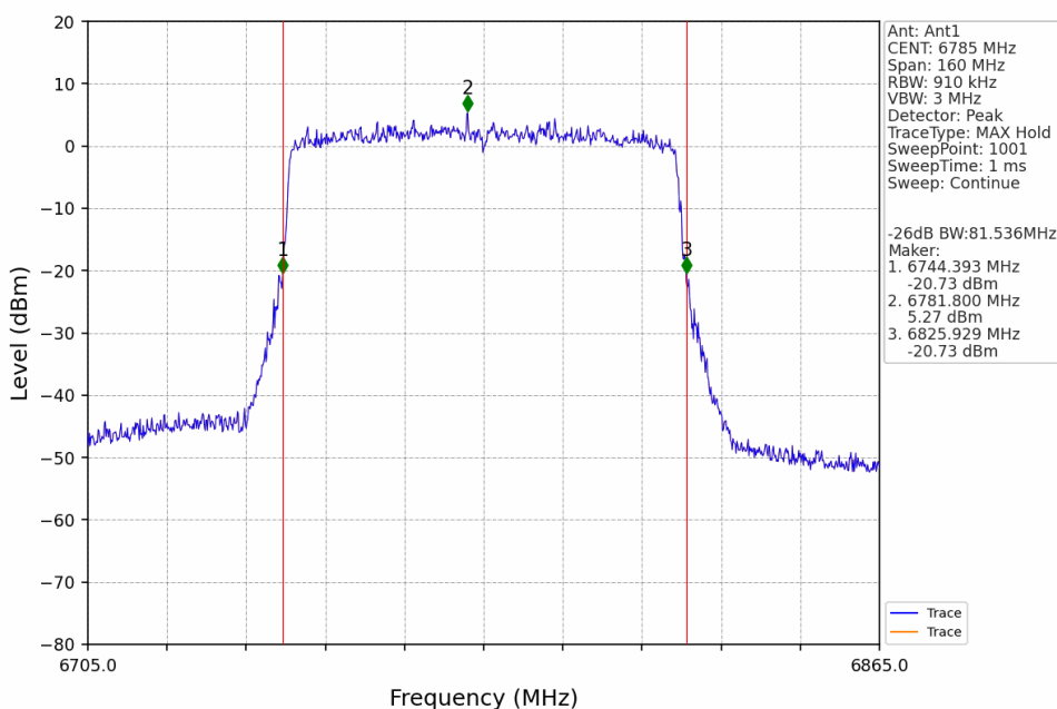
802.11ax(HEW80)_HCH_6785MHz_SU_Ant1_NTNV
