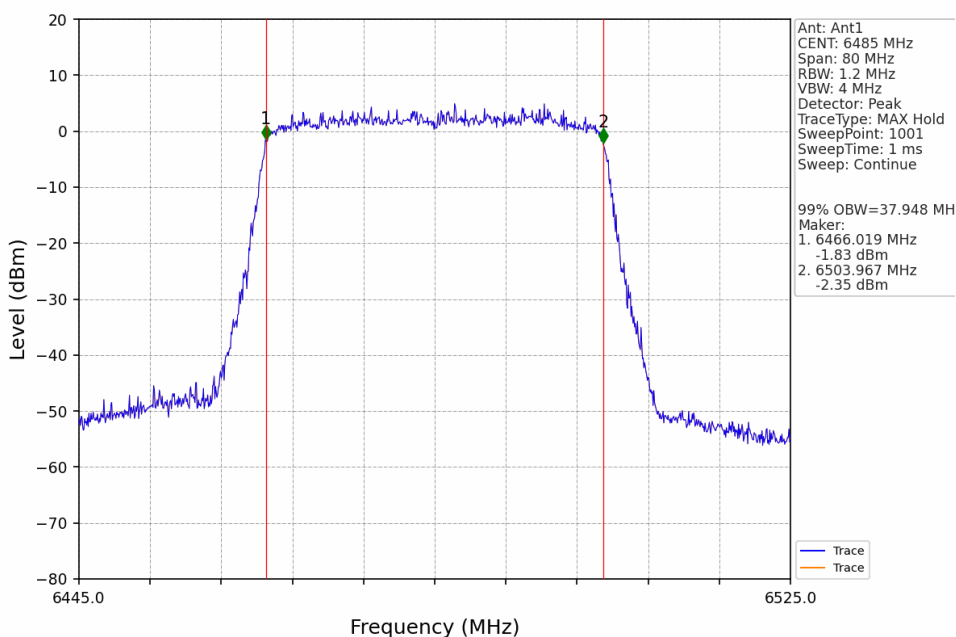
802.11ax(HEW40)_MCH_6485MHz_SU_Ant1_NTNV
