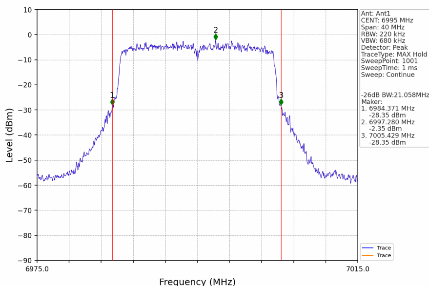
802.11ax(HEW20)_MCH_6995MHz_SU_Ant1_NTNV
