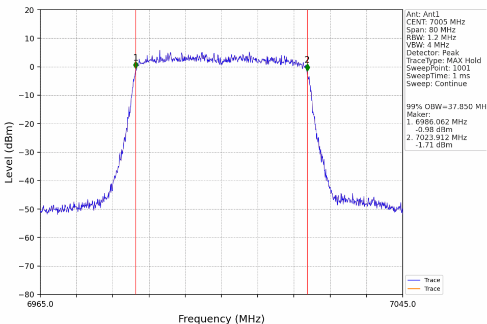
802.11ax(HEW40)_MCH_7005MHz_SU_Ant1_NTNV
