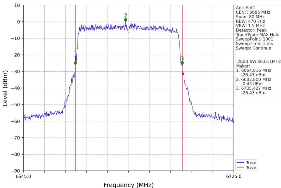
802.11ax(HEW40)_MCH_6685MHz_SU_Ant1_NTNV
