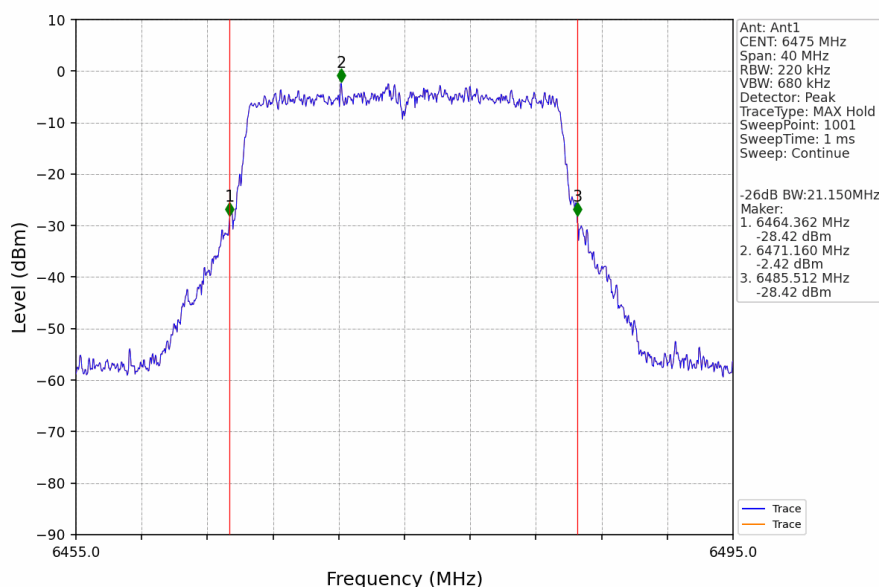
802.11ax(HEW20)_MCH_6475MHz_SU_Ant1_NTNV
