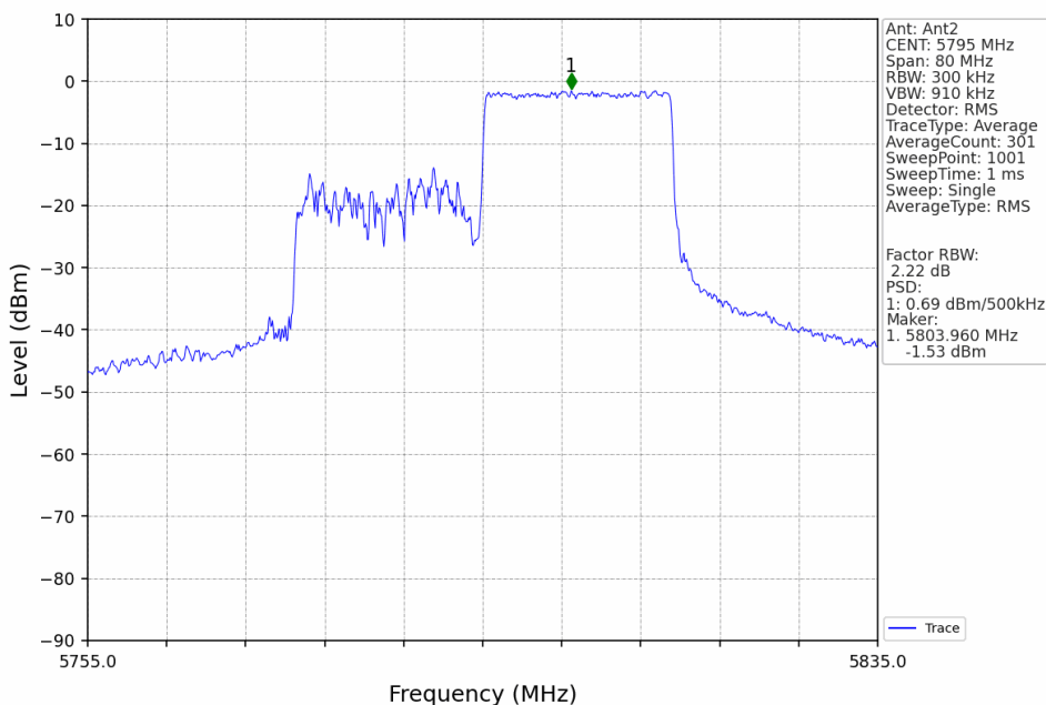
802.11ax(HEW40)_HCH_5795MHz_RU242_Right_Ant2_NTNV
