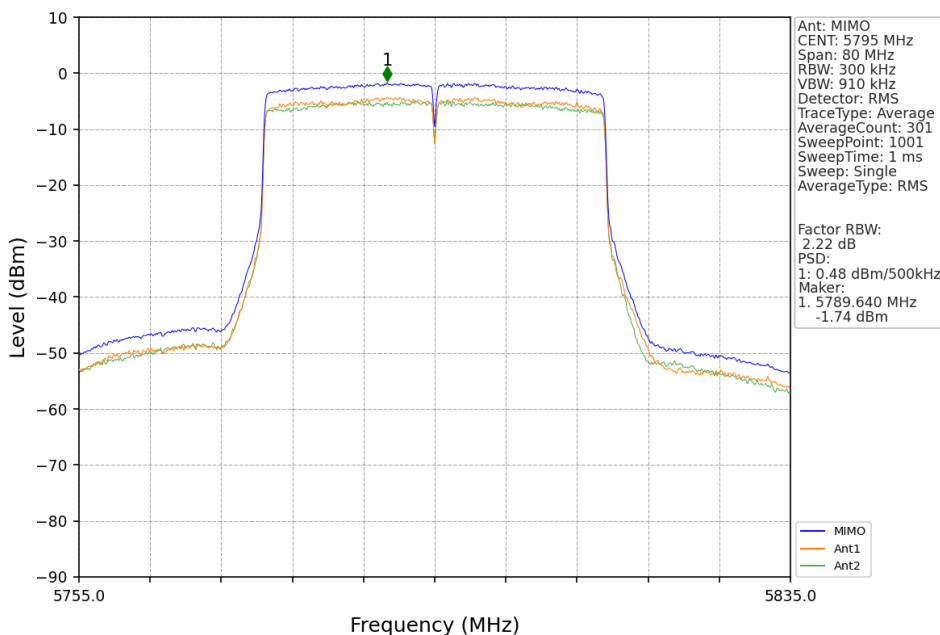
802.11ax(HEW40)_HCH_5795MHz_SU_MIMO_NTNV
