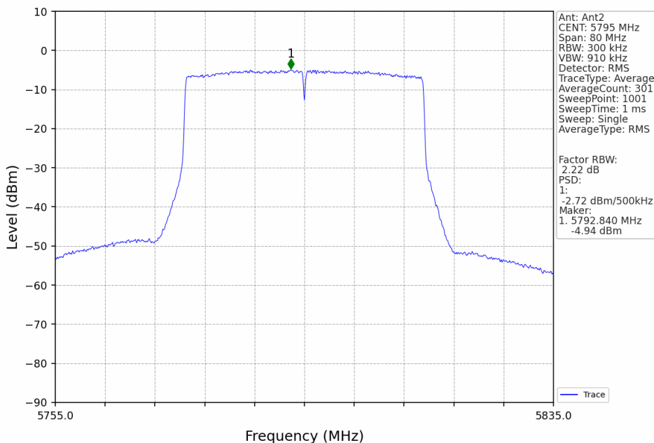
802.11ax(HEW40)_HCH_5795MHz_SU_MIMO_NTNV
