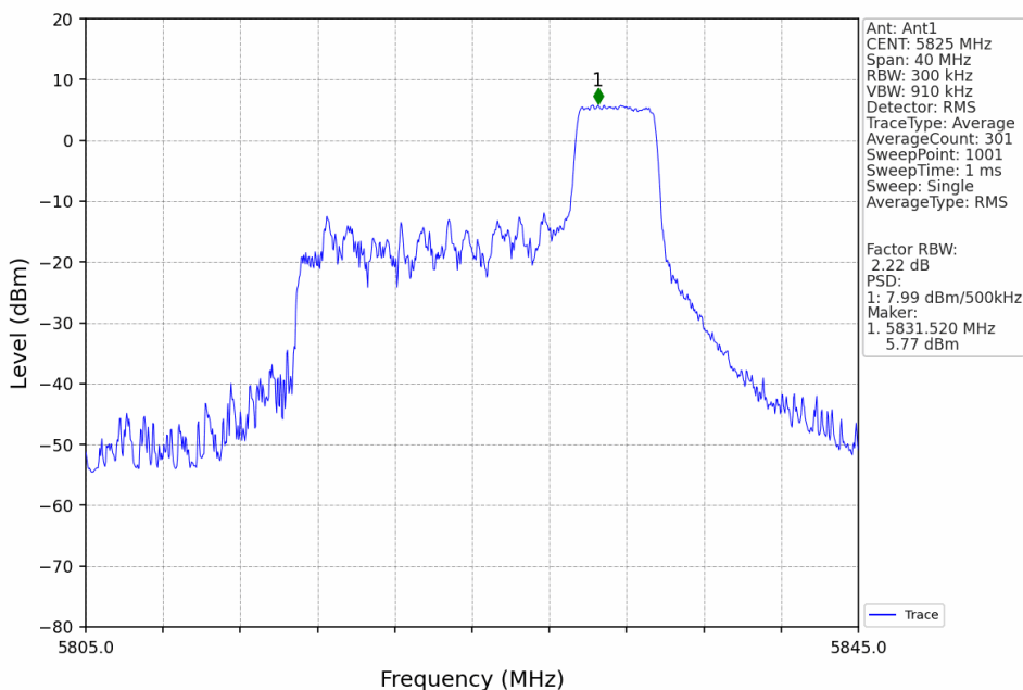
802.11ax(HEW20)_HCH_5825MHz_RU52_Right_Ant1_NTNV
