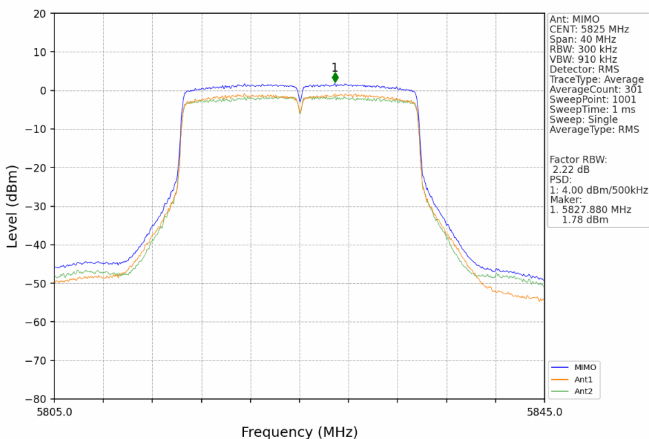
802.11ax(HEW20)_HCH_5825MHz_SU_MIMO_NTNV
