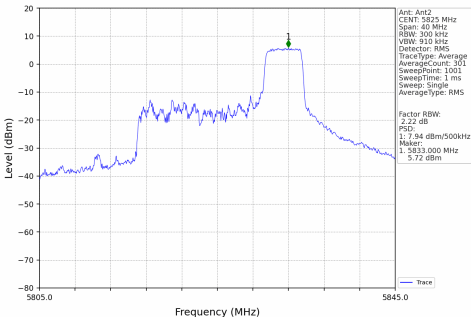
802.11ax(HEW20)_HCH_5825MHz_RU52_Right_MIMO_NTNV
