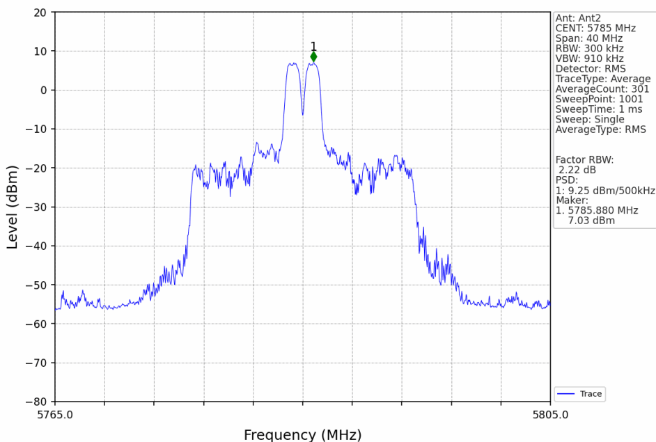
802.11ax(HEW20)_MCH_5785MHz_RU26_Mid_Ant2_NTNV
