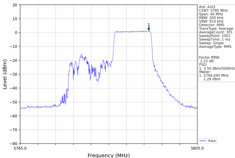
802.11ax(HEW20)_MCH_5785MHz_RU106_Right_Ant2_NTNV
