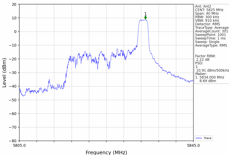
802.11ax(HEW20)_HCH_5825MHz_RU26_Right_Ant2_NTNV
