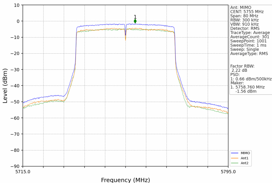
802.11ax(HEW40)_LCH_5755MHz_SU_MIMO_NTNV
