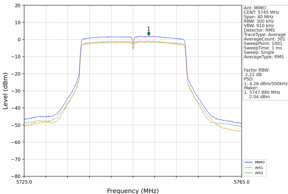
802.11ax(HEW20)_LCH_5745MHz_SU_MIMO_NTNV
