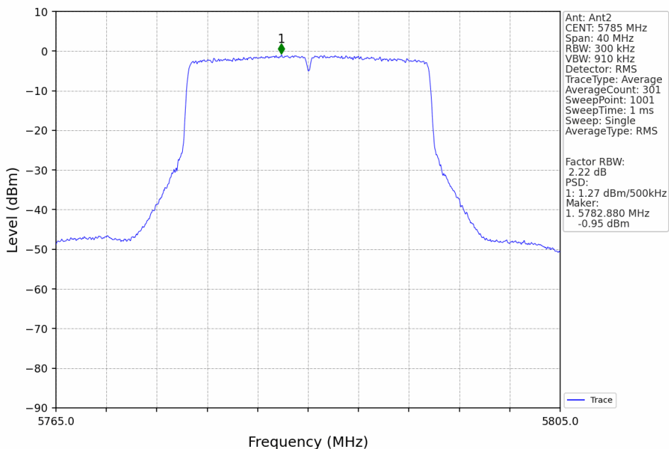
802.11ax(HEW20)_MCH_5785MHz_SU_MIMO_NTNV
