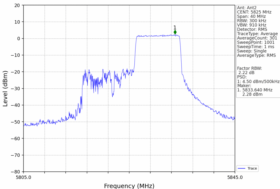
802.11ax(HEW20)_HCH_5825MHz_RU106_Right_Ant2_NTNV
