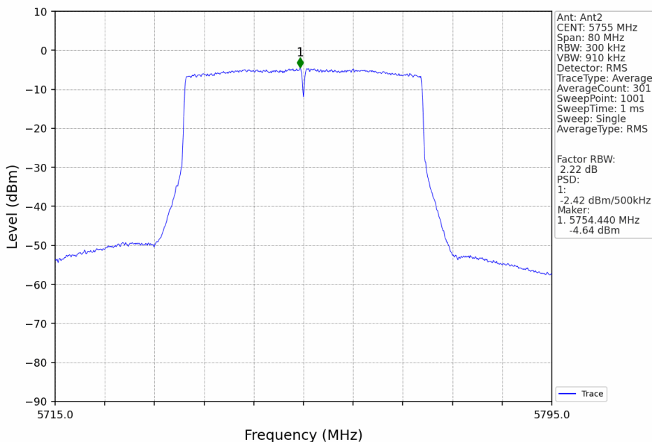
802.11ax(HEW40)_LCH_5755MHz_SU_MIMO_NTNV
