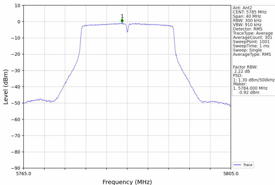
802.11ac(VHT20)_MCH_5785MHz_MIMO_NTNV
