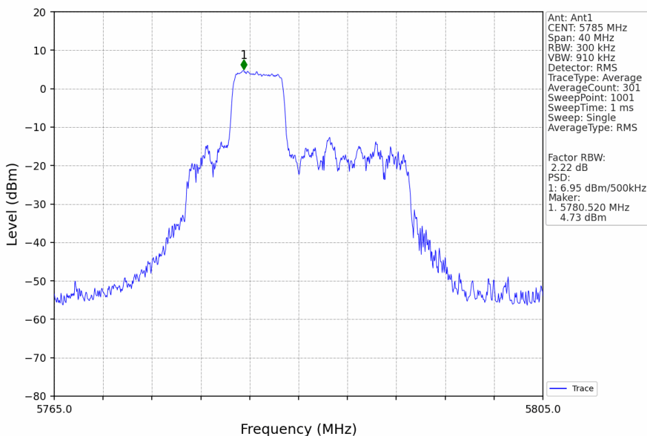
802.11ax(HEW20)_MCH_5785MHz_RU52_Mid_Ant1_NTNV
