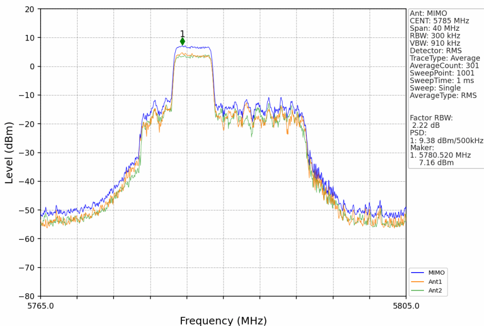
802.11ax(HEW20)_MCH_5785MHz_RU52_Mid_MIMO_NTNV
