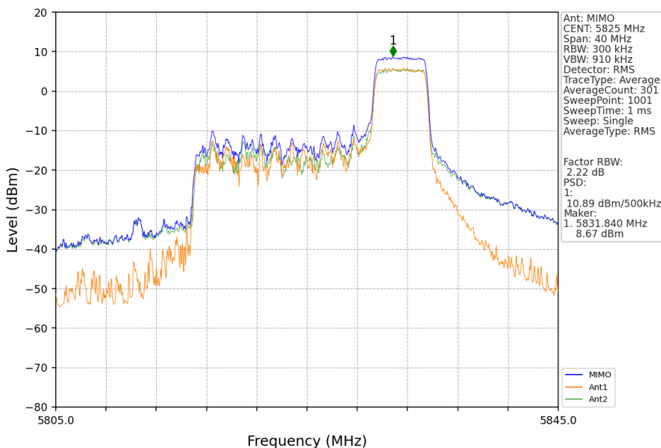
802.11ax(HEW20)_HCH_5825MHz_RU52_Right_MIMO_NTNV
