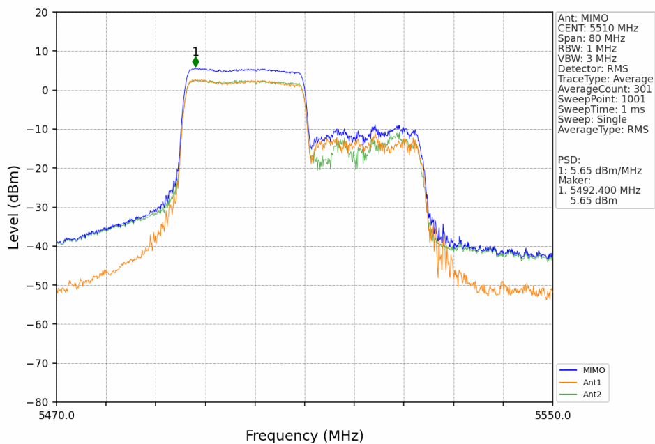
802.11ax(HEW40)_LCH_5510MHz_RU242_Left_MIMO_NTNV
