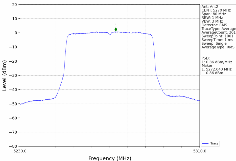
802.11ax(HEW40)_LCH_5270MHz_SU_Ant2_NTNV
