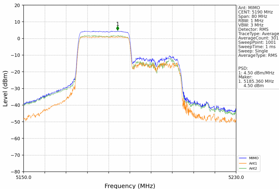
802.11ax(HEW40)_LCH_5190MHz_RU242_Left_MIMO_NTNV
