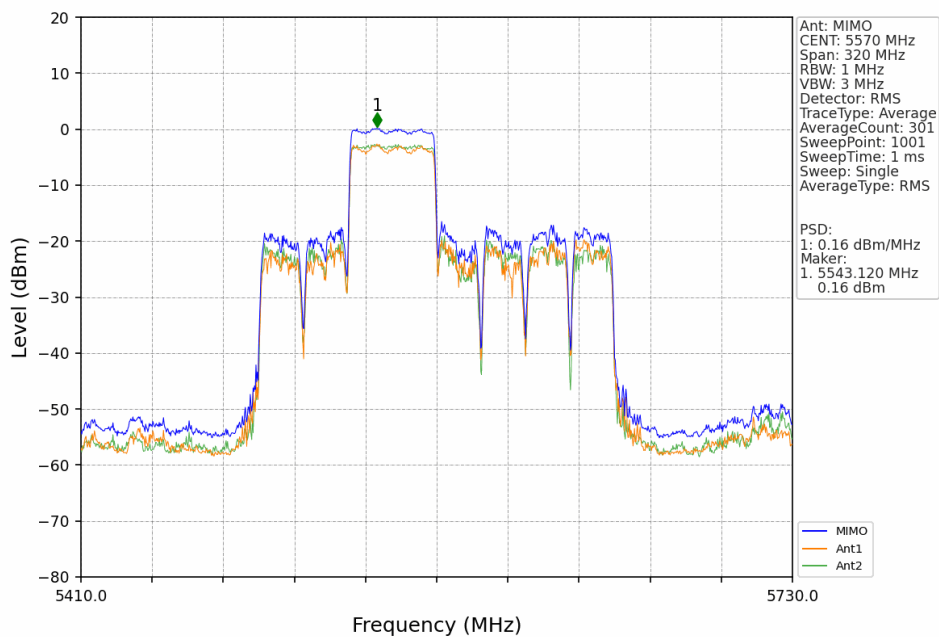
802.11ax(HEW160)_MCH_5570MHz_RU996_Right_MIMO_NTNV
