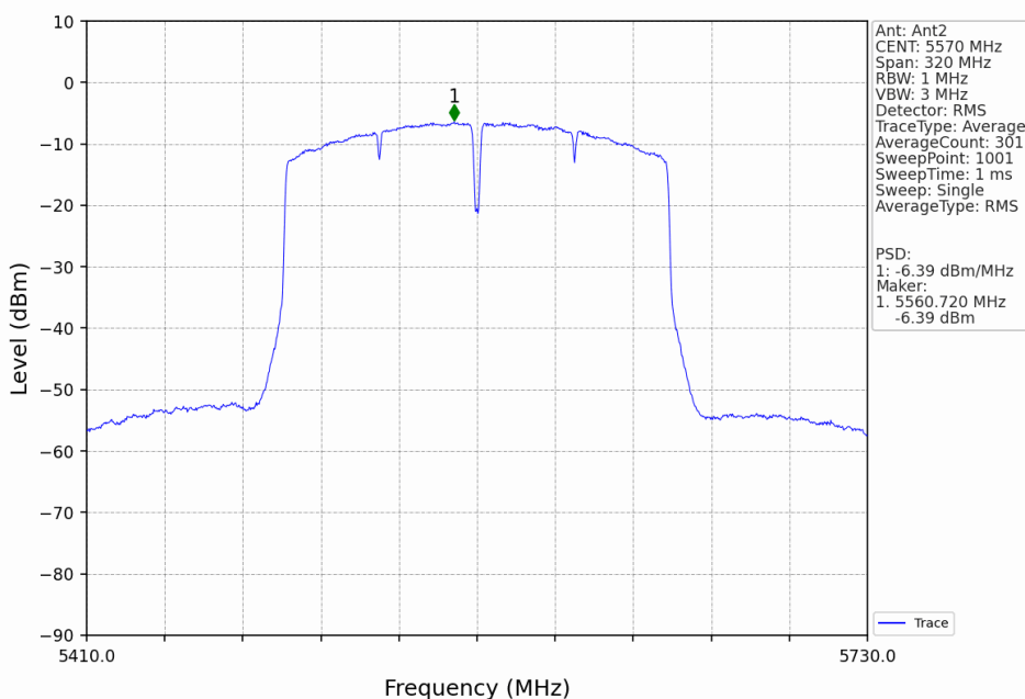
802.11ax(HEW160)_MCH_5570MHz_SU_Ant2_NTNV
