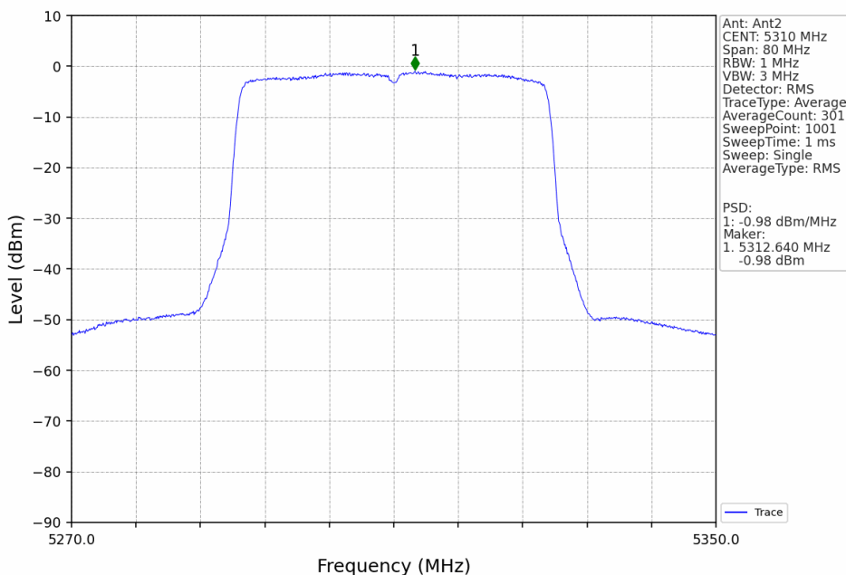
802.11ax(HEW40)_HCH_5310MHz_SU_Ant2_NTNV
