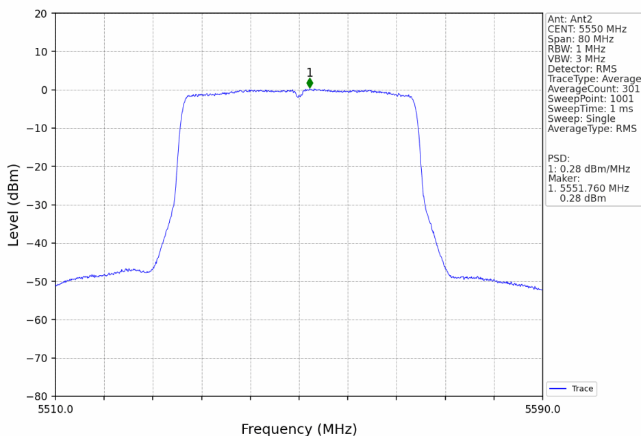
802.11ax(HEW40)_MCH_5550MHz_SU_Ant2_NTNV
