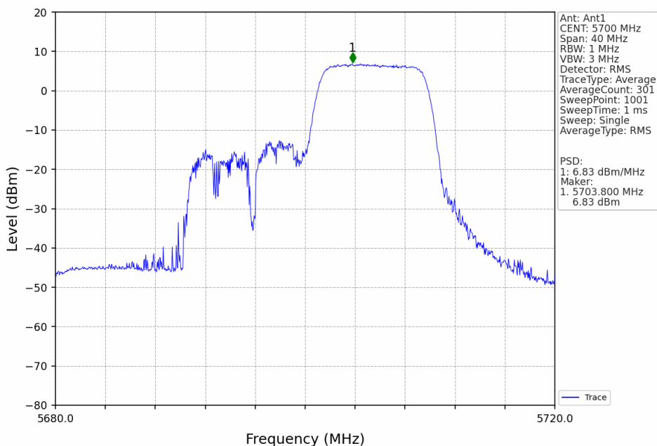
802.11ax(HEW20)_HCH_5700MHz_RU106_Right_Ant1_NTNV
