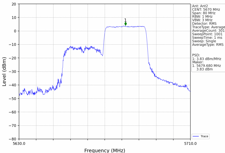
802.11ax(HEW40)_HCH_5670MHz_RU242_Right_MIMO_NTNV
