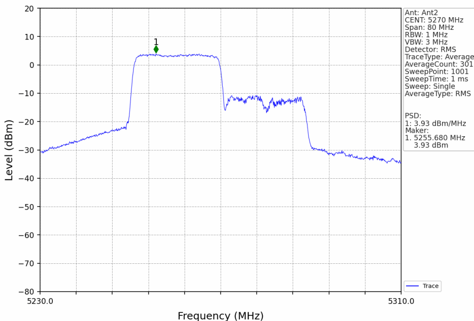
802.11ax(HEW40)_LCH_5270MHz_RU242_Left_MIMO_NTNV
