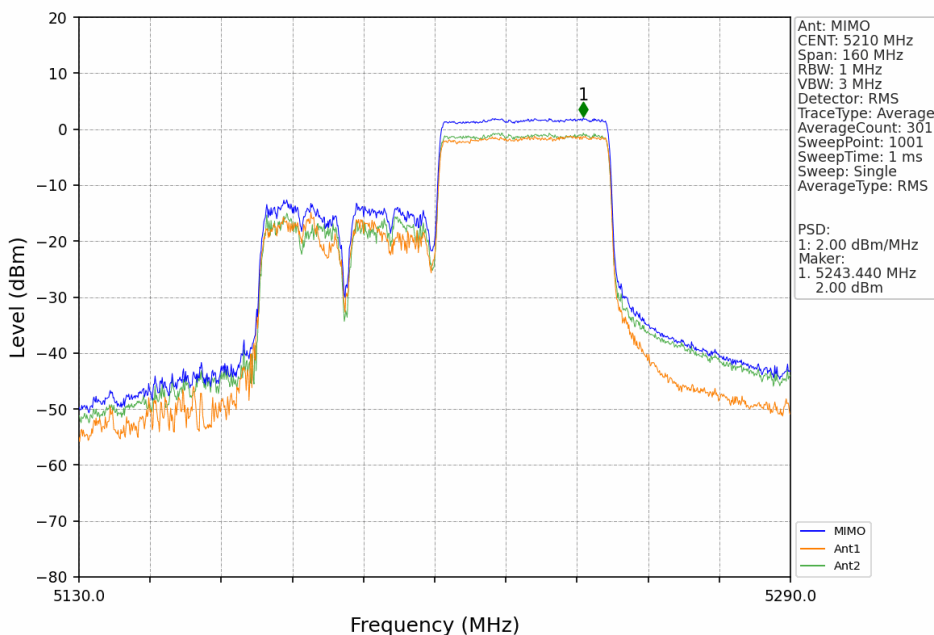
802.11ax(HEW80)_MCH_5210MHz_RU484_Right_MIMO_NTNV
