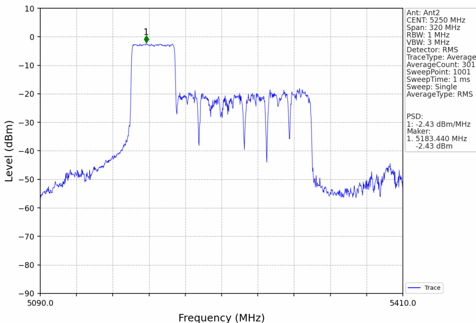
802.11ax(HEW160)_MCH_5250MHz_RU996_Left_MIMO_NTNV
