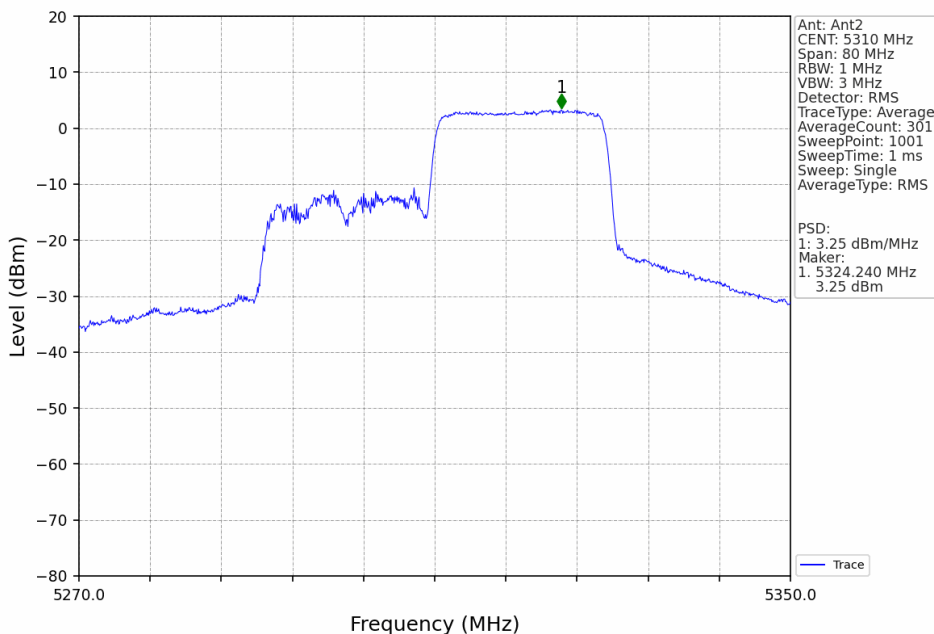
802.11ax(HEW40)_HCH_5310MHz_RU242_Right_MIMO_NTNV
