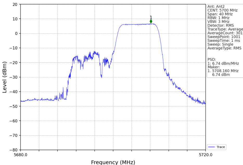
802.11ax(HEW20)_HCH_5700MHz_RU106_Right_MIMO_NTNV
