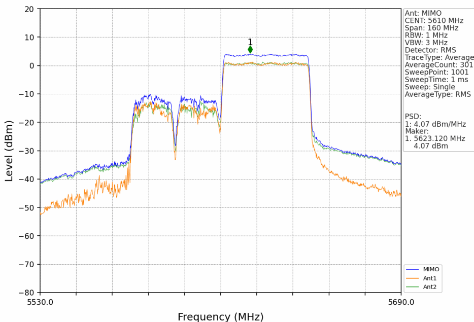
802.11ax(HEW80)_HCH_5610MHz_RU484_Right_MIMO_NTNV
