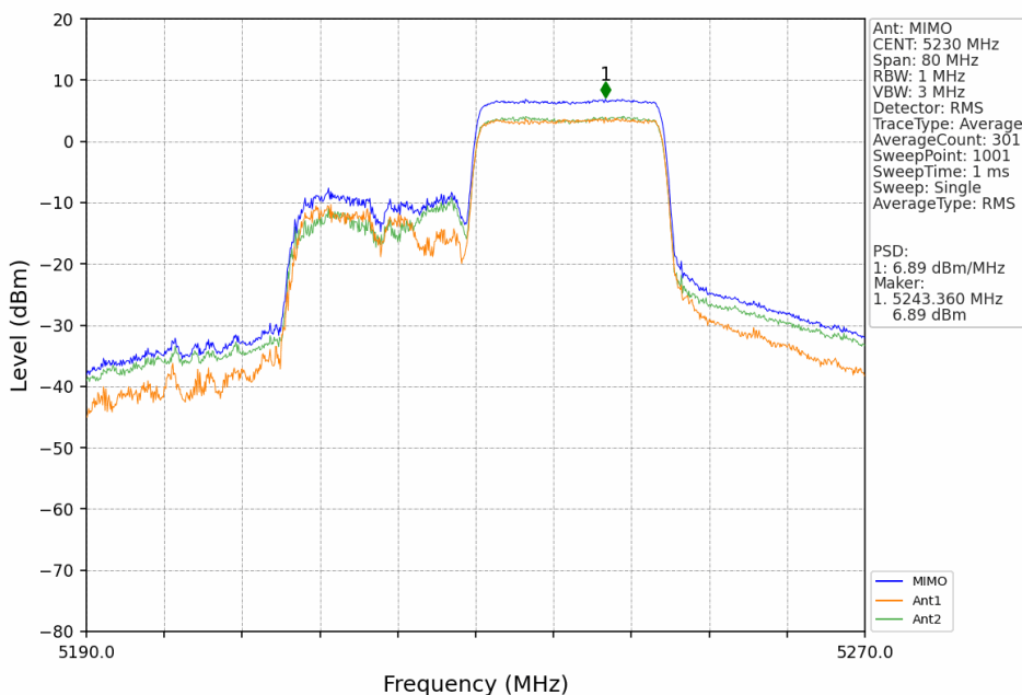
802.11ax(HEW40)_HCH_5230MHz_RU242_Right_MIMO_NTNV
