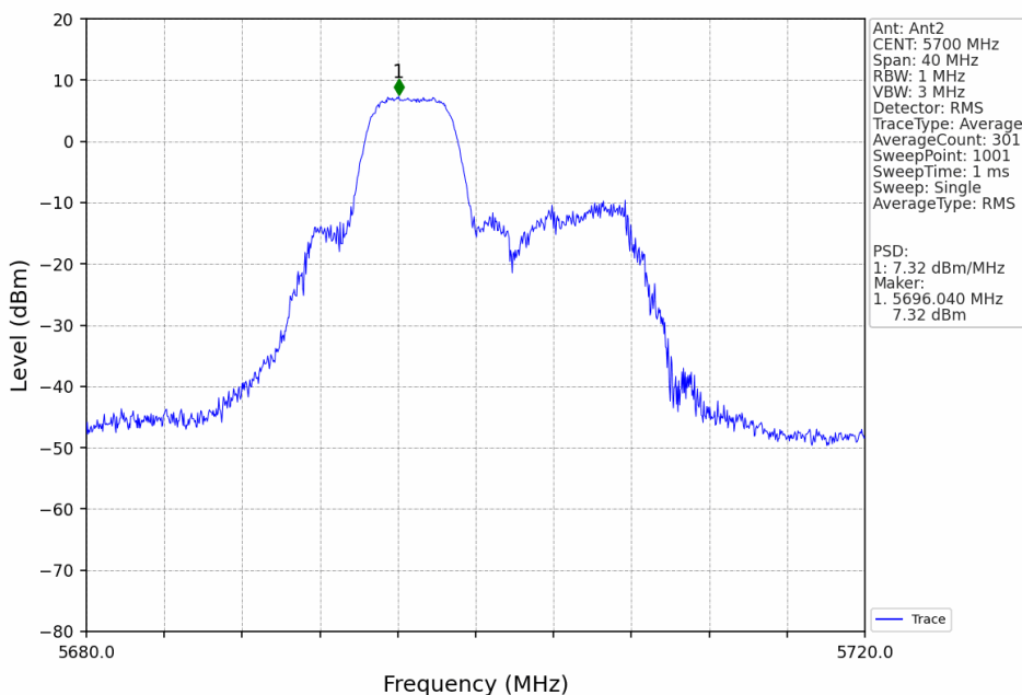
802.11ax(HEW20)_HCH_5700MHz_RU52_Right_Ant2_NTNV
