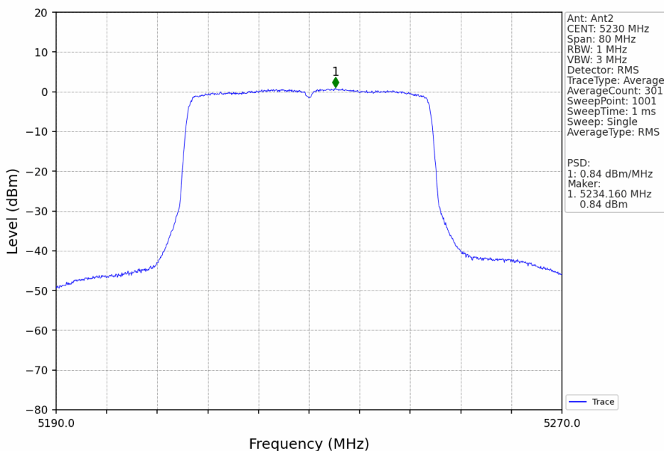
802.11ax(HEW40)_HCH_5230MHz_SU_Ant2_NTNV
