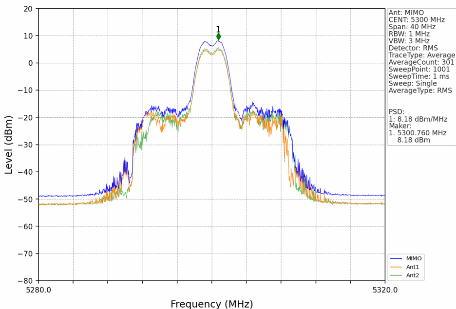
802.11ax(HEW20)_MCH_5300MHz_RU26_Mid_MIMO_NTNV
