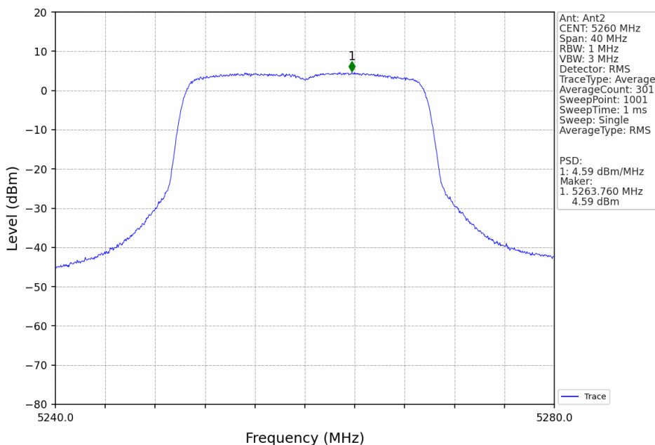
802.11ax(HEW20)_LCH_5260MHz_SU_Ant2_NTNV
