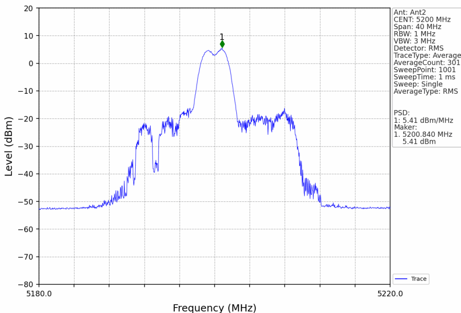
802.11ax(HEW20)_MCH_5200MHz_RU26_Mid_MIMO_NTNV
