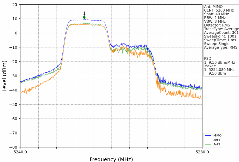
802.11ax(HEW20)_LCH_5260MHz_RU106_Left_MIMO_NTNV
