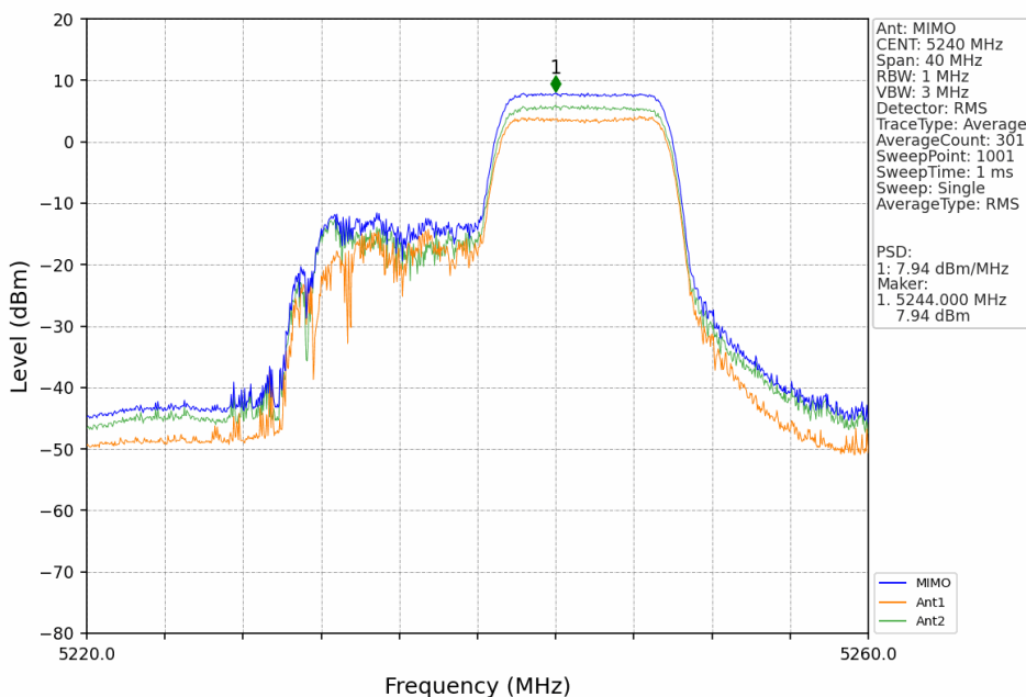
802.11ax(HEW20)_HCH_5240MHz_RU106_Right_MIMO_NTNV
