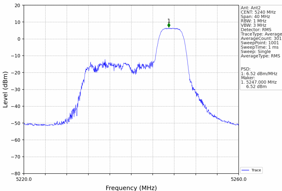
802.11ax(HEW20)_HCH_5240MHz_RU52_Right_Ant2_NTNV
