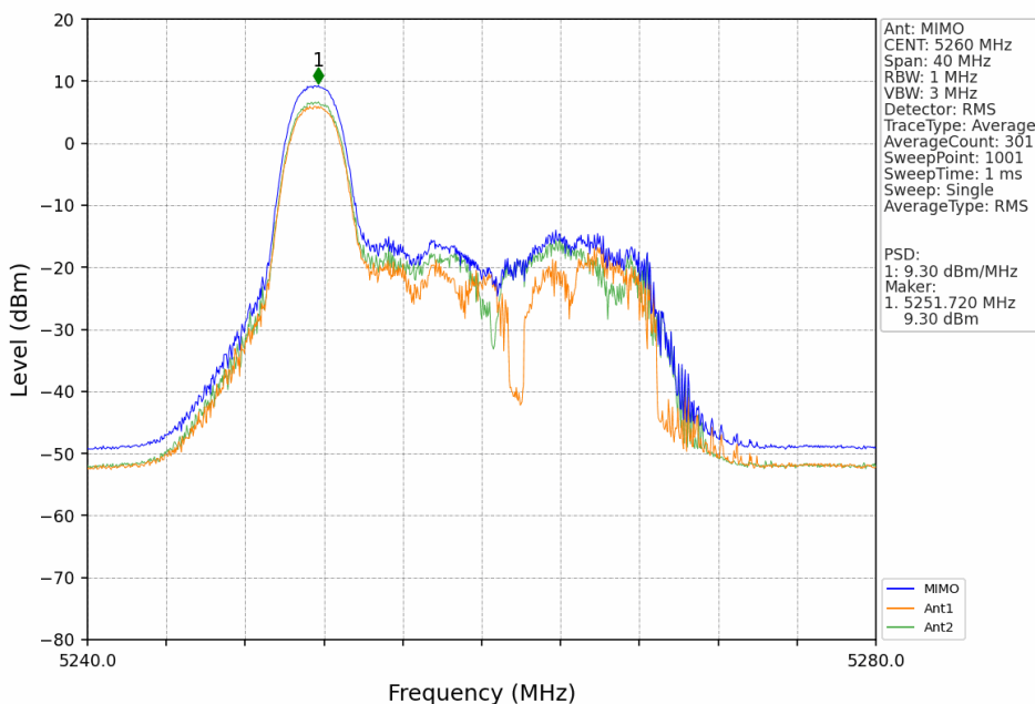
802.11ax(HEW20)_LCH_5260MHz_RU26_Left_MIMO_NTNV
