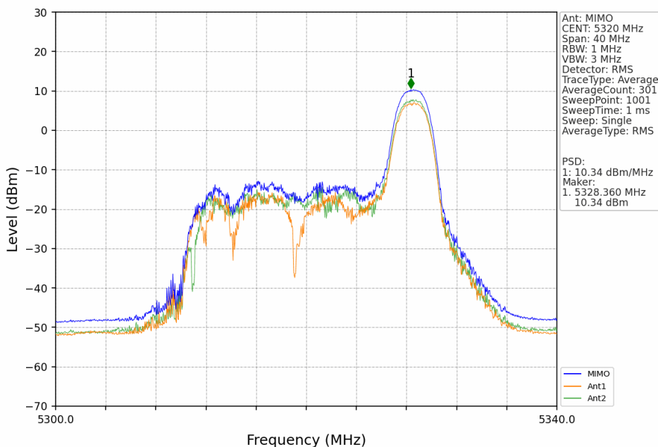
802.11ax(HEW20)_HCH_5320MHz_RU26_Right_MIMO_NTNV
