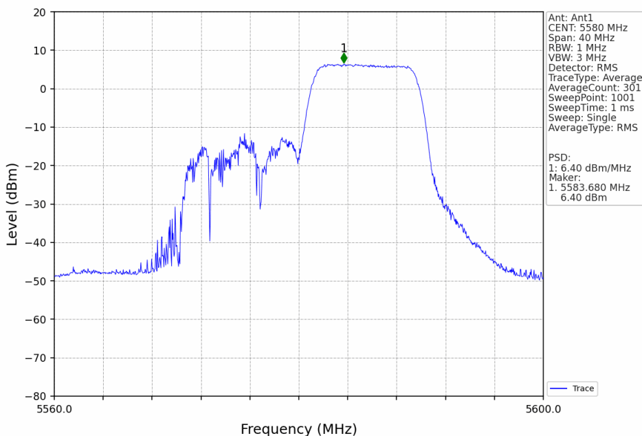
802.11ax(HEW20)_MCH_5580MHz_RU106_Right_Ant1_NTNV
