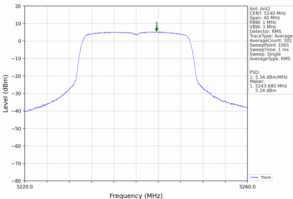
802.11ax(HEW20)_HCH_5240MHz_SU_Ant2_NTNV
