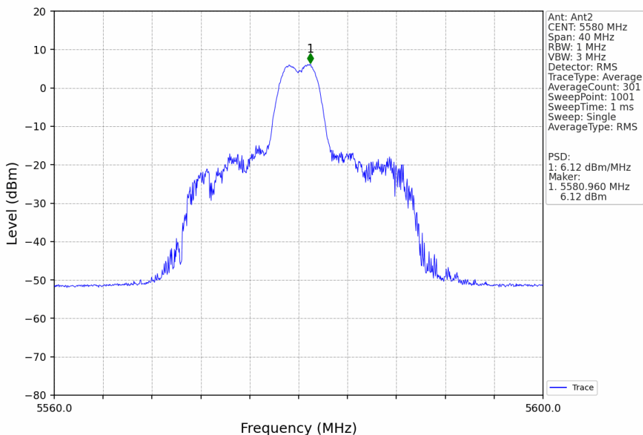
802.11ax(HEW20)_MCH_5580MHz_RU26_Mid_MIMO_NTNV
