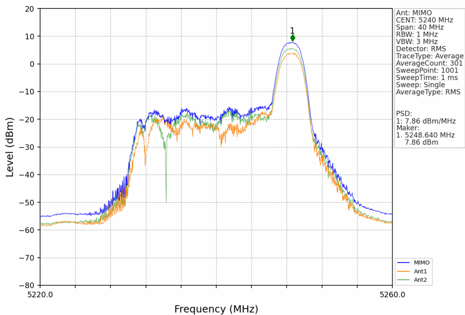
802.11ax(HEW20)_HCH_5240MHz_RU26_Right_MIMO_NTNV
