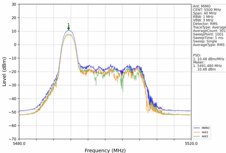
802.11ax(HEW20)_LCH_5500MHz_RU26_Left_MIMO_NTNV
