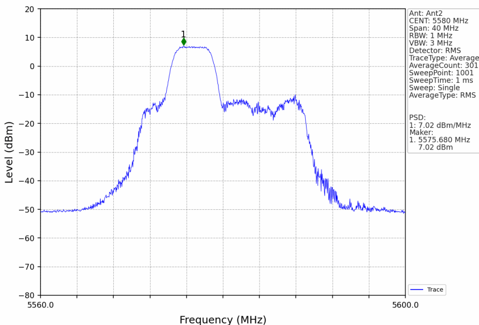
802.11ax(HEW20)_MCH_5580MHz_RU52_Mid_Ant2_NTNV
