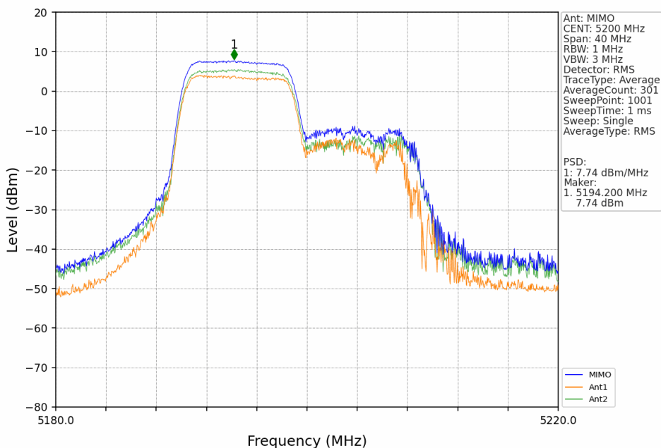
802.11ax(HEW20)_MCH_5200MHz_RU106_Right_MIMO_NTNV
