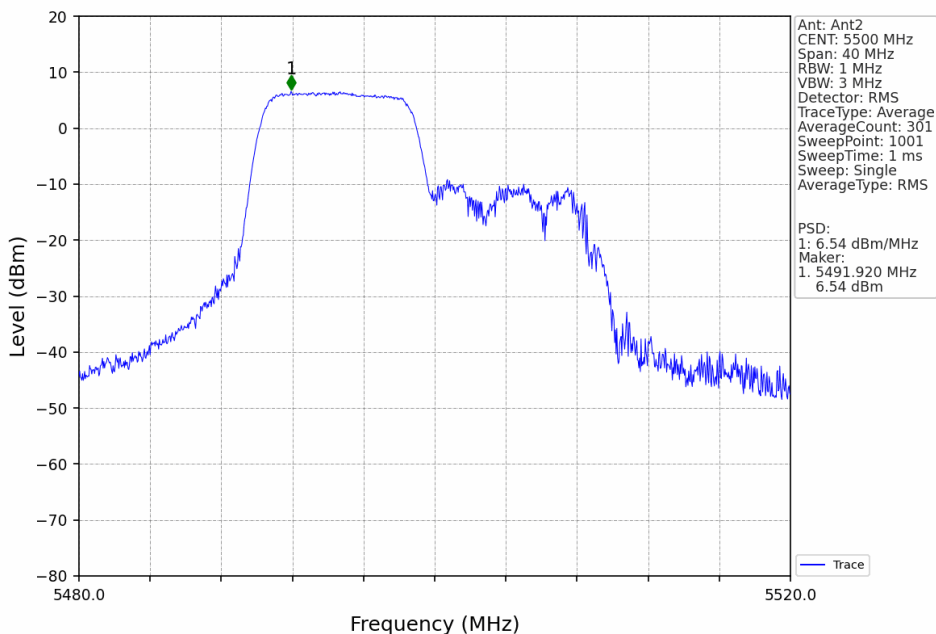
802.11ax(HEW20)_LCH_5500MHz_RU106_Left_MIMO_NTNV
