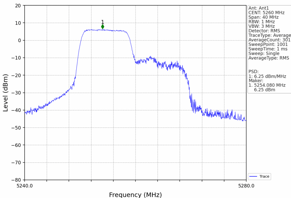
802.11ax(HEW20)_LCH_5260MHz_RU106_Left_Ant1_NTNV
