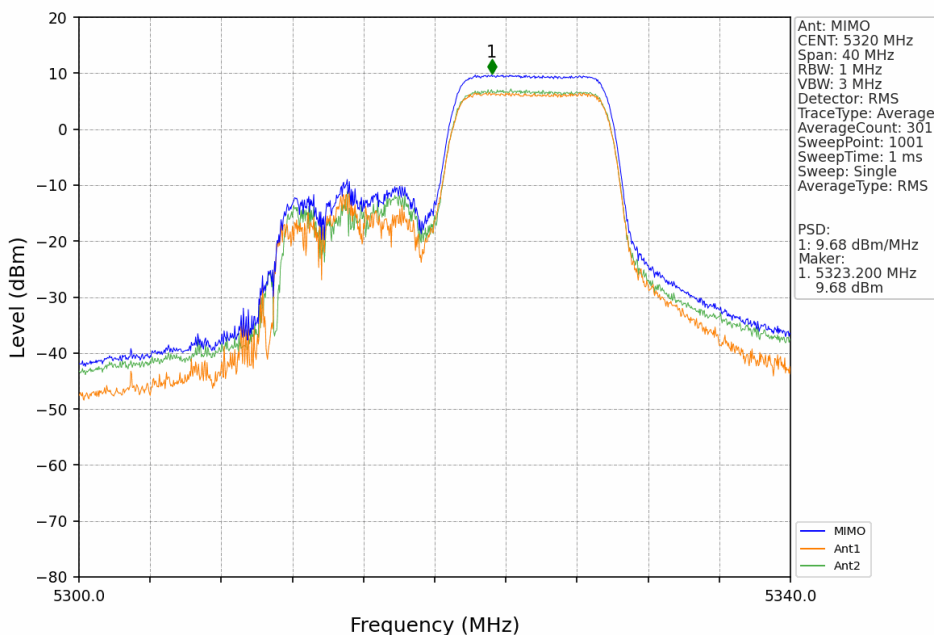
802.11ax(HEW20)_HCH_5320MHz_RU106_Right_MIMO_NTNV
