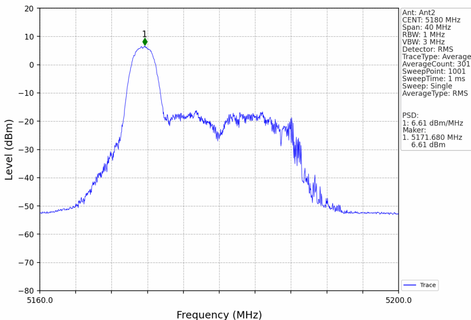
802.11ax(HEW20)_LCH_5180MHz_RU26_Left_MIMO_NTNV
