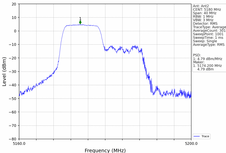
802.11ax(HEW20)_LCH_5180MHz_RU106_Left_MIMO_NTNV
