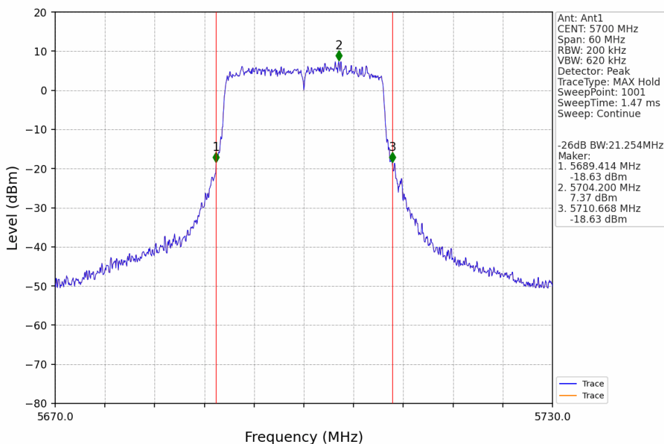
802.11ax(HEW20)_HCH_5700MHz_SU_Ant1_NTNV
