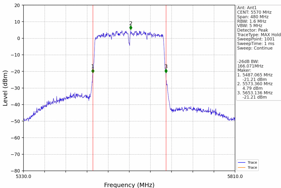
802.11ax(HEW160)_MCH_5570MHz_SU_Ant1_NTNV
