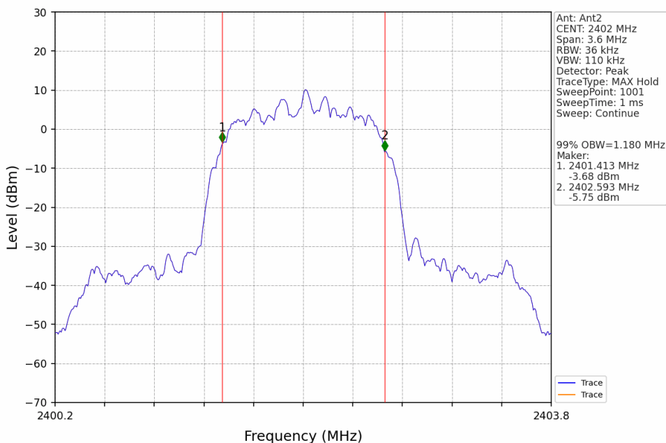
Pi/4DQPSK_2DH5_LCH_2402MHz_Ant2_NTNV
