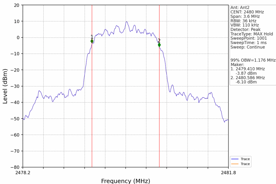
Pi/4DQPSK_2DH5_HCH_2480MHz_Ant2_NTNV
