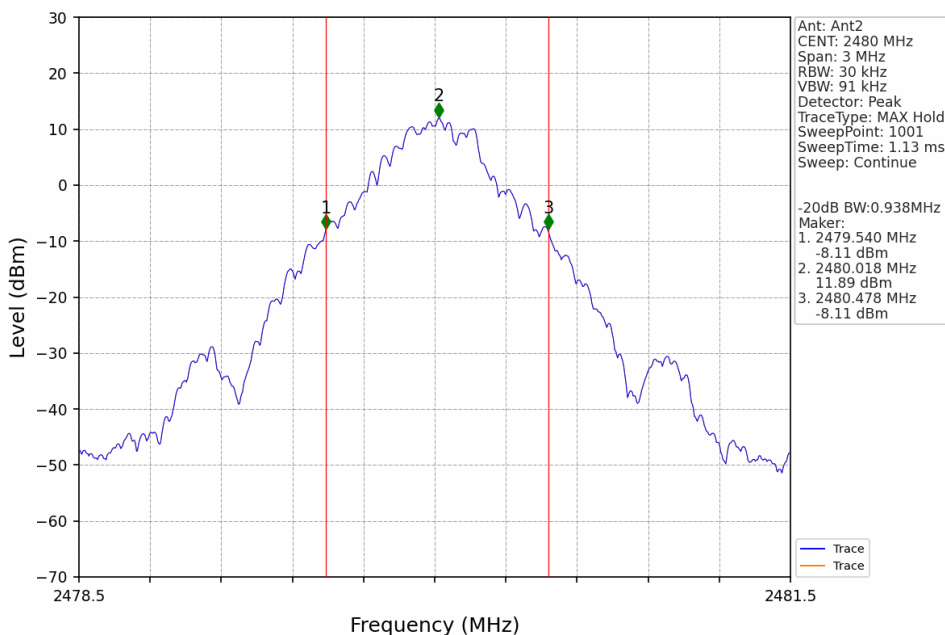
GFSK_DH5_HCH_2480MHz_Ant2_NTNV
