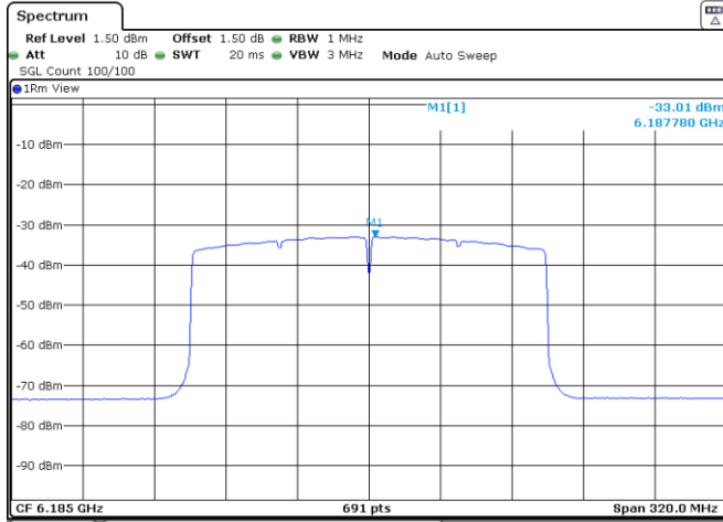
Port 1 Conducted PSD
