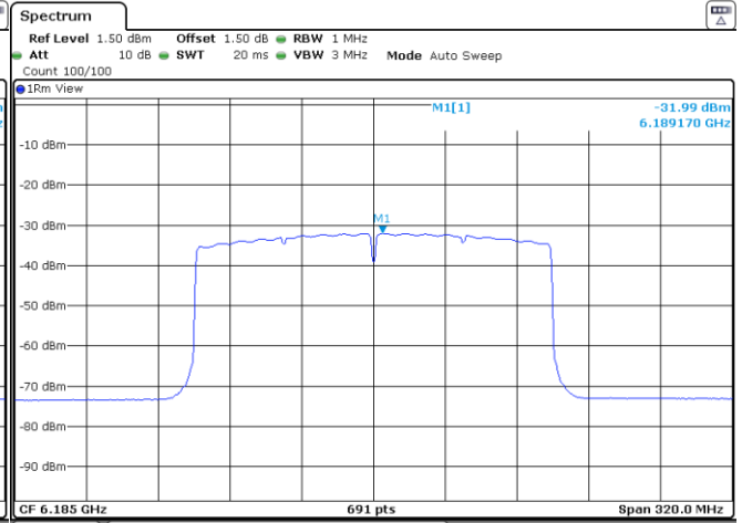
Port 2 Conducted PSD
