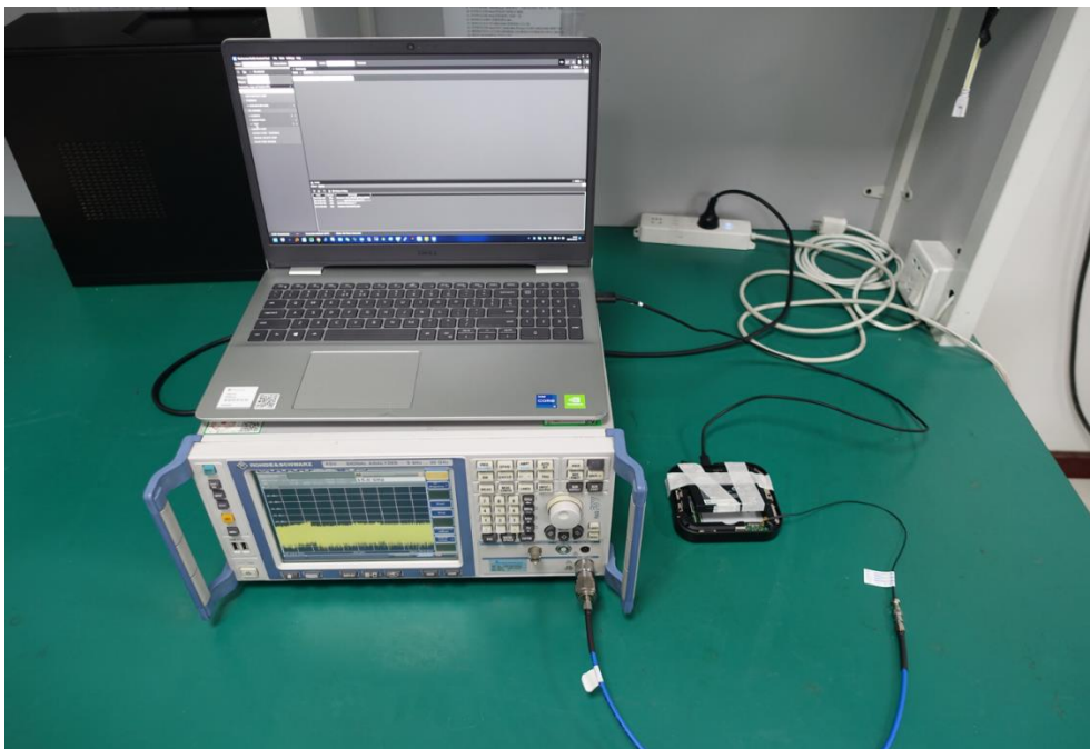
Figure 2: EUT connect to spectrum analyzer
