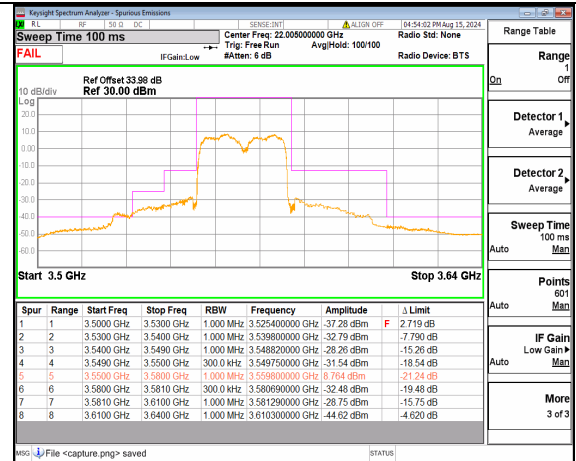
n48 30M DFT-s-OFDM QPSK Outer_Full Low
