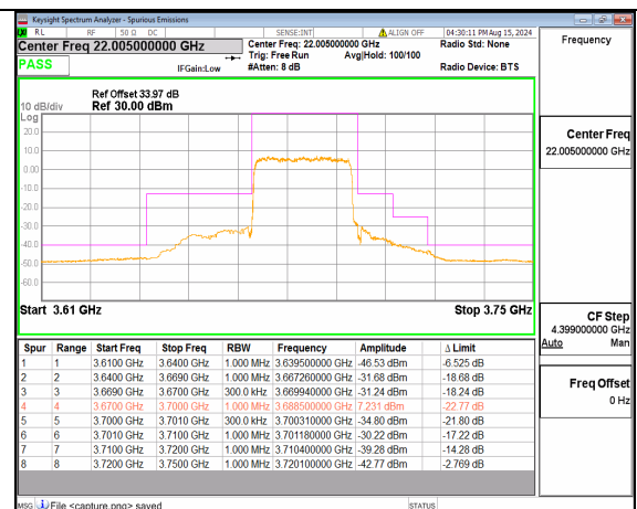
n48 30M DFT-s-OFDM QPSK Outer_Full High
