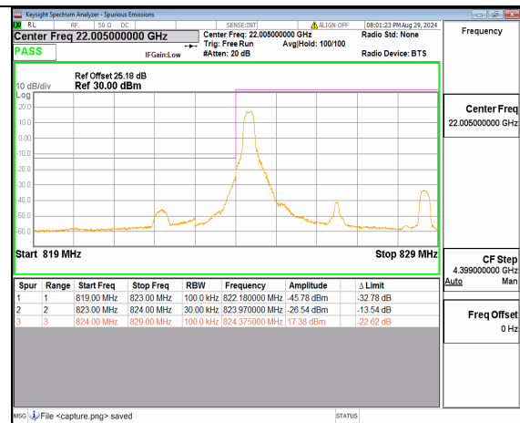
n5 5M DFT-s-OFDM 16QAM Edge_1RB_Left Low
