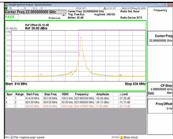
n5 10M DFT-s-OFDM 16QAM Edge_1RB_Left Low
