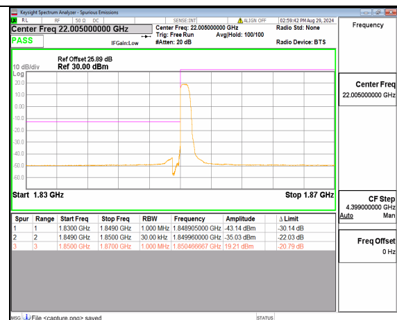
n2 20M DFT-s-OFDM 16QAM Edge_1RB_Left Low
