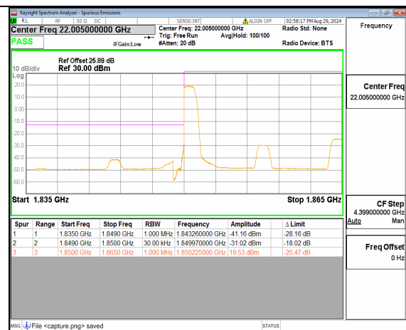
n2 15M DFT-s-OFDM 16QAM Edge_1RB_Left Low
