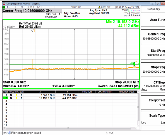
n48 (30MHz-20GHz) 40M DFT-s-OFDM BPSK Inner_1RB_Left Low
