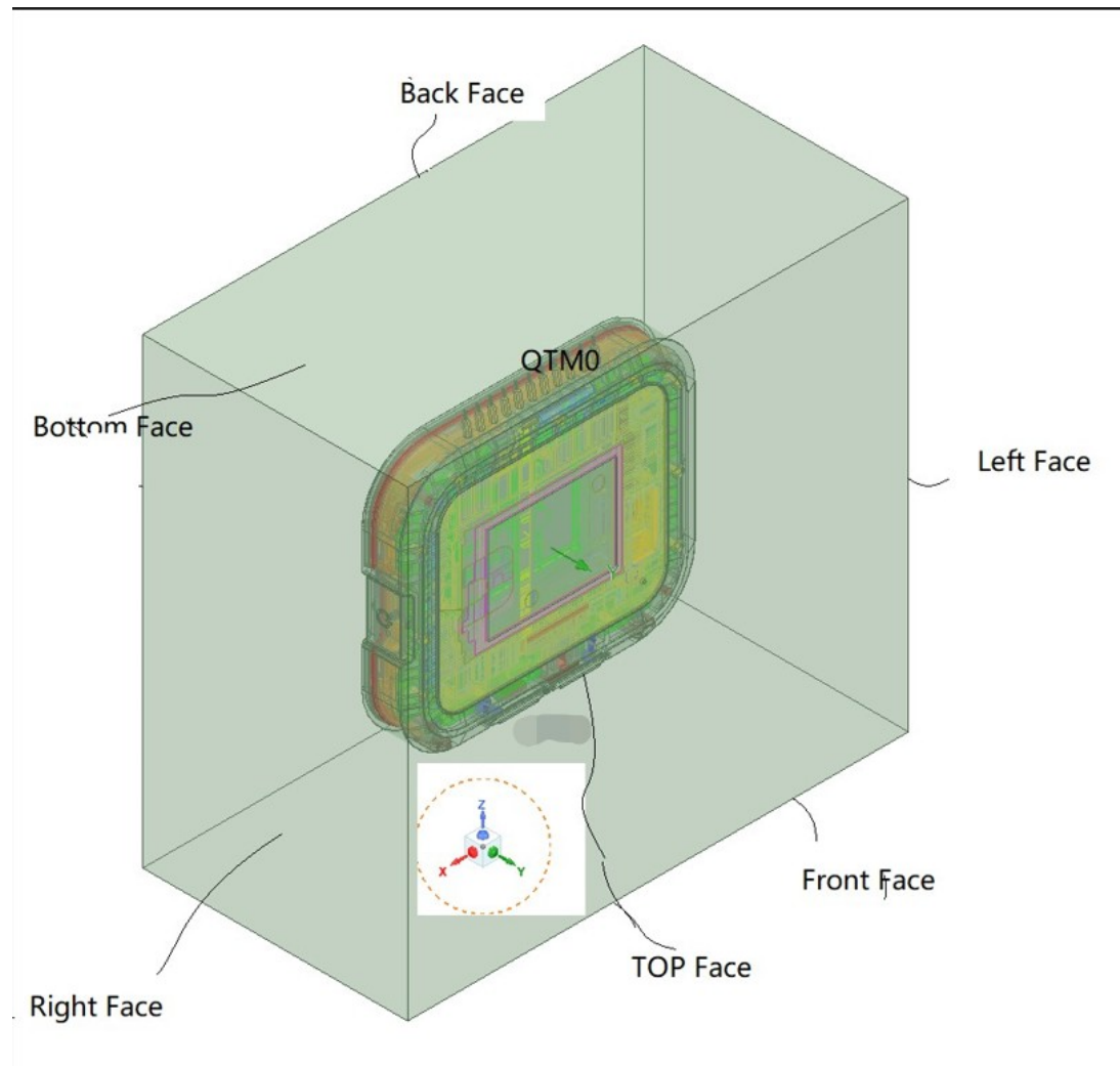
Figure 3.1-2: EUT simulation model
