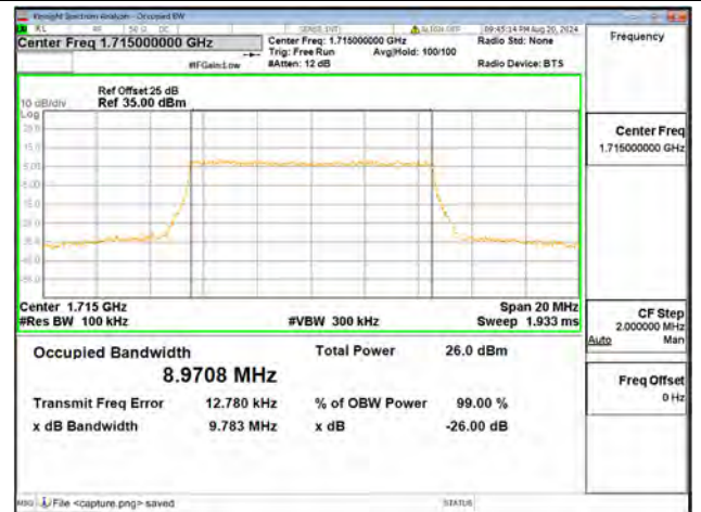
B66 / 10MHz / 256QAM/ Low CH
