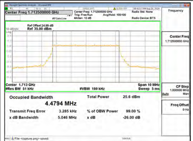
B66 / 5MHz / 256QAM/ Low CH
