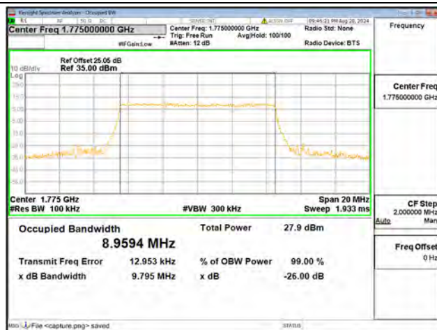
B66 / 10MHz / 64QAM/ High CH
