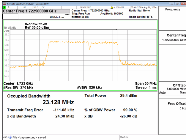
66C / 15+10MHz / 64QAM/ Low CH
