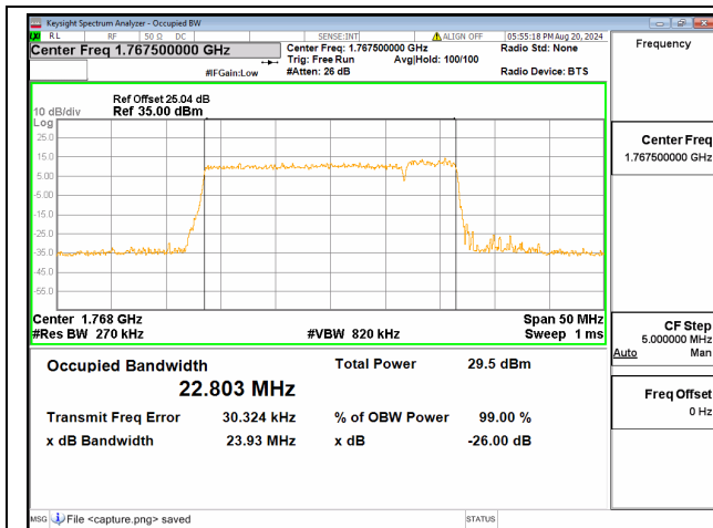
66C / 20+5MHz / 64QAM/ High CH
