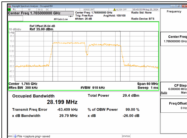
66C / 15+15MHz / 64QAM/ High CH
