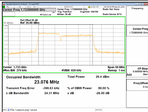
66C / 10+15MHz / 64QAM/ Low CH
