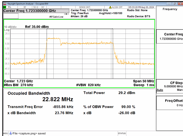
66C / 5+20MHz / 64QAM/ Low CH
