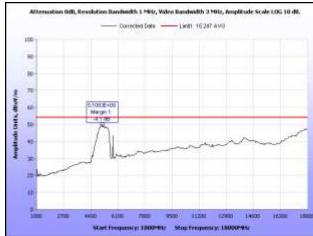
Plot 43. Radiated Spurious Emissions, 5785 MHz, 1 GHz – 18 GHz, Average, Dish Antenna
