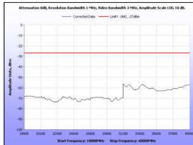
Plot 66. EIRP, 5785 MHz, 18 GHz – 40 GHz, Dish Antenna
