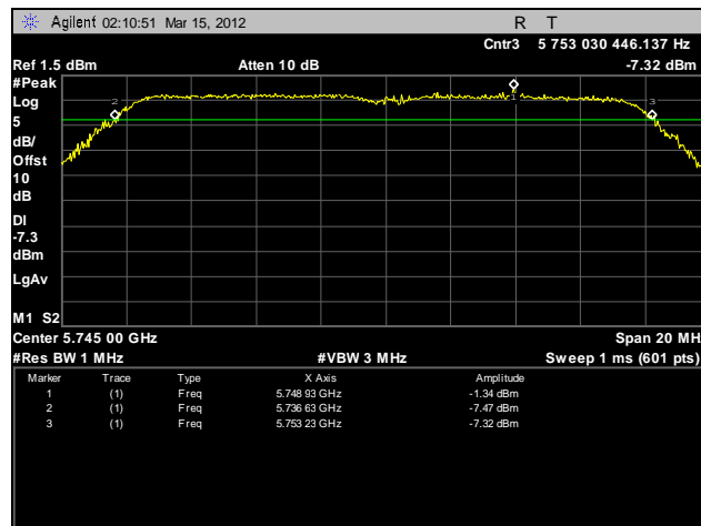
Plot 79. Frequency Stability, 5725 – 5825 MHz, 20°C, 120 V
