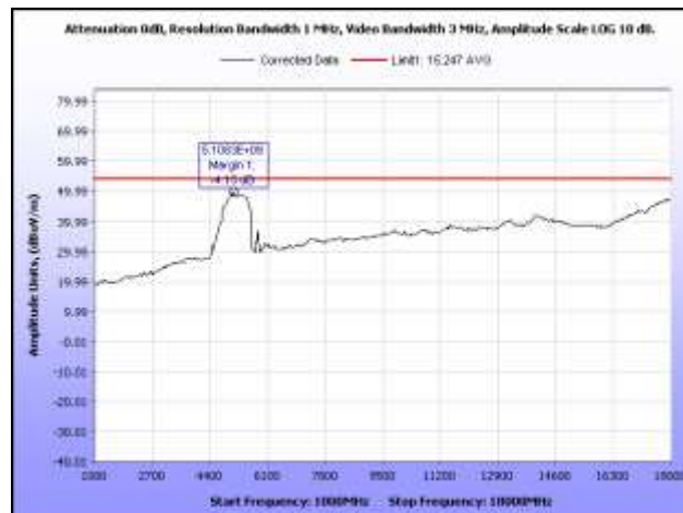
Plot 48. Radiated Spurious Emissions, 5805 MHz, 1 GHz – 18 GHz, Average, Dish Antenna
