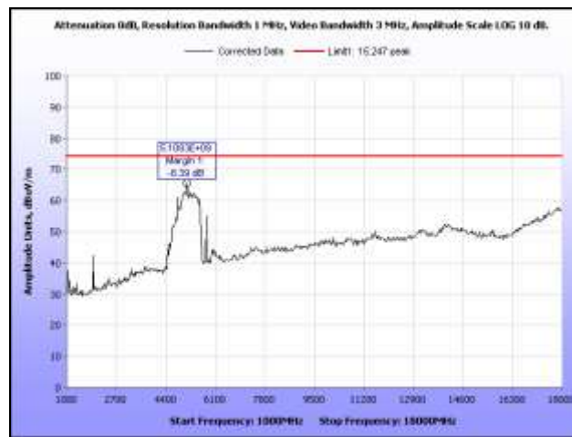
Plot 44. Radiated Spurious Emissions, 5785 MHz, 1 GHz – 18 GHz, Peak Antenna, Dish Antenna
