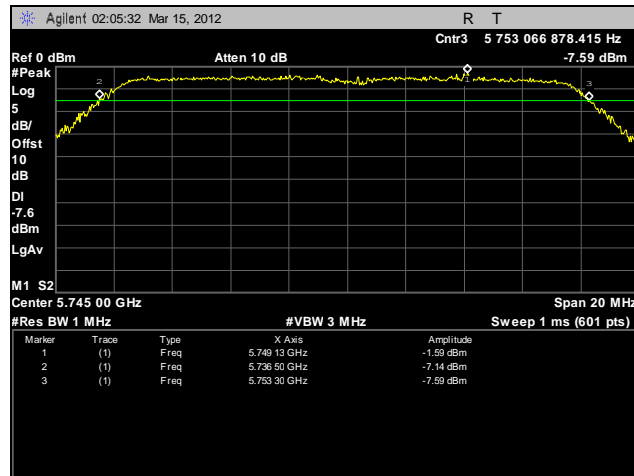
Plot 81. Frequency Stability, 5725 – 5825 MHz, 30°C, 120 V
