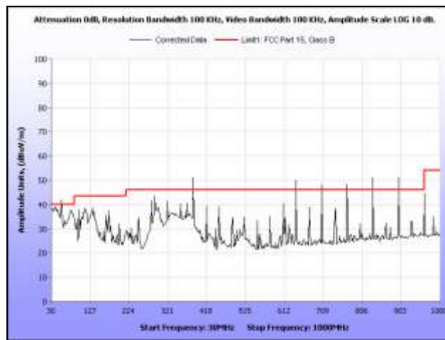
Plot 32. Radiated Spurious Emissions, 5805 MHz, 30 MHz – 1 GHz, Omni Antenna
