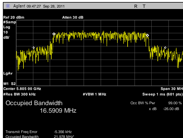
Plot 12. 99% Occupied Bandwidth, 5805 MHz
