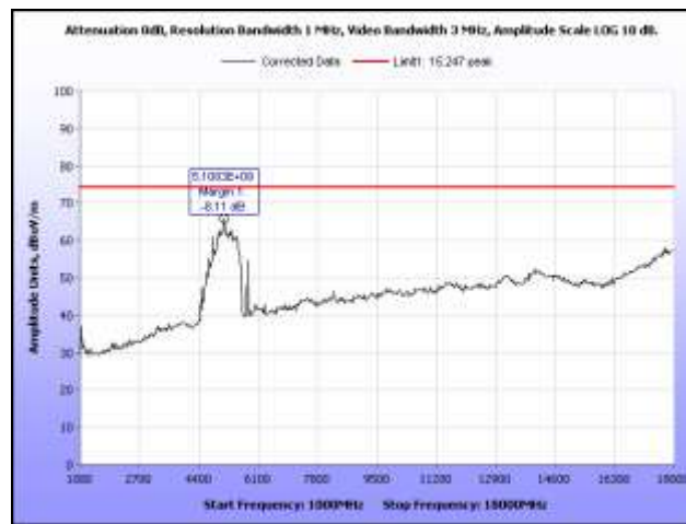
Plot 29. Radiated Spurious Emissions, 5785 MHz, 1 GHz – 18 GHz, Peak, Omni Antenna
