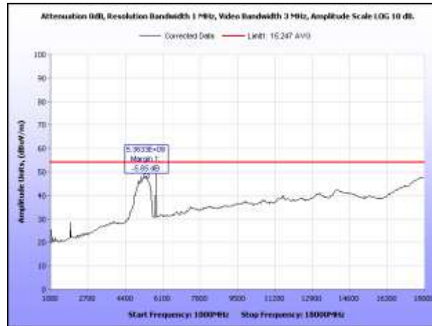
Plot 28. Radiated Spurious Emissions, 5785 MHz, 1 GHz – 18 GHz, Average, Omni Antenna
