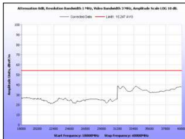
Plot 30. Radiated Spurious Emissions, 5785 MHz, 18 GHz – 40 GHz, Average, Omni Antenna
