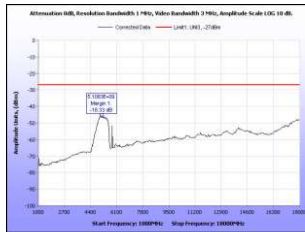
Plot 65. EIRP, 5785 MHz, 1 GHz – 18 GHz, Dish Antenna
