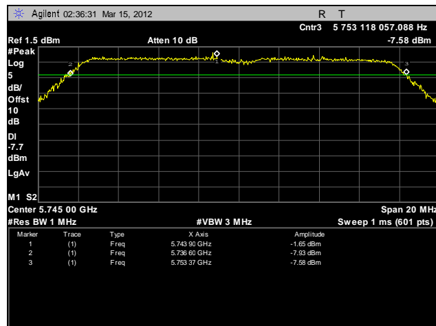
Plot 76. Frequency Stability, 5725 – 5825 MHz, 0°C, 120 V
