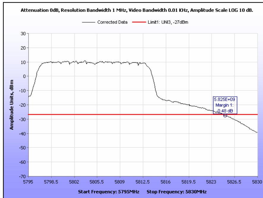
Plot 73. Radiated Band Edge, 5805 MHz, Dish Antenna
