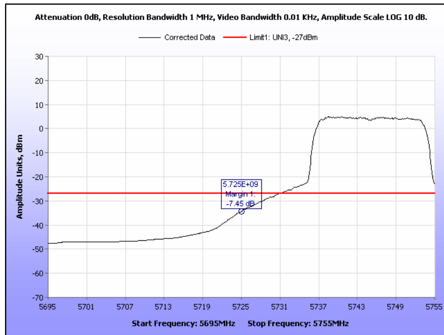
Plot 70. Radiated Band Edge, 5745 MHz
