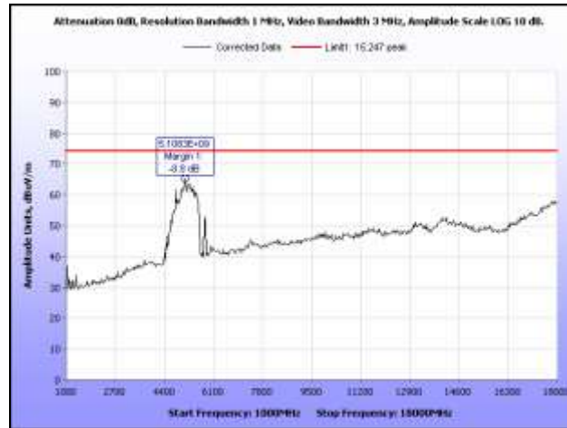
Plot 49. Radiated Spurious Emissions, 5805 MHz, 1 GHz – 18 GHz, Peak, Dish Antenna
