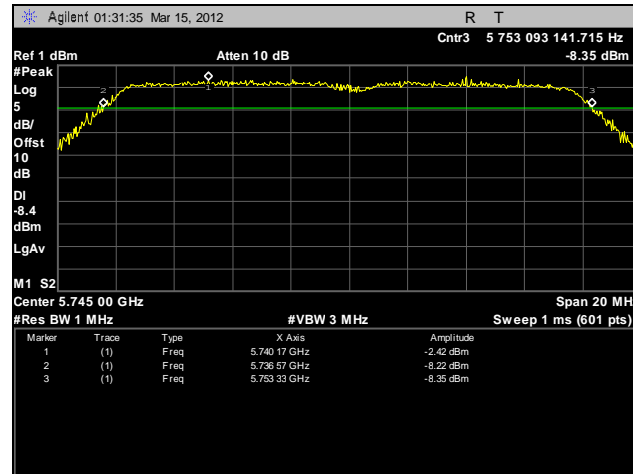
Plot 83. Frequency Stability, 5725 – 5825 MHz, 50°C, 120 V
