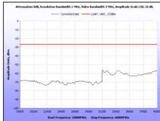
Plot 63. EIRP, 5745 MHz, 18 GHz – 40 GHz, Dish Antenna
