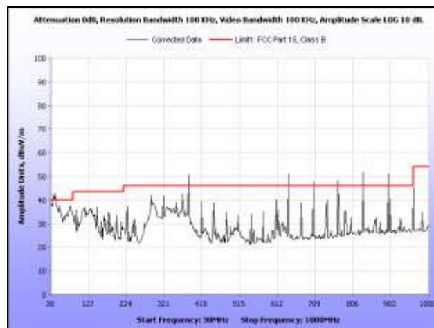
Plot 27. Radiated Spurious Emissions, 5785 MHz, 30 MHz – 1 GHz, Omni Antenna
