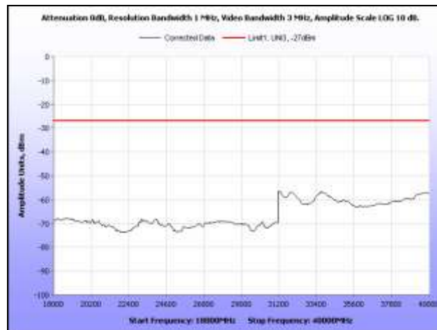
Plot 57. EIRP, 5785 MHz, 18 GHz – 40 GHz, Omni Antenna
