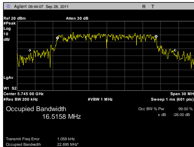
Plot 7. 26 dB Occupied Bandwidth, 5745 MHz
