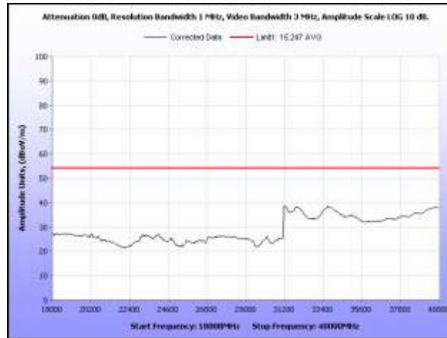
Plot 40. Radiated Spurious Emissions, 5745 MHz, 18 GHz – 40 GHz, Average, Dish Antenna
