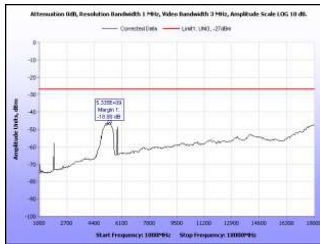
Plot 59. EIRP, 5805 MHz, 1 GHz – 18 GHz, Omni Antenna
