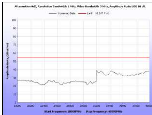
Plot 50. Radiated Spurious Emissions, 5805 MHz, 18 GHz – 40 GHz, Average, Dish Antenna
