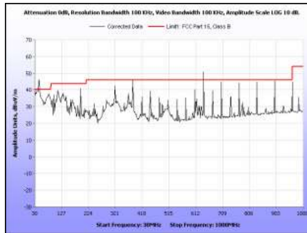
Plot 22. Radiated Spurious Emissions, 5745 MHz, 30 MHz – 1 GHz, Omni Antenna
