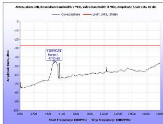
Plot 53. EIRP, 5745 MHz, 1 GHz – 18 GHz, Omni Antenna
