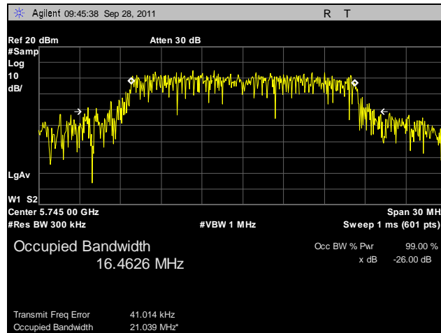
Plot 10. 99% Occupied Bandwidth, 5745 MHz
