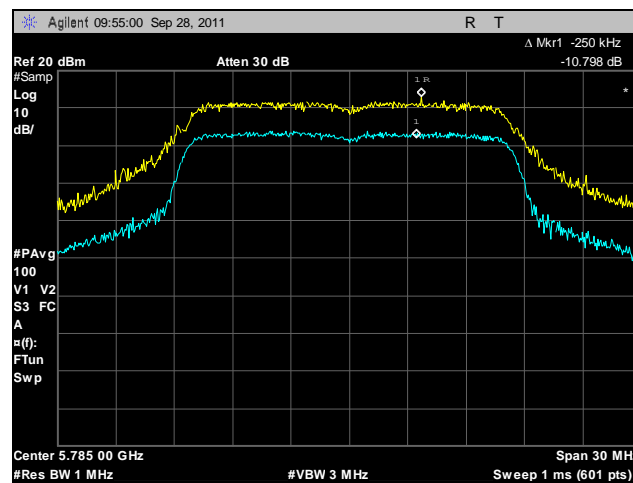
Plot 20. Peak Excursion Ratio, 5785 MHz
