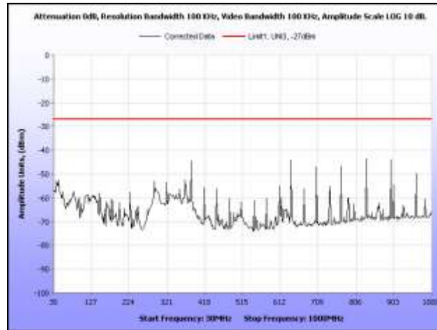
Plot 55. EIRP, 5785 MHz, 30 MHz – 1 GHz, Omni Antenna
