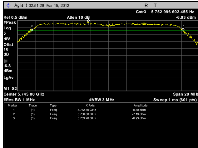
Plot 74. Frequency Stability, 5725 – 5825 MHz, -20°C, 120 V
