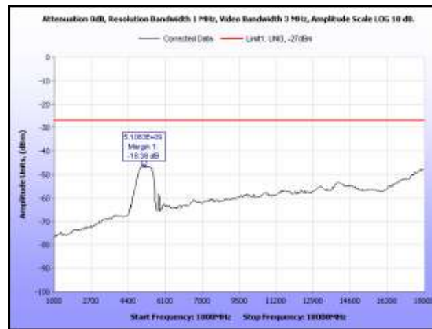
Plot 68. EIRP, 5805 MHz, 1 GHz – 18 GHz, Dish Antenna
