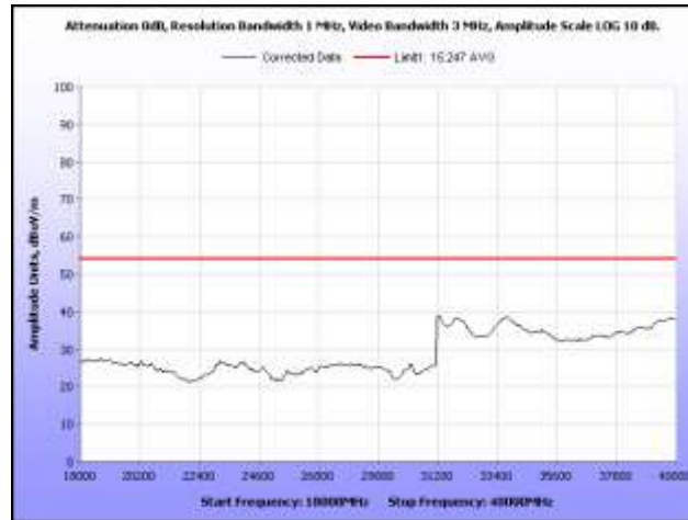
Plot 25. Radiated Spurious Emissions, 5745 MHz, 18 GHz – 40 GHz, Average, Omni Antenna
