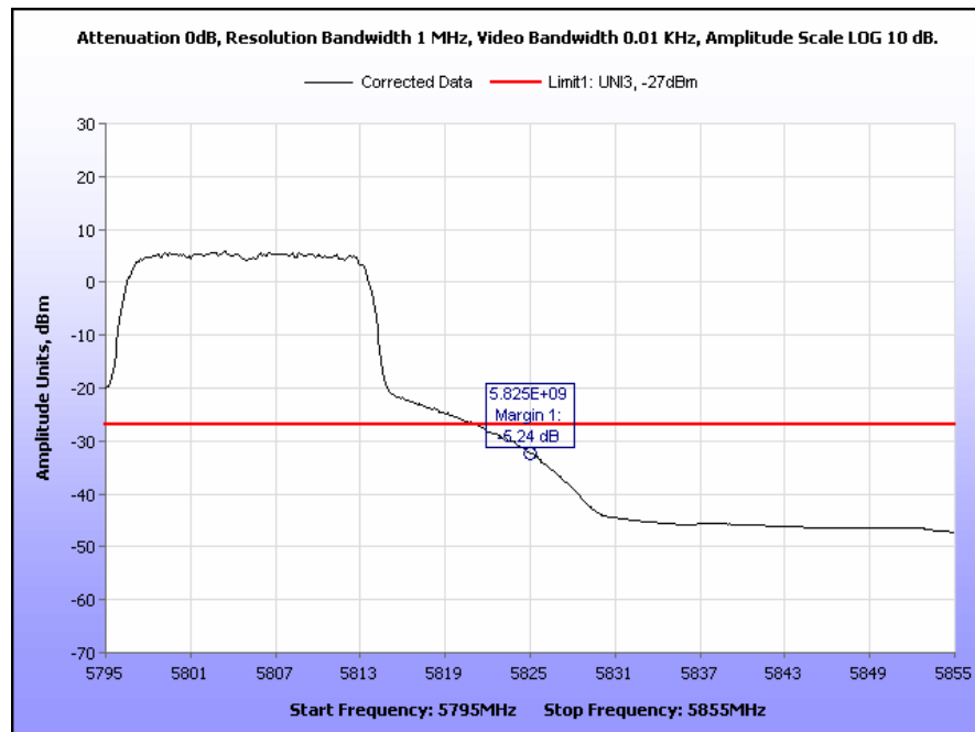
Plot 71. Radiated Band Edge, 5805 MHz
