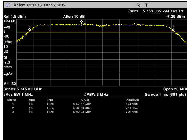
Plot 80. Frequency Stability, 5725 – 5825 MHz, 20°C, 132 V
