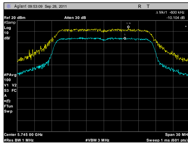
Plot 19. Peak Excursion Ratio, 5745 MHz
