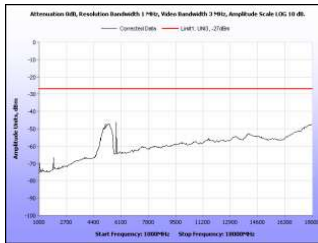
Plot 56. EIRP, 5785 MHz, 1 GHz – 18 GHz, Omni Antenna
