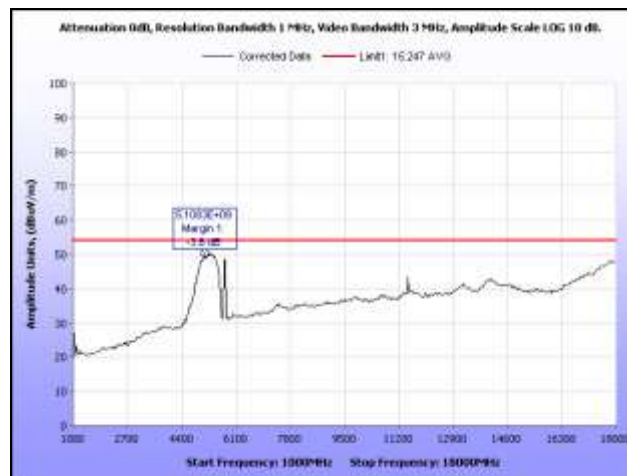
Plot 23. Radiated Spurious Emissions, 5745 MHz, 1 GHz – 18 GHz, Average, Omni Antenna
