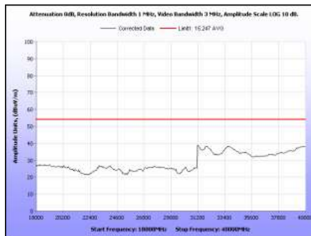
Plot 45. Radiated Spurious Emissions, 5785 MHz, 18 GHz – 40 GHz, Average, Dish Antenna
