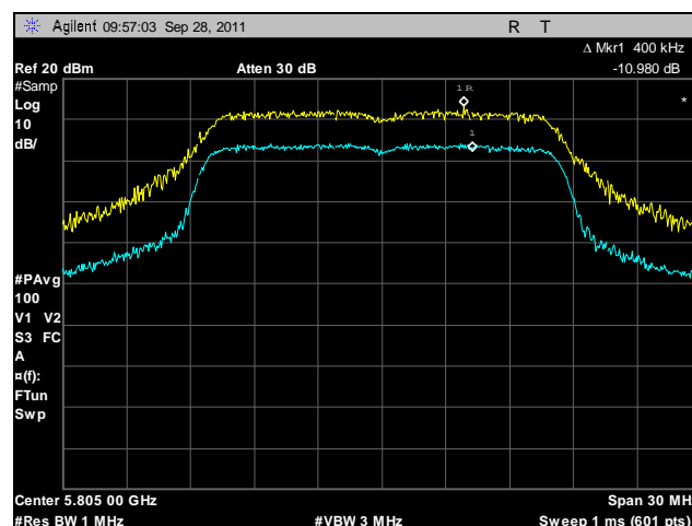
Plot 21. Peak Excursion Ratio, 5805 MHz
