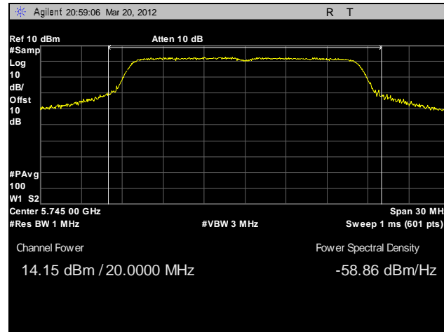
Plot 13. RF Power Output, 5745 MHz
