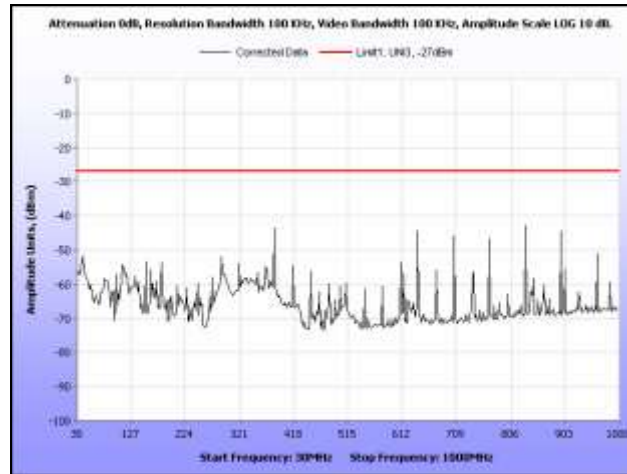
Plot 52. EIRP, 5745 MHz, 30 MHz – 1 GHz, Omni Antenna
