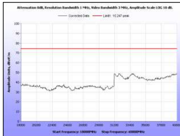
Plot 26. Radiated Spurious Emissions, 5745 MHz, 18 GHz – 40 GHz, Peak, Omni Antenna
