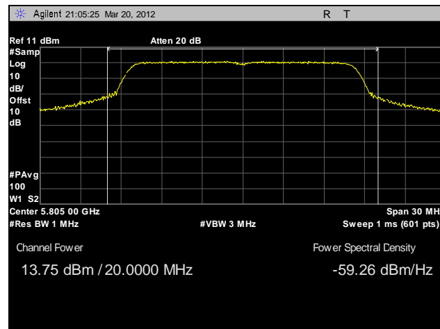
Plot 15. RF Power Output, 5805 MHz
