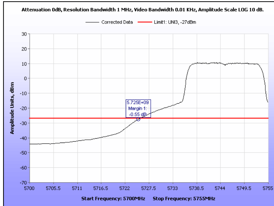
Plot 72. Radiated Band Edge, 5745 MHz, Dish Antenna
