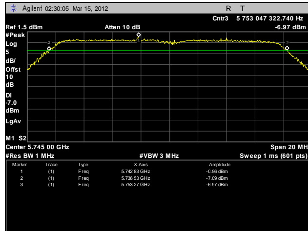
Plot 77. Frequency Stability, 5725 – 5825 MHz, 10°C, 120 V
