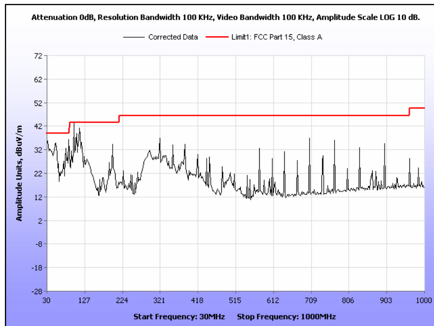
Plot 4. Radiated Emissions, 30 MHz - 1 GHz, FCC Limits, Dish Antenna
