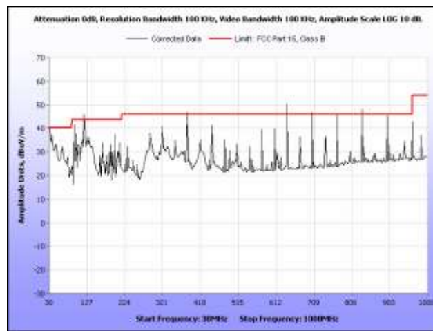
Plot 47. Radiated Spurious Emissions, 5805 MHz, 30 MHz – 1 GHz, Dish Antenna
