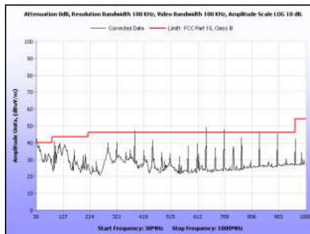
Plot 42. Radiated Spurious Emissions, 5785 MHz, 30 MHz – 1 GHz, Dish Antenna
