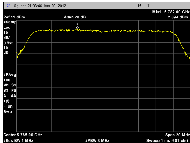
Plot 17. Power Spectral Density, 5785 MHz
