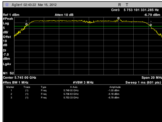
Plot 75. Frequency Stability, 5725 – 5825 MHz, -10°C, 120 V
