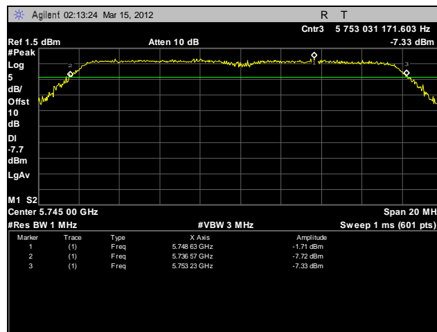
Plot 78. Frequency Stability, 5725 – 5825 MHz, 20°C, 108 V
