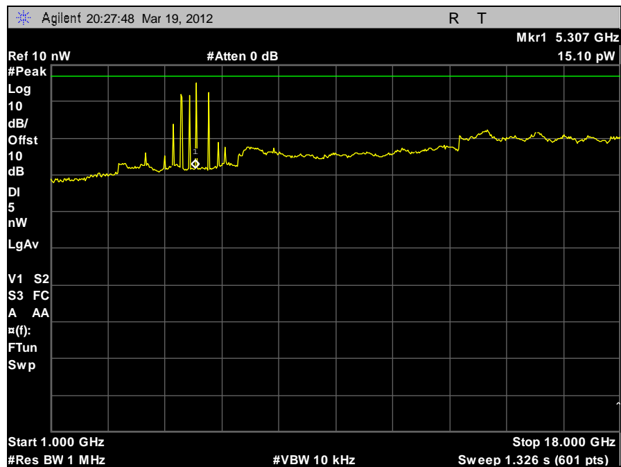
Plot 86. Receiver Spurious Emission, 1 GHz – 18 GHz
