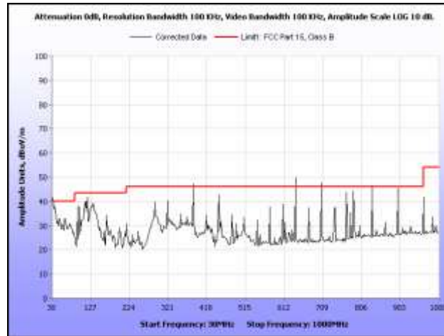
Plot 37. Radiated Spurious Emissions, 5745 MHz, 30 MHz – 1 GHz, Dish Antenna
