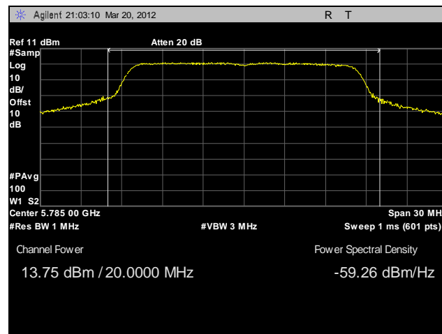
Plot 14. RF Power Output, 5785 MHz
