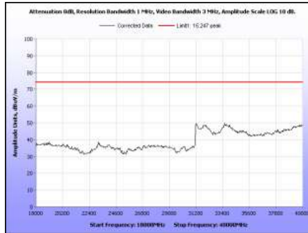
Plot 46. Radiated Spurious Emissions, 5785 MHz, 18 GHz – 40 GHz, Peak, Dish Antenna
