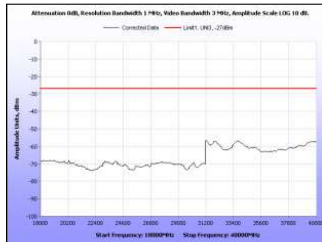
Plot 69. EIRP, 5805 MHz, 18 GHz – 40 GHz, Dish Antenna
