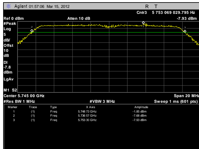
Plot 82. Frequency Stability, 5725 – 5825 MHz, 40°C, 120 V
