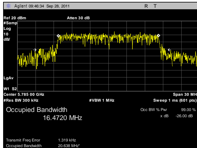
Plot 11. 99% Occupied Bandwidth, 5785 MHz
