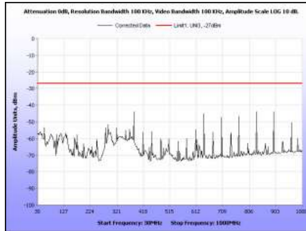
Plot 58. EIRP, 5805 MHz, 30 MHz – 1 GHz, Omni Antenna
