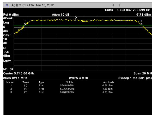
Plot 84. Frequency Stability, 5725 – 5825 MHz, 55°C, 120 V
