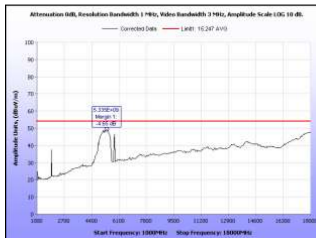
Plot 33. Radiated Spurious Emissions, 5805 MHz, 1 GHz – 18 GHz, Average, Omni Antenna
