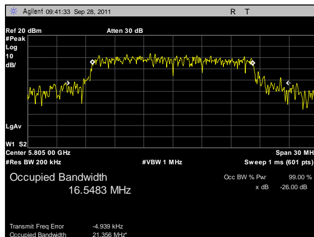
Plot 9. 26 dB Occupied Bandwidth, 5805 MHz
