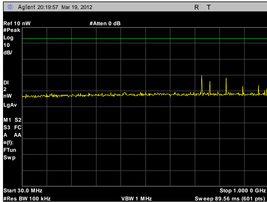
Plot 85. Receiver Spurious Emission, 30 MHz – 1 GHz
