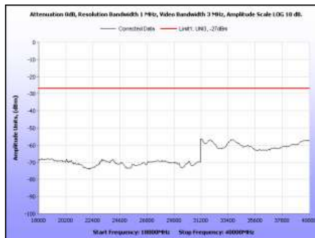
Plot 54. EIRP, 5745 MHz, 18 GHz – 40 GHz, Omni Antenna
