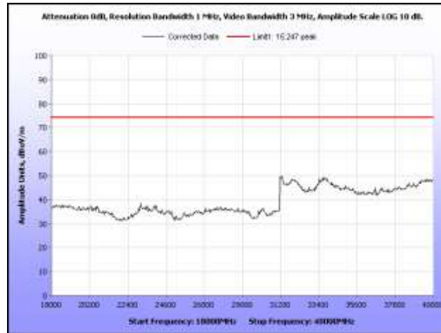
Plot 31. Radiated Spurious Emissions, 5785 MHz, 18 GHz – 40 GHz, Peak, Omni Antenna
