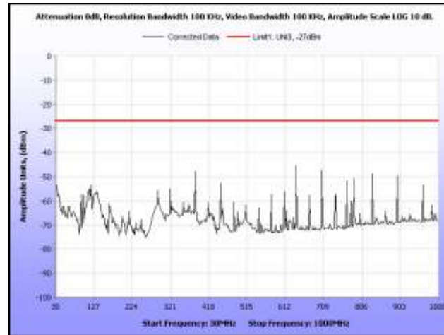
Plot 61. EIRP, 5745 MHz, 30 MHz – 1 GHz, Dish Antenna
