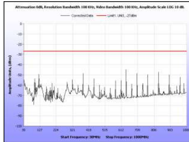
Plot 67. EIRP, 5805 MHz, 30 MHz – 1 GHz, Dish Antenna
