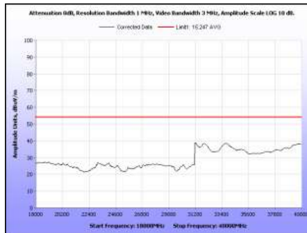
Plot 35. Radiated Spurious Emissions, 5805 MHz, 18 GHz – 40 GHz, Average, Omni Antenna
