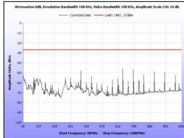
Plot 64. EIRP, 5785 MHz, 30 MHz – 1 GHz, Dish Antenna
