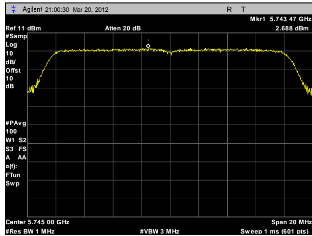
Plot 16. Power Spectral Density, 5745 MHz
