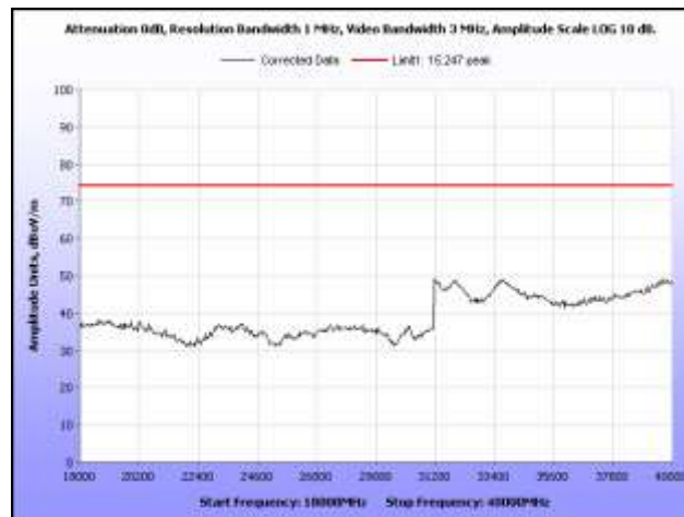
Plot 51. Radiated Spurious Emissions, 5805 MHz, 18 GHz – 40 GHz, Peak, Dish Antenna
