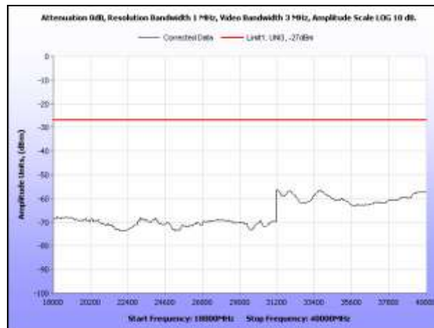
Plot 60. EIRP, 5805 MHz, 18 GHz – 40 GHz, Omni Antenna
