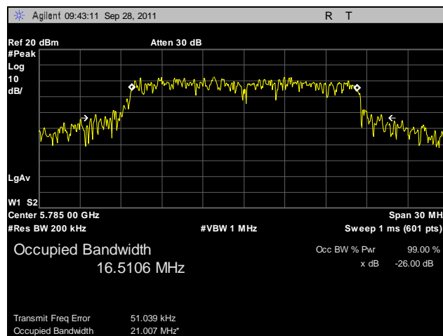
Plot 8. 26 dB Occupied Bandwidth, 5785 MHz
