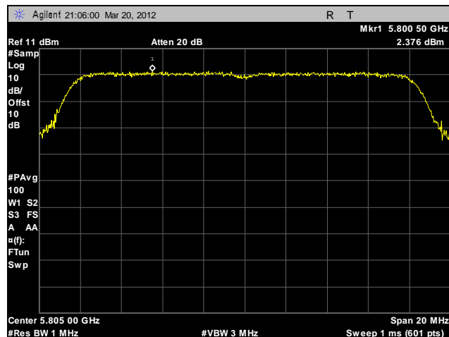
Plot 18. Power Spectral Density, 5805 MHz
