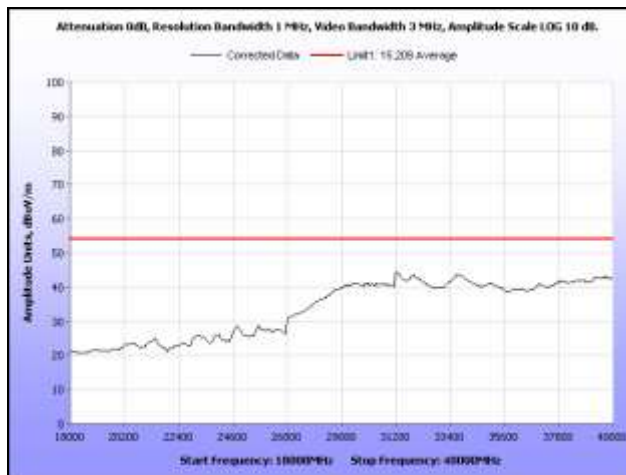
Plot 10. Radiated Spurious Emissions, Low Channel, 18 GHz – 40 GHz, Average
