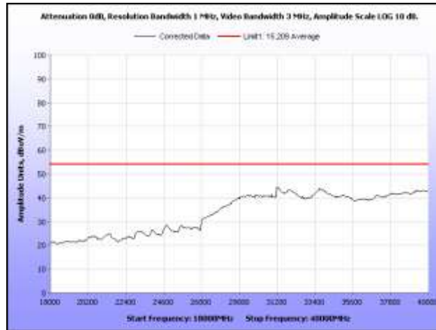
Plot 15. Radiated Spurious Emissions, Mid Channel, 18 GHz – 40 GHz, Average
