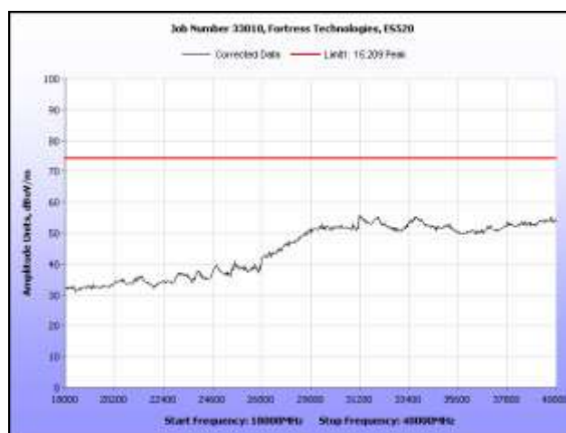
Plot 21. Radiated Spurious Emissions, High Channel, 18 GHz – 40 GHz, Peak
