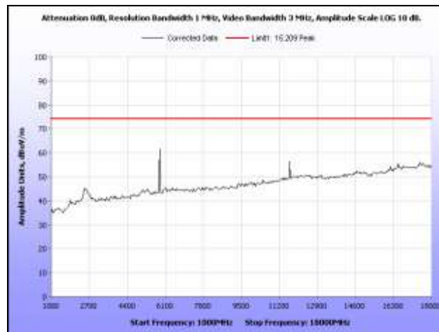
Plot 19. Radiated Spurious Emissions, High Channel, 1 GHz – 18 GHz, Peak
