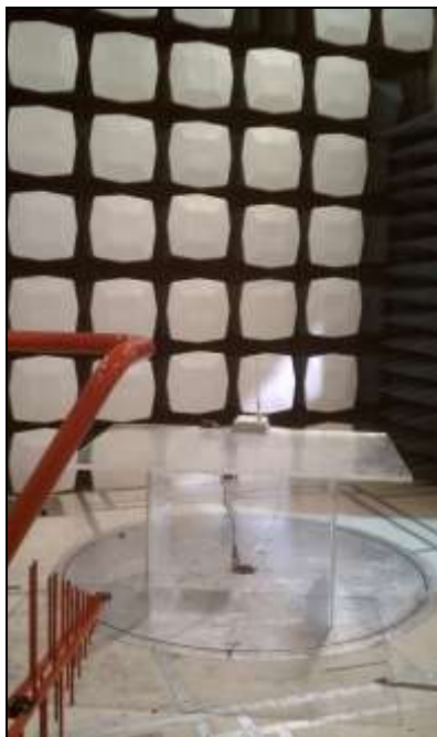
Photograph 5. Radiated Spurious Emissions, Test Setup (2)
