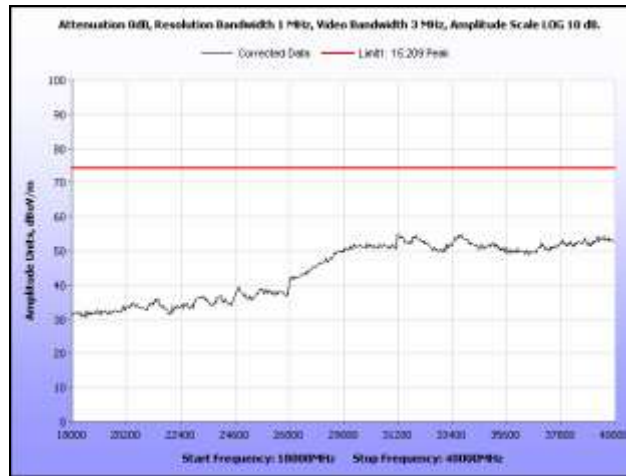
Plot 16. Radiated Spurious Emissions, Mid Channel, 18 GHz – 40 GHz, Peak
