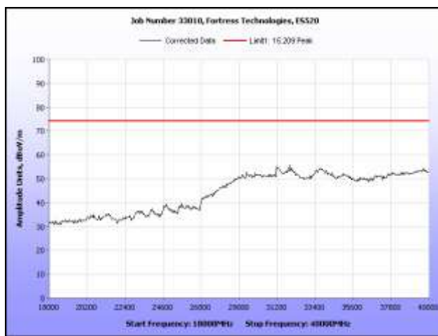
Plot 11. Radiated Spurious Emissions, Low Channel, 18 GHz – 40 GHz, Peak
