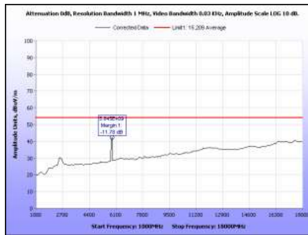
Plot 18. Radiated Spurious Emissions, High Channel, 1 GHz – 18 GHz, Average
