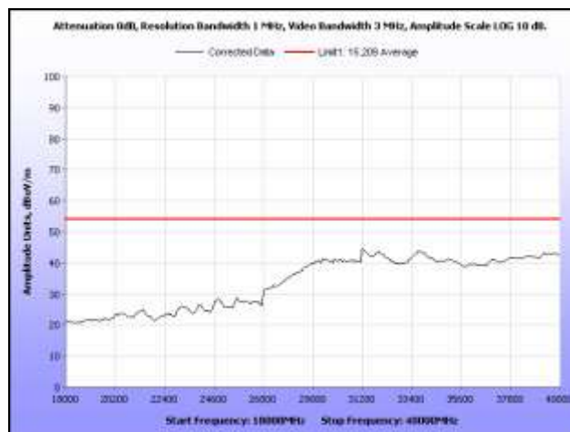
Plot 20. Radiated Spurious Emissions, High Channel, 18 GHz – 40 GHz, Average
