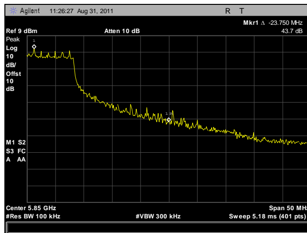
Plot 129. Conducted Band Edge, High Channel, 5.8 GHz, HT40
