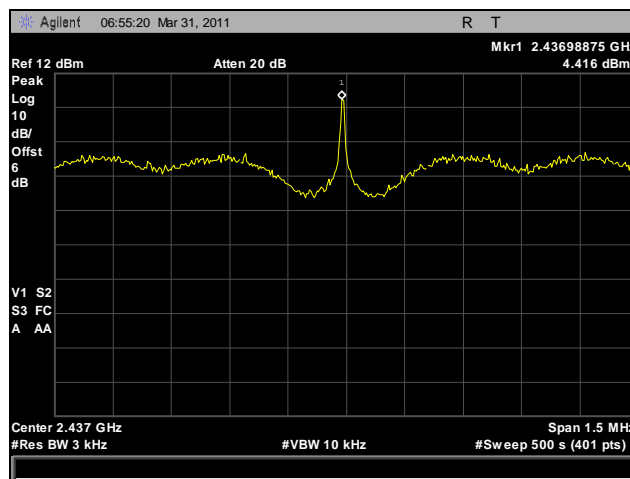
Plot 131. Peak Power Spectral Density, Mid Channel, 2.4 GHz, HT20
