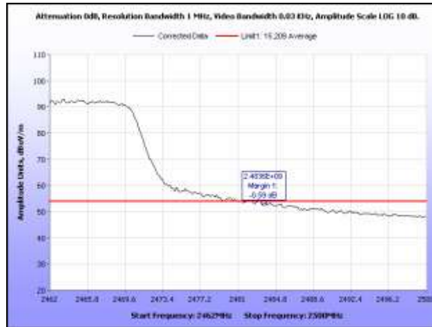
Plot 97. Radiated Restricted Band Edge, 2452 MHz, Average, HT40
