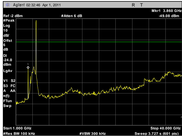
Plot 108. Conducted Spurious Emissions, Mid Channel, 1 GHz – 40 GHz, 5.8 GHz, HT20
