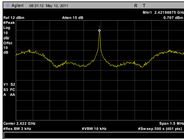
Plot 136. Peak Power Spectral Density, Low Channel, 2.4 GHz, HT40
