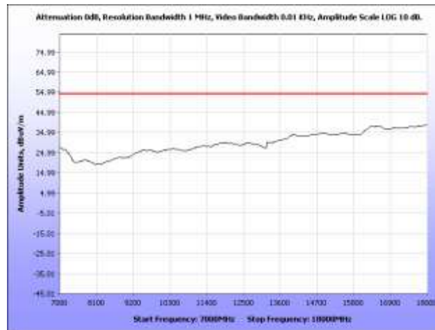
Plot 81. Radiated Spurious Emissions, High Channel, 7 GHz – 18 GHz, Average 5.8 GHz, HT40
