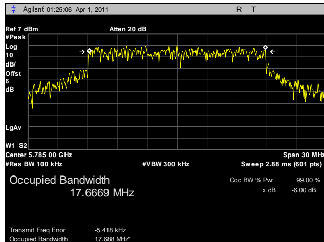
Plot 5. 6 dB Occupied Bandwidth, Mid Channel, 5.8 GHz, HT20
