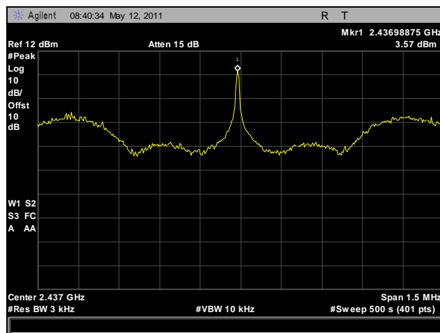
Plot 137. Peak Power Spectral Density, Mid Channel, 2.4 GHz, HT40
