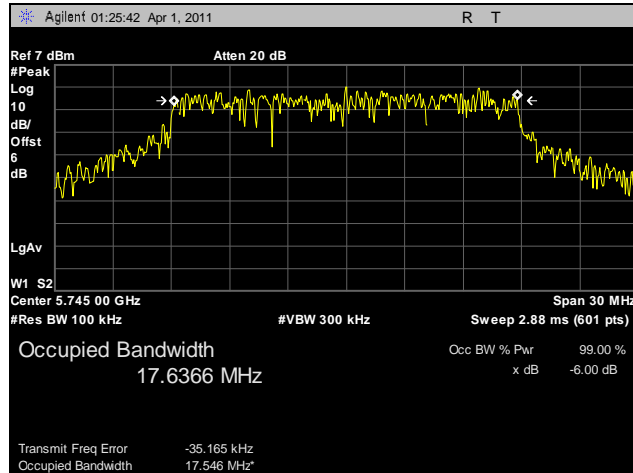
Plot 4. 6 dB Occupied Bandwidth, Low Channel, 5.8 GHz, HT20
