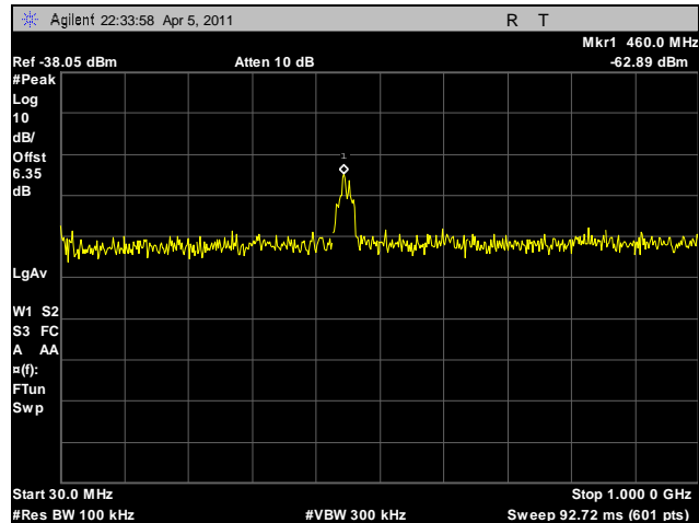
Plot 111. Conducted Spurious Emissions, Low Channel, 30 MHz – 1 GHz, 2.4 GHz, HT40
