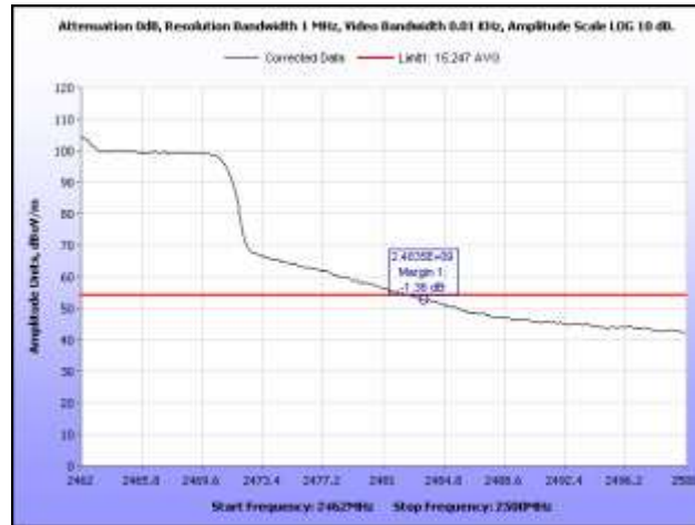
Plot 85. Radiated Restricted Band Edge, High Channel, Average, HT20
