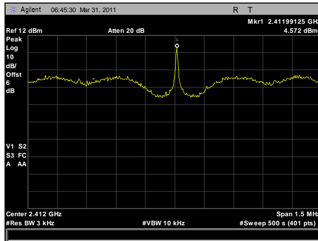
Plot 130. Peak Power Spectral Density, Low Channel, 2.4 GHz, HT20
