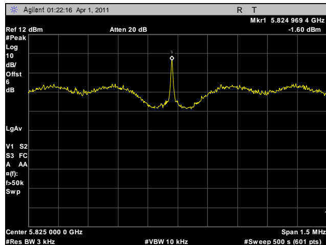
Plot 135. Peak Power Spectral Density, High Channel, 5.8 GHz, HT20
