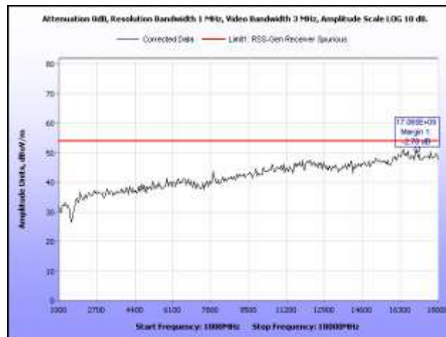
Plot 142. Receiver Spurious Emission, 1 GHz – 18 GHz, 2.4 GHz, HT20
