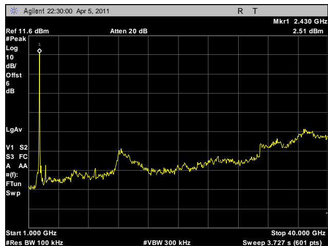
Plot 112. Conducted Spurious Emissions, Low Channel, 1 GHz – 40 GHz, 2.4 GHz, HT40
