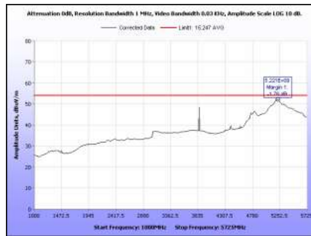
Plot 71. Radiated Spurious Emissions, Mid Channel, 1 GHz – 5.725 GHz, Average, 5.8 GHz, HT40
