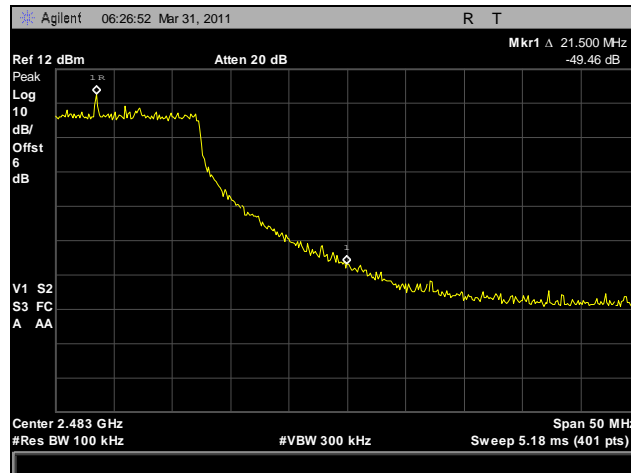
Plot 123. Conducted Band Edge, High Channel, 2.4 GHz, HT20
