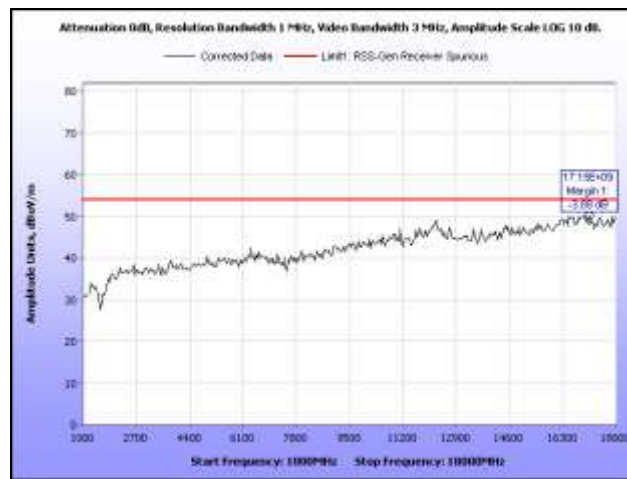
Plot 148. Receiver Spurious Emission, 1 GHz – 18 GHz, 5.8 GHz, HT40
