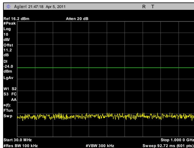
Plot 103. Conducted Spurious Emissions, High Channel, 30 MHz – 1 GHz, 2.4 GHz, HT20
