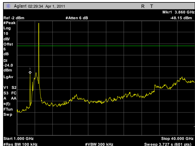
Plot 110. Conducted Spurious Emissions, High Channel, 1 GHz – 40 GHz, 5.8 GHz, HT20
