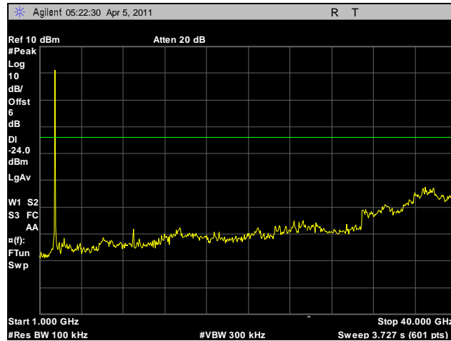
Plot 102. Conducted Spurious Emissions, Mid Channel, 1 GHz – 40 GHz, 2.4 GHz, HT20
