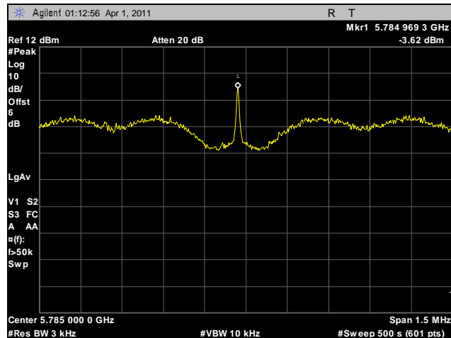
Plot 134. Peak Power Spectral Density, Mid Channel, 5.8 GHz, HT20
