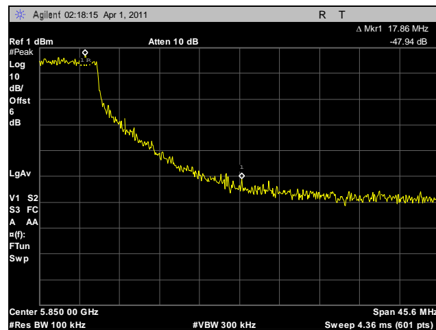
Plot 125. Conducted Band Edge, High Channel, 5.8 GHz, HT20
