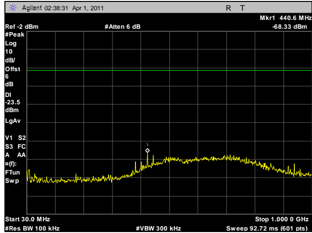
Plot 117. Conducted Spurious Emissions, Low Channel, 30 MHz – 1 GHz, 5.8 GHz, HT40
