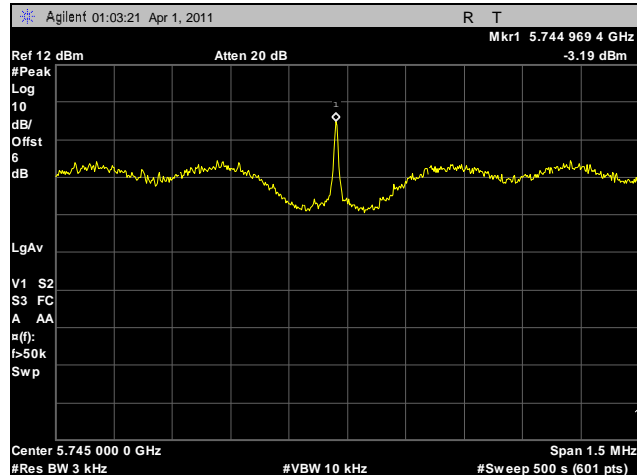
Plot 133. Peak Power Spectral Density, Low Channel, 5.8 GHz, HT20
