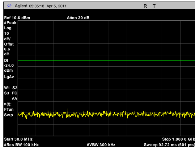
Plot 99. Conducted Spurious Emissions, Low Channel, 30 MHz – 1 GHz, 2.4 GHz, HT20
