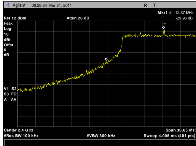
Plot 122. Conducted Band Edge, Low Channel, 2.4 GHz, HT20
