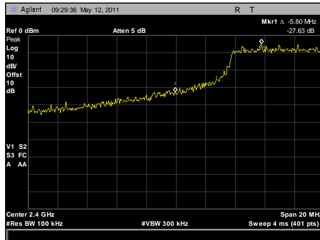
Plot 126. Conducted Band Edge, Low Channel, 2.4 GHz, HT40
