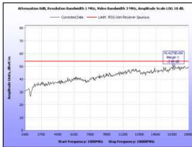
Plot 144. Receiver Spurious Emission, 1 GHz – 18 GHz, 5.8 GHz, HT20
