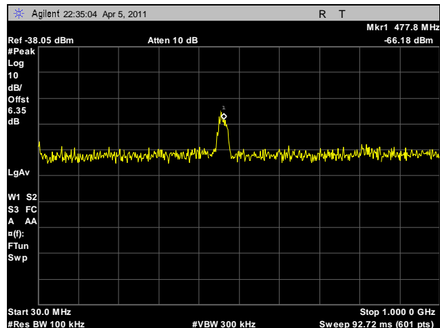
Plot 113. Conducted Spurious Emissions, Mid Channel, 30 MHz – 1 GHz, 2.4 GHz, HT40
