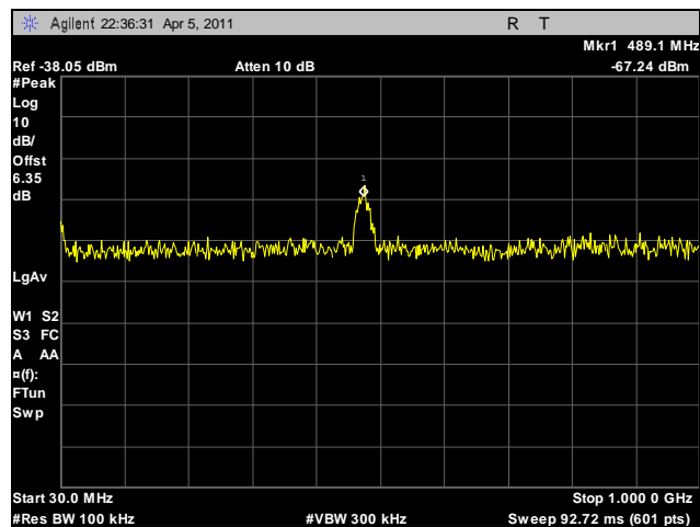
Plot 115. Conducted Spurious Emissions, High Channel, 30 MHz – 1 GHz, 2.4 GHz, HT40
