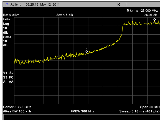
Plot 128. Conducted Band Edge, Low Channel, 5.8 GHz, HT40
