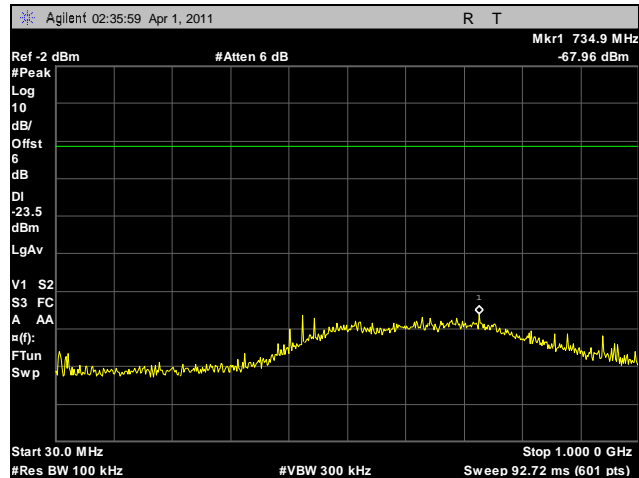
Plot 105. Conducted Spurious Emissions, Low Channel, 30 MHz – 1 GHz, 5.8 GHz, HT20
