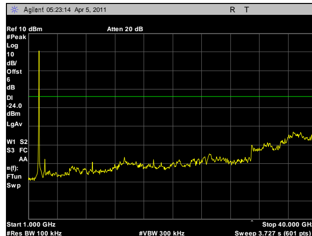
Plot 100. Conducted Spurious Emissions, Low Channel, 1 GHz – 40 GHz, 2.4 GHz, HT20
