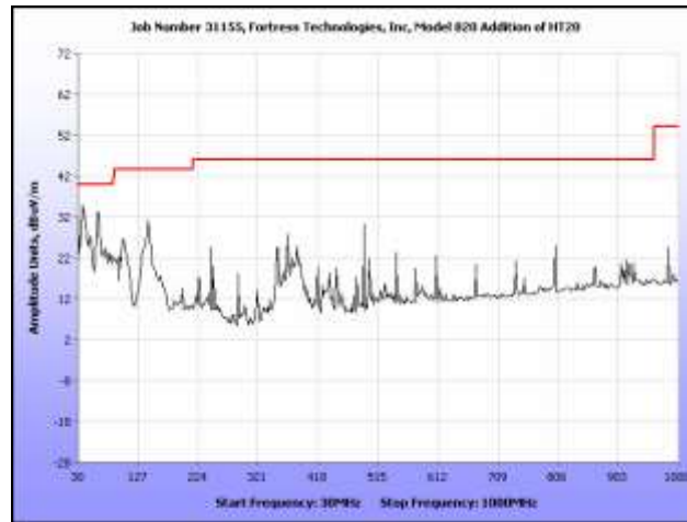
Plot 141. Receiver Spurious Emission, 30 MHz – 1 GHz, 2.4 GHz, HT20
