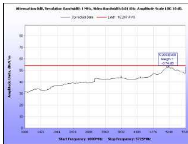
Plot 41. Radiated Spurious Emissions, Low Channel, 1 GHz – 5.725 GHz, Average, 5.8 GHz, HT20
