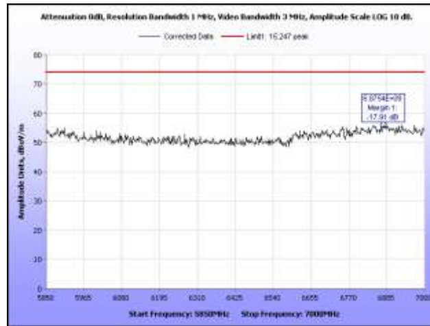
Plot 44. Radiated Spurious Emissions, Low Channel, 5.850 GHz – 7 GHz, Peak, 5.8 GHz, HT20
