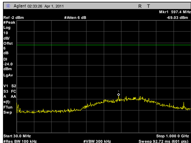
Plot 107. Conducted Spurious Emissions, Mid Channel, 30 MHz – 1 GHz, 5.8 GHz, HT20
