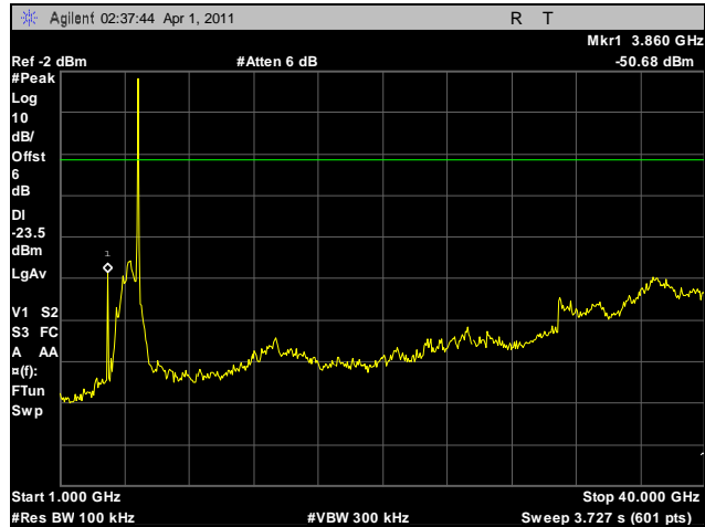
Plot 118. Conducted Spurious Emissions, Low Channel, 1 GHz – 40 GHz, 5.8 GHz, HT40
