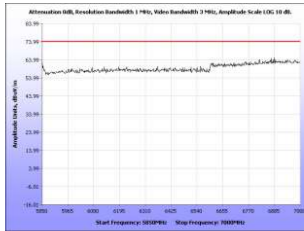
Plot 80. Radiated Spurious Emissions, High Channel, 5.850 GHz – 7 GHz, Peak, 5.8 GHz, HT40
