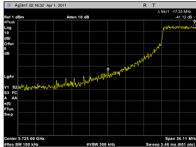
Plot 124. Conducted Band Edge, Low Channel, 5.8 GHz, HT20
