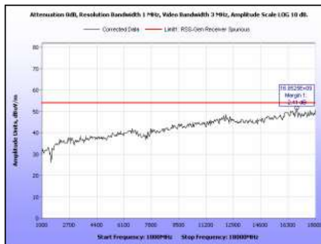
Plot 146. Receiver Spurious Emission, 1 GHz – 18 GHz, 2.4 GHz, HT40
