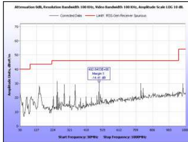
Plot 147. Receiver Spurious Emission, 30 MHz – 1 GHz, 5.8 GHz, HT40
