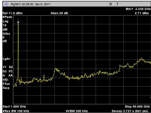
Plot 114. Conducted Spurious Emissions, Mid Channel, 1 GHz – 40 GHz, 2.4 GHz, HT40
