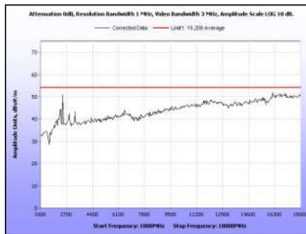
Plot 59. Radiated Spurious Emissions, Low Channel, 1 GHz – 18 GHz, 2.4 GHz, HT40
