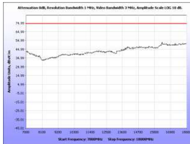
Plot 82. Radiated Spurious Emissions, High Channel, 7 GHz – 18 GHz, Peak 5.8 GHz, HT40
