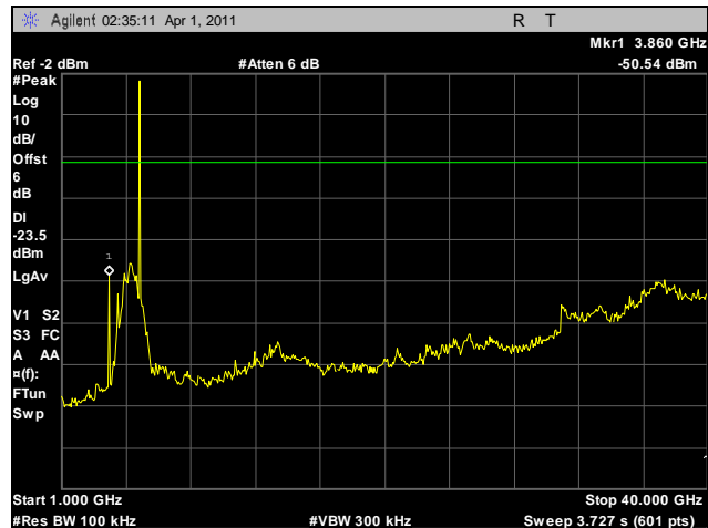
Plot 106. Conducted Spurious Emissions, Low Channel, 1 GHz – 40 GHz, 5.8 GHz, HT20
