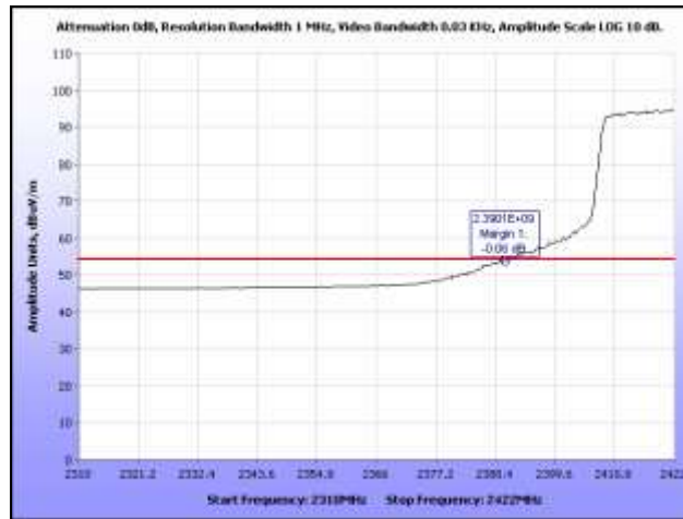
Plot 89. Radiated Restricted Band Edge, 2427 MHz, Average, HT40
