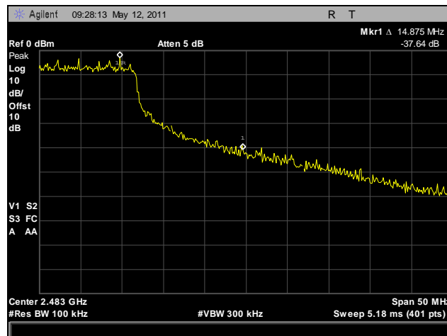
Plot 127. Conducted Band Edge, High Channel, 2.4 GHz, HT40
