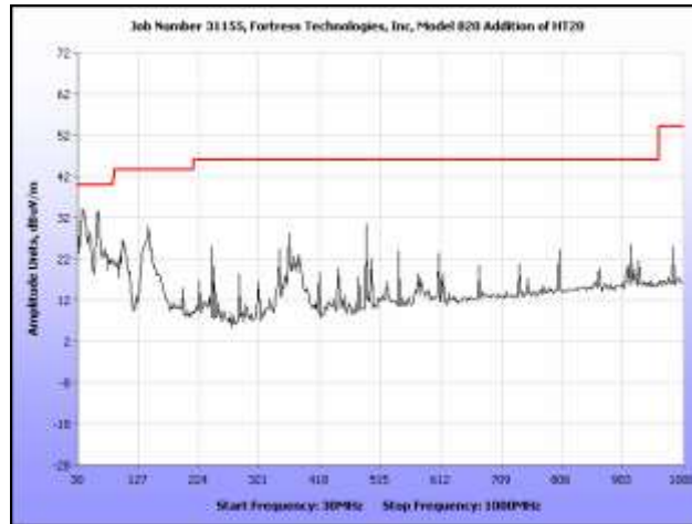
Plot 143. Receiver Spurious Emission, 30 MHz – 1 GHz, 5.8 GHz, HT20
