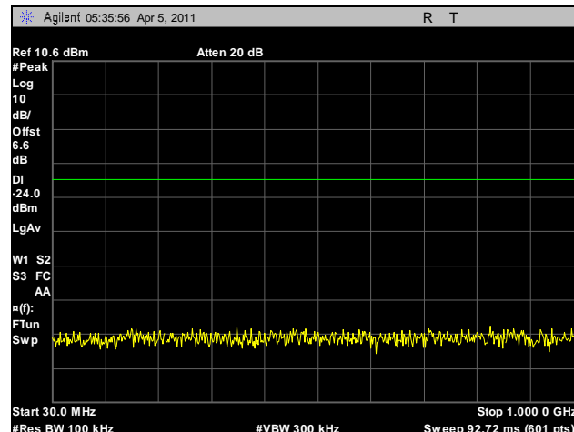
Plot 101. Conducted Spurious Emissions, Mid Channel, 30 MHz – 1 GHz, 2.4 GHz, HT20
