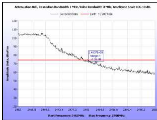
Plot 98. Radiated Restricted Band Edge, 2452 MHz, Peak, HT40
