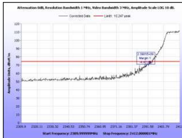
Plot 84. Radiated Restricted Band Edge, Low Channel, Peak, HT20
