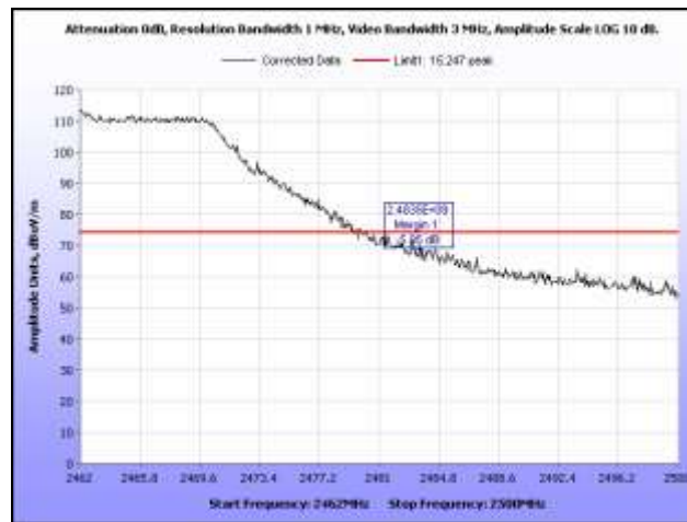
Plot 86. Radiated Restricted Band Edge, High Channel, Peak, HT20
