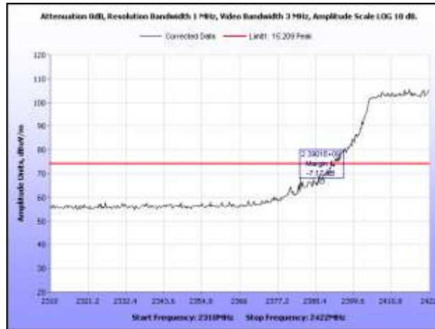
Plot 88. Radiated Restricted Band Edge, 2422 MHz, Peak, HT40
