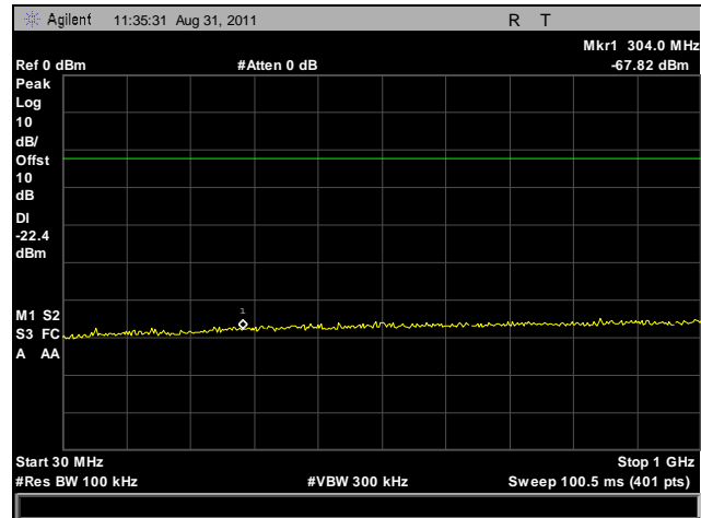
Plot 119. Conducted Spurious Emissions, High Channel, 30 MHz – 1 GHz, 5.8 GHz, HT40
