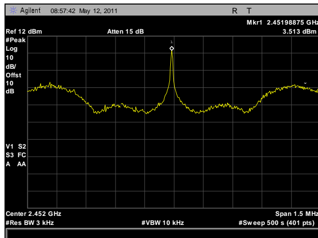
Plot 138. Peak Power Spectral Density, High Channel, 2.4 GHz, HT40
