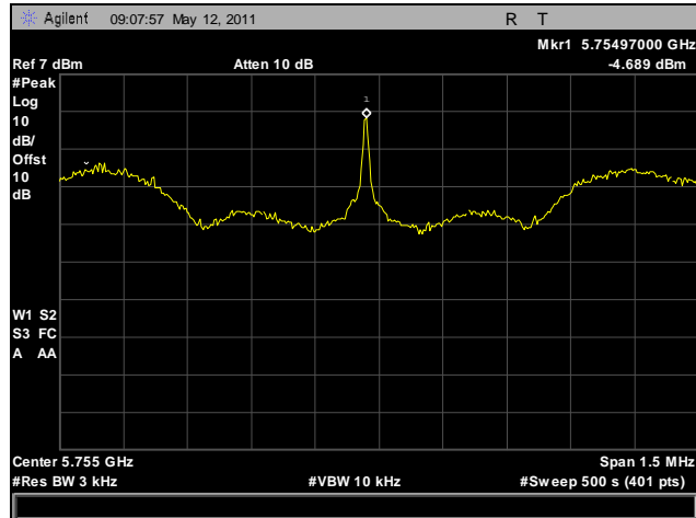
Plot 139. Peak Power Spectral Density, Low Channel, 5.8 GHz, HT40
