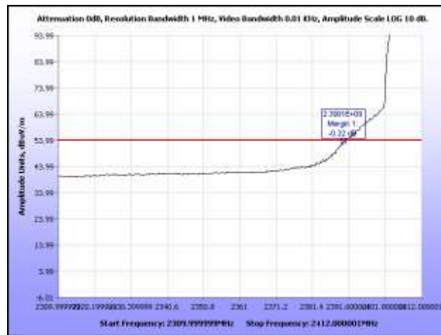
Plot 83. Radiated Restricted Band Edge, Low Channel, Average, HT20
