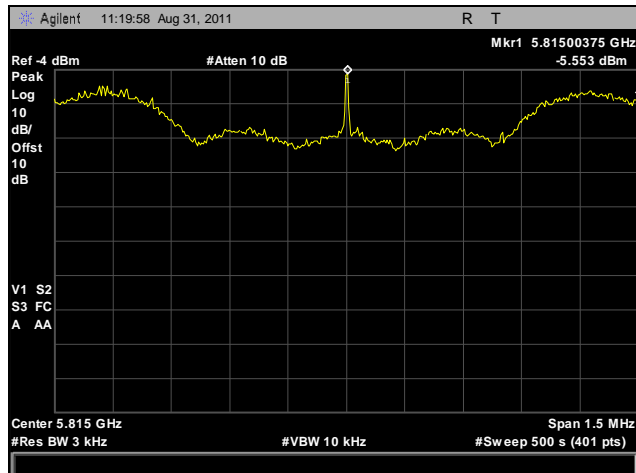
Plot 140. Peak Power Spectral Density, High Channel, 5.8 GHz, HT40
