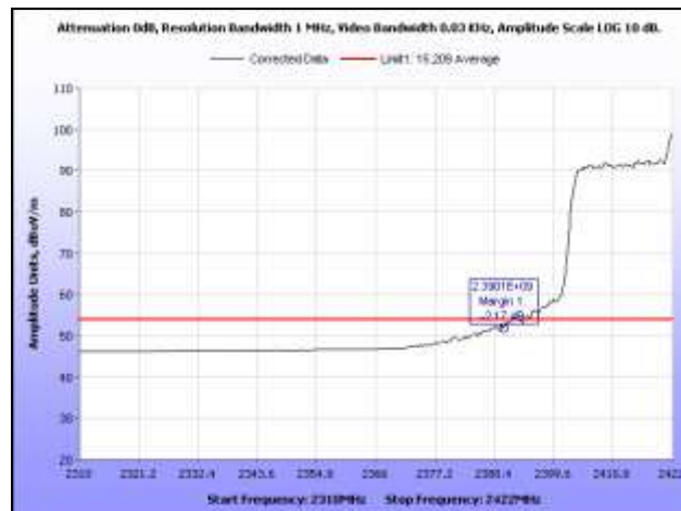
Plot 87. Radiated Restricted Band Edge, 2422 MHz, Average, HT40
