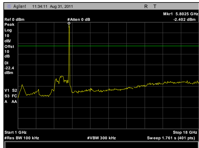
Plot 120. Conducted Spurious Emissions, High Channel, 1 GHz – 18 GHz, 5.8 GHz, HT40
