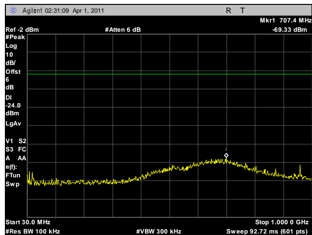
Plot 109. Conducted Spurious Emissions, High Channel, 30 MHz – 1 GHz, 5.8 GHz, HT20
