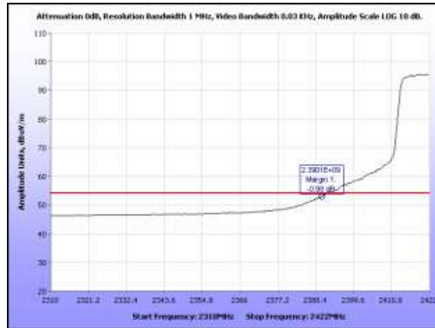
Plot 91. Radiated Restricted Band Edge, 2432 MHz, Average, HT40
