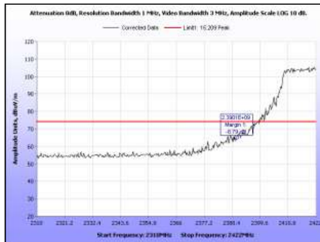
Plot 90. Radiated Restricted Band Edge, 2427 MHz, Peak, HT40
