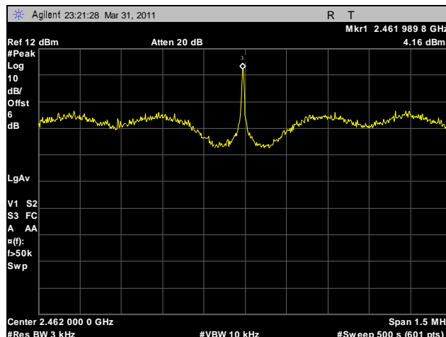
Plot 132. Peak Power Spectral Density, High Channel, 2.4 GHz, HT20
